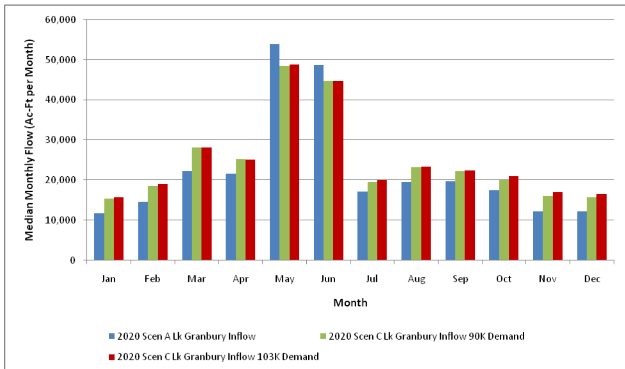
Figure 12 Monthly Median Simulated Inflow to Lake Granbury Scenarios A and C – 2020 Conditions
