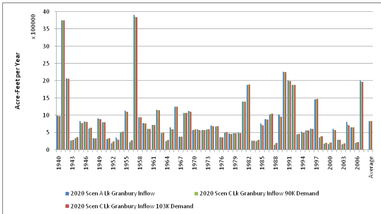
Figure 10 Simulated Annual Inflow to Lake Granbury Scenarios A and C – 2020 Conditions
