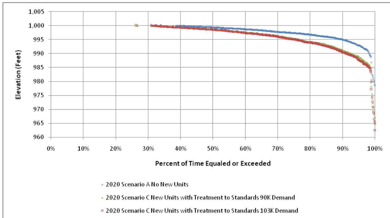
Figure 6 Exceedence Frequencies of Simulated Lake Possum Kingdom Elevations Scenarios A and C – 2020 Conditions
