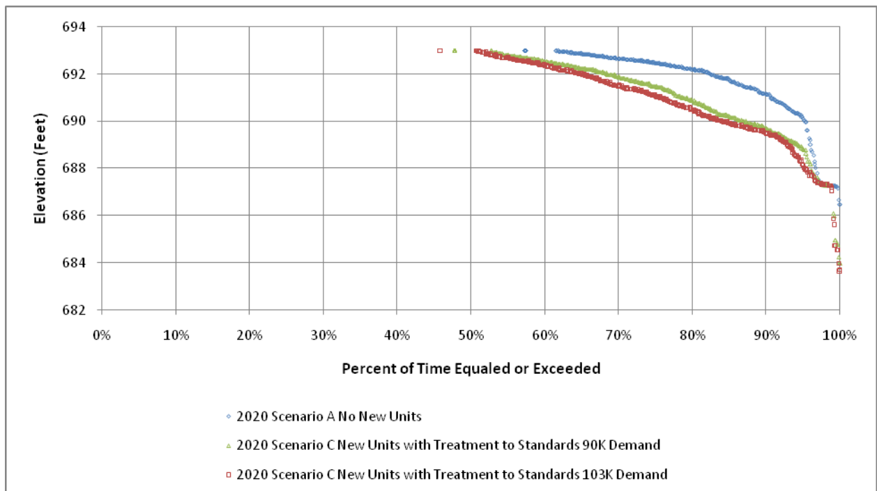
Figure 4 Exceedence Frequencies of Simulated Lake Granbury Elevations Scenarios A and C – 2020 Conditions
