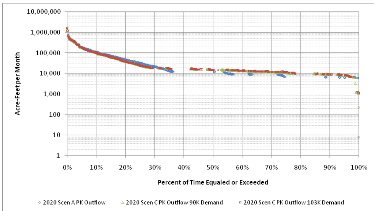
Figure 8 Exceedence Frequencies of Monthly Simulated Outflow from Lake Possum Kingdom Scenarios A and C – 2020 Conditions
