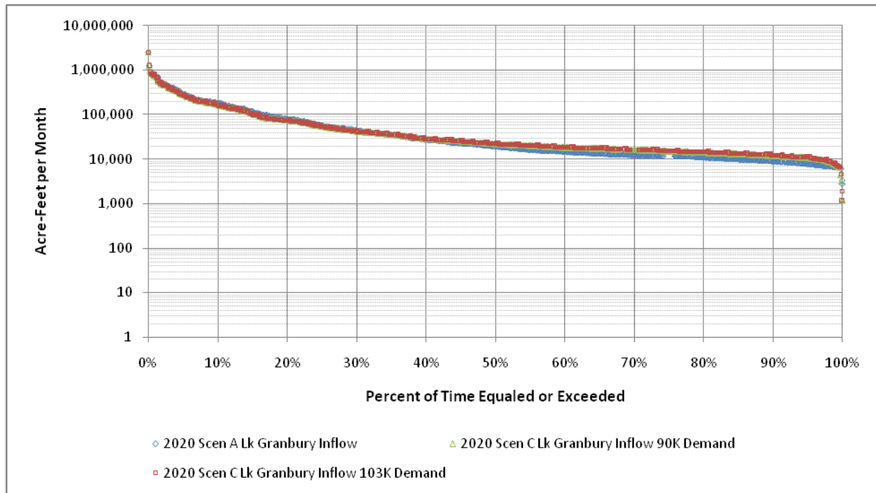
Figure 12 Monthly Median Simulated Inflow to Lake Granbury Scenarios A and C – 2020 Conditions
