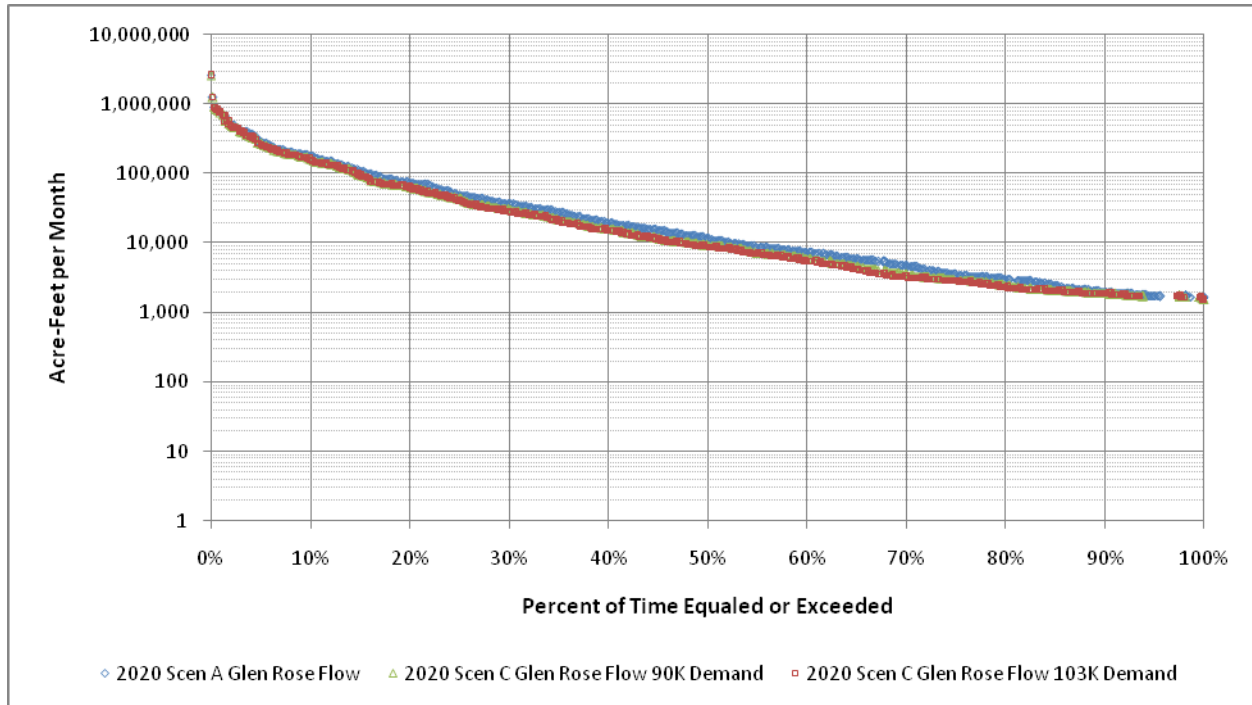
Figure 18 Monthly Median Simulated Flow at Brazos River near Glen Rose Gage Scenarios A and C – 2020 Conditions
