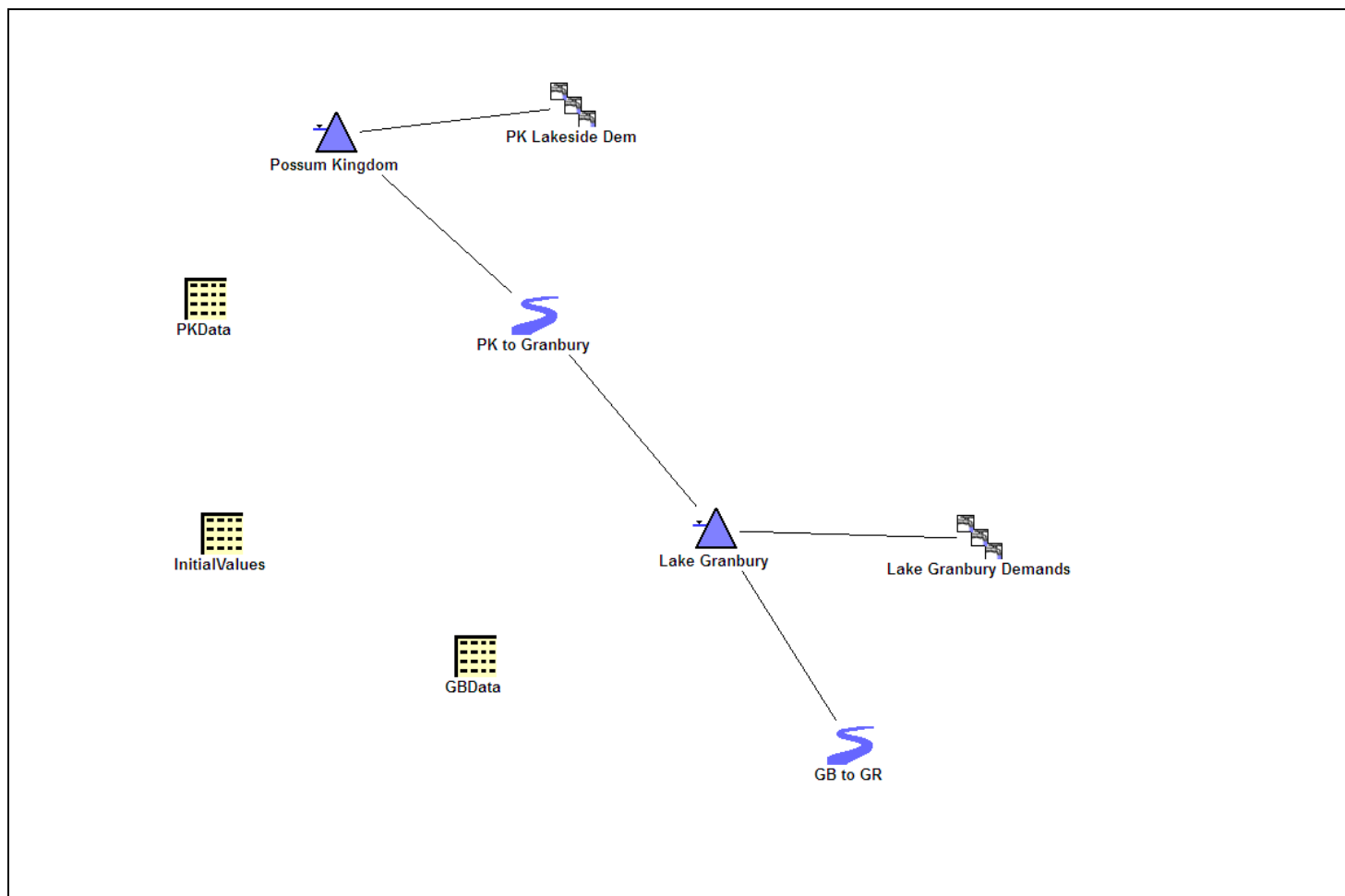
Figure 2 Objects in RiverWare Model
