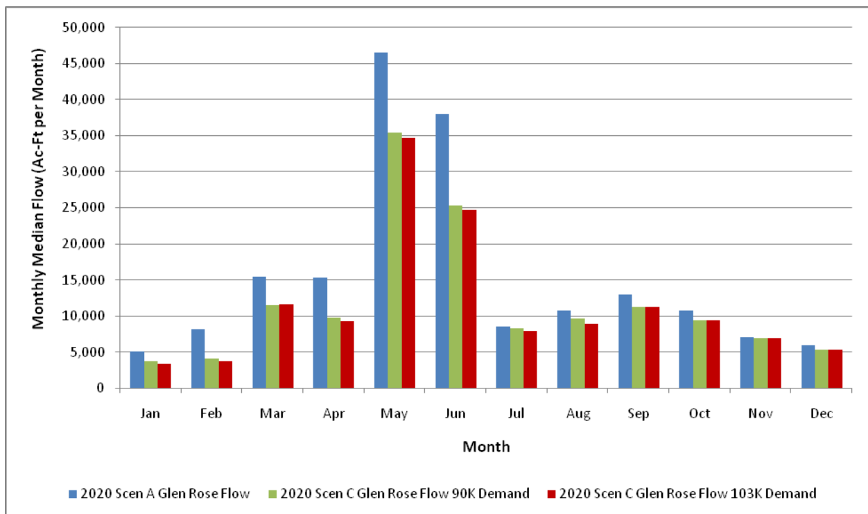
Figure 18 Monthly Median Simulated Flow at Brazos River near Glen Rose Gage Scenarios A and C – 2020 Conditions
