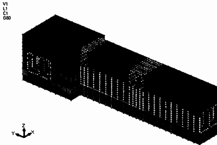
Tunnel Segment 3 including surrounding soil layers and fill beneath
