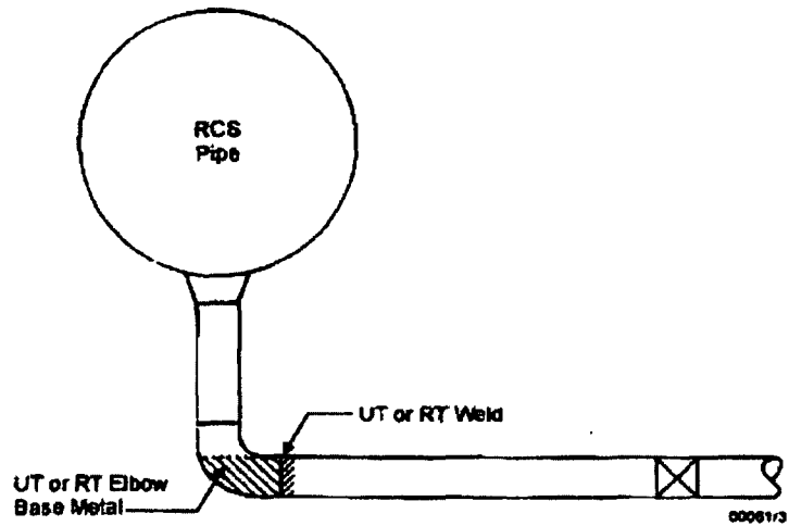
Figure 2-15 Examination Zones for Butt-Welded Bottom Connected Lines
