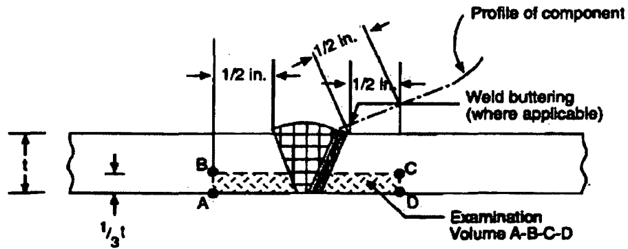
Figure 2-17 Examination Volume for Thermal Fatigue Cracking in Piping Welds Less than NPS 4 [14]
