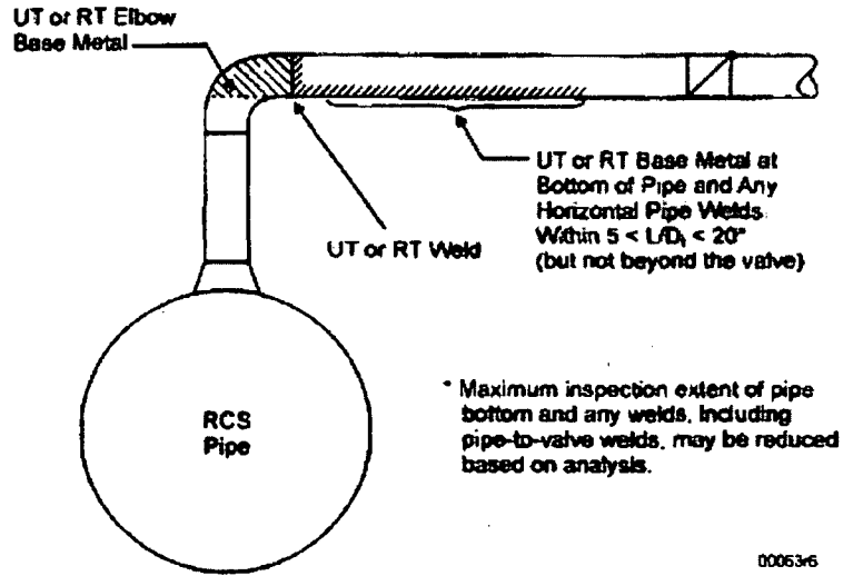
Figure 2-12 Examination Zones for Butt-Welded Lines Vertically Upward from RCS Piping
