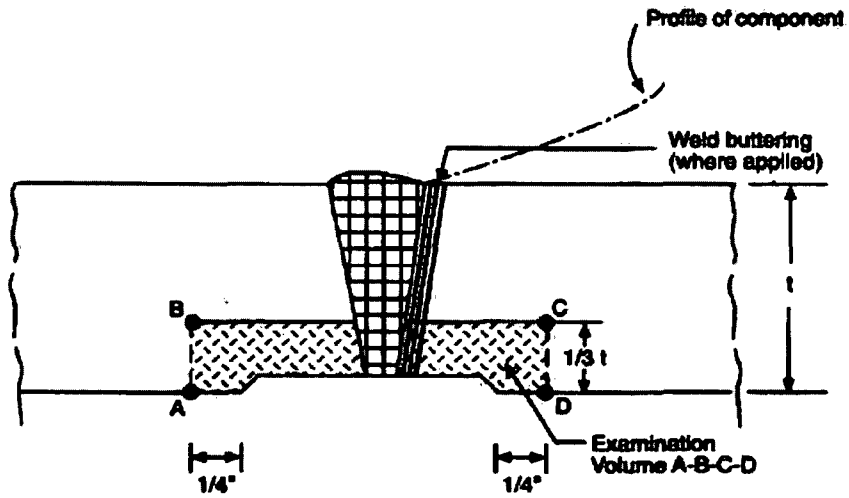
Figure 2-18 Examination Volume for Thermal Fatigue Cracking in Piping Welds NPS 4 or Larger [14]
