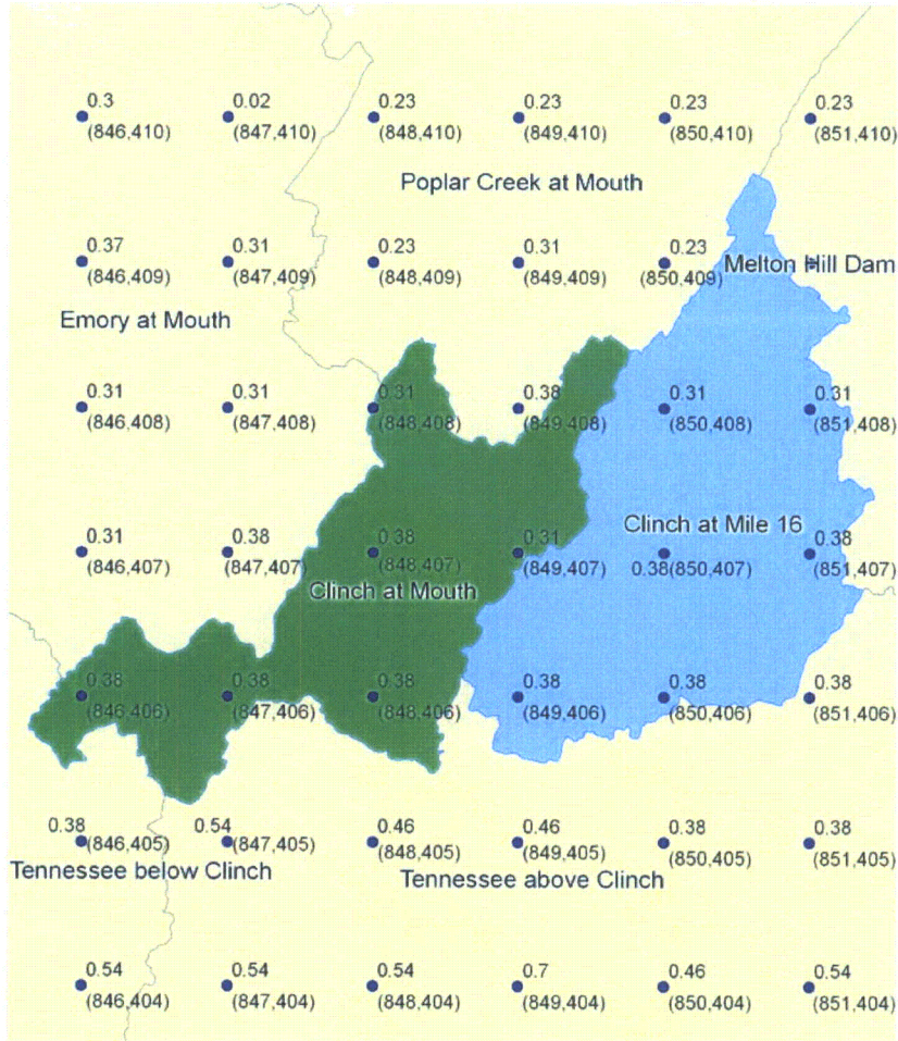
Figure 2: Hourly Precipitation Ending at 9/16/2004 18:00 for "Clinch at Mouth" and "Clinch at Mile 16" Subbasins
