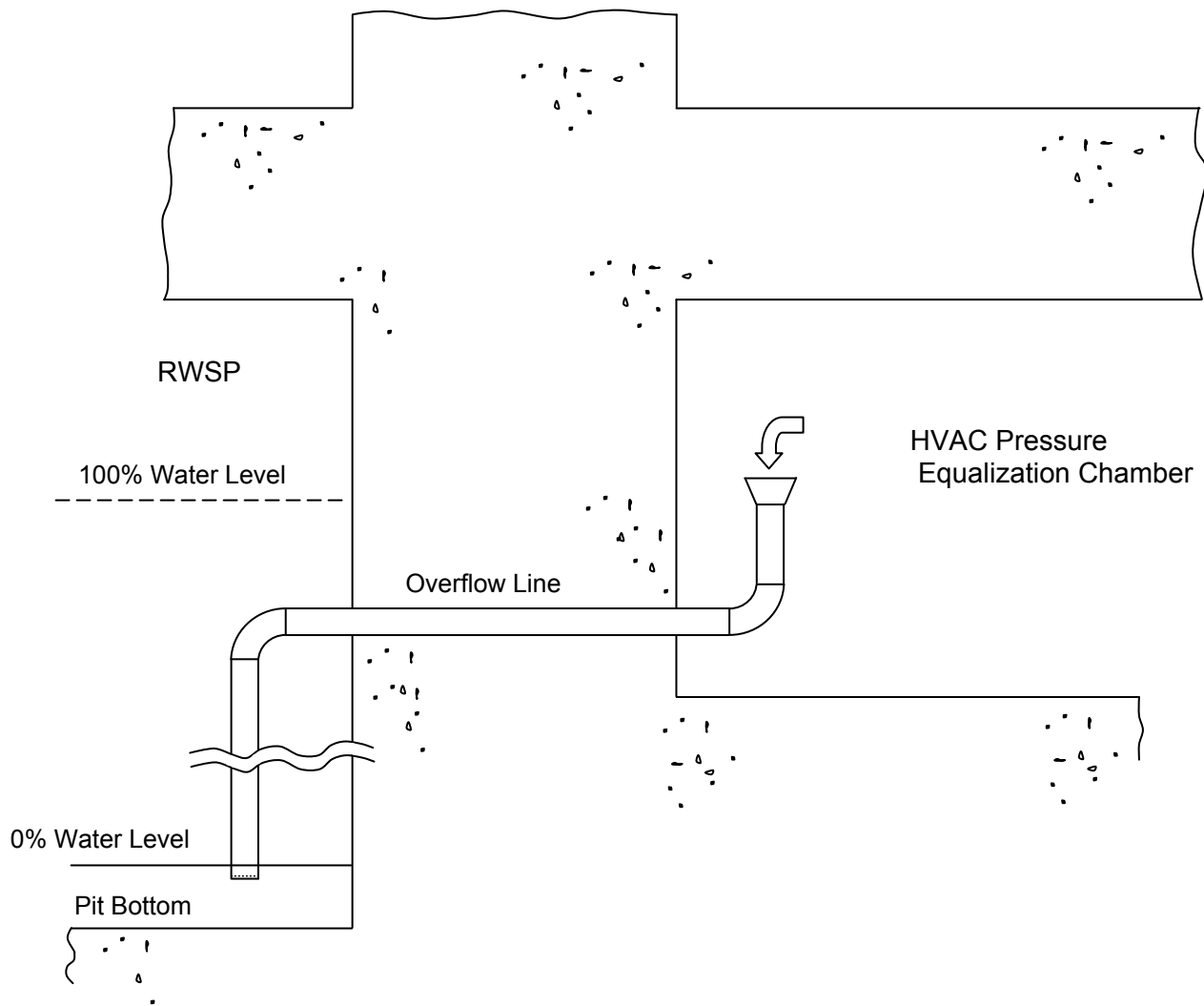
Figure 6.2.1-14 Communicating Piping of HVAC Pressure Equalization Chamber
