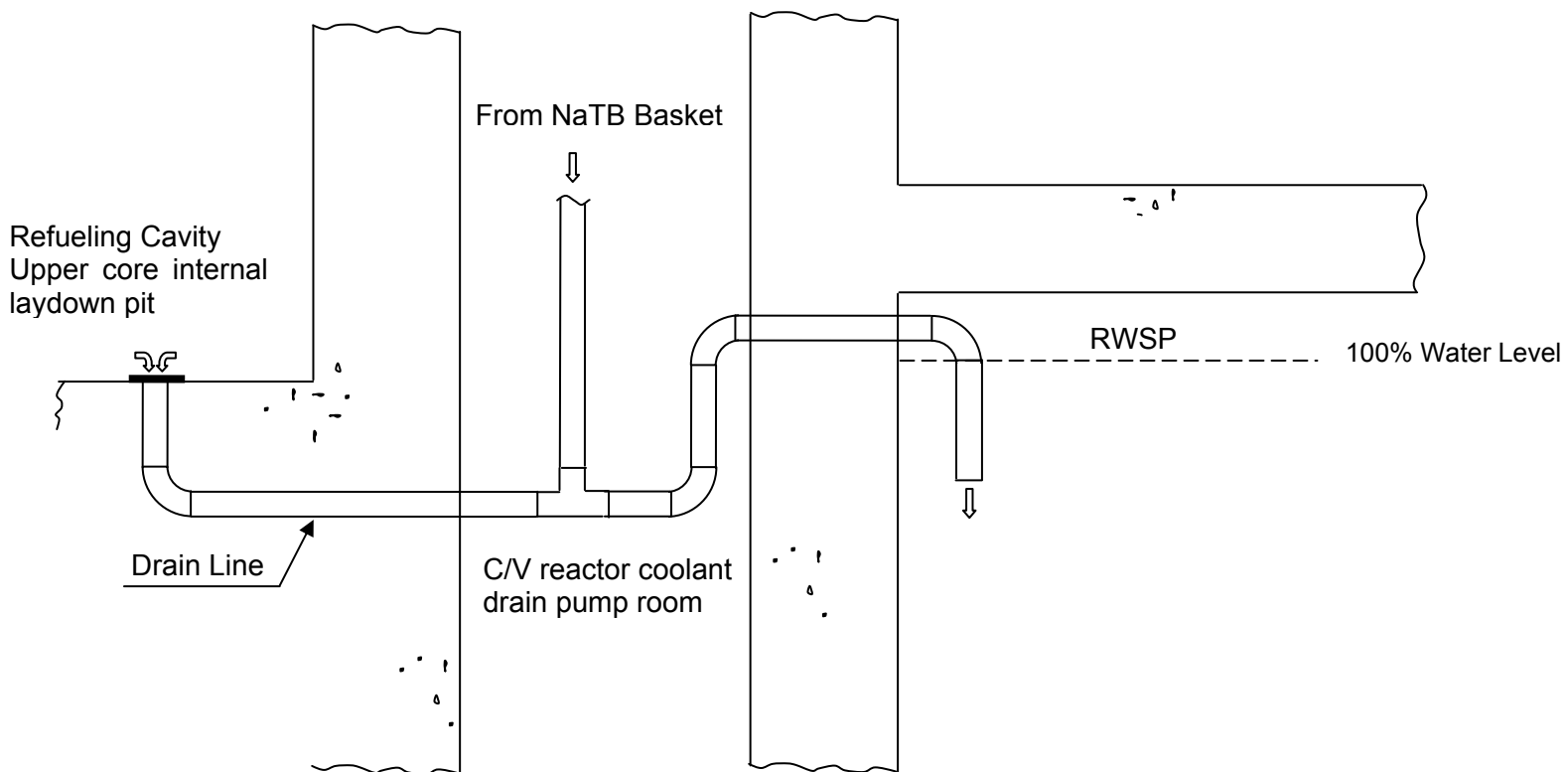
Figure 6.2.1-13 Refueling Cavity Drain Line
