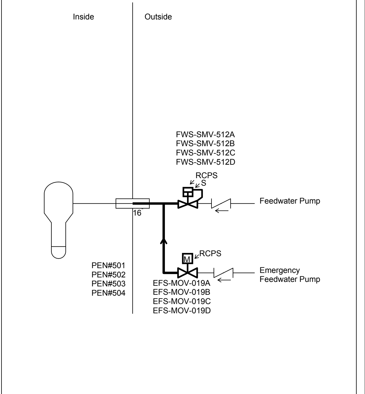
Figure 6.2.4-1 Containment Isolation Configurations (Sheet 14 of 51)
