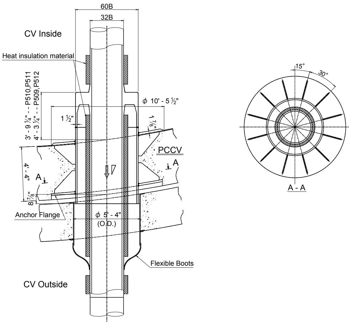
Figure 6.2.1-6 Main Steam Line Penetrations
