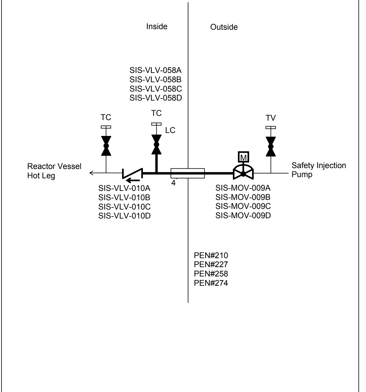
Figure 6.2.4-1 Containment Isolation Configurations (Sheet 10 of 51)
