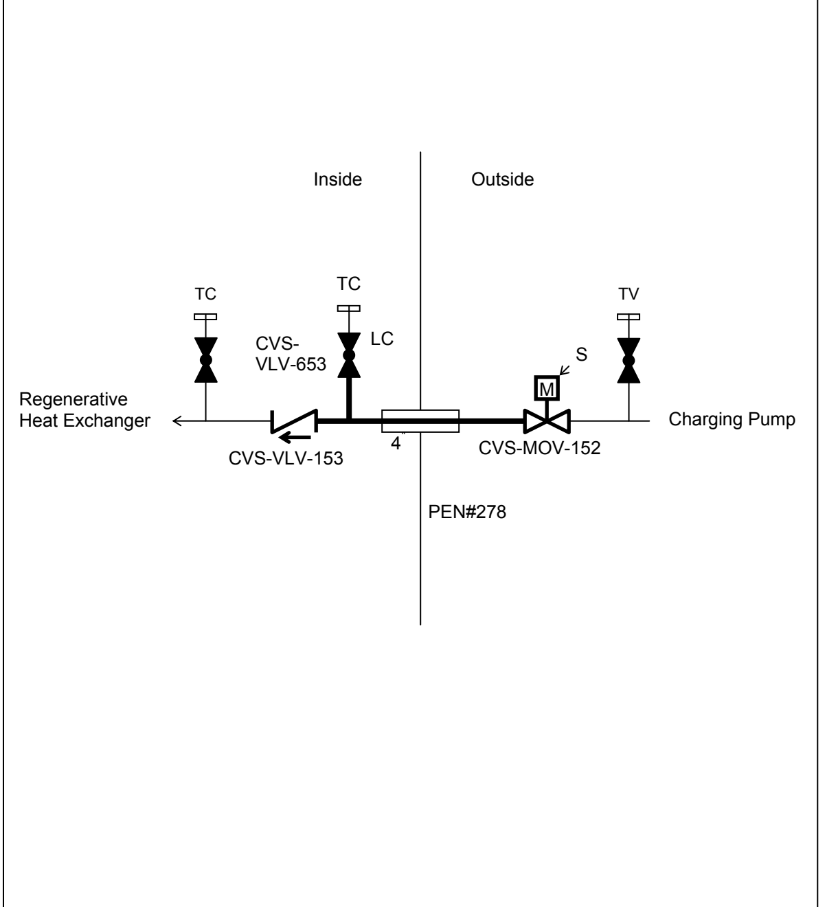
Figure 6.2.4-1 Containment Isolation Configurations (Sheet 6 of 51)
