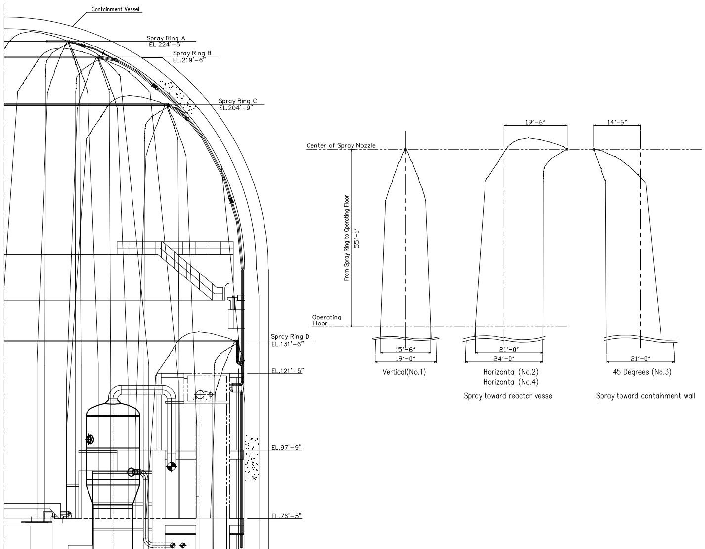
Figure 6.2.2-5 Containment Spray System Spray Ring Elevations
