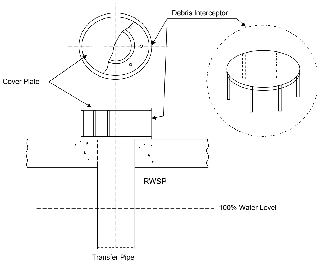
Figure 6.2.1-12 Transfer Piping
