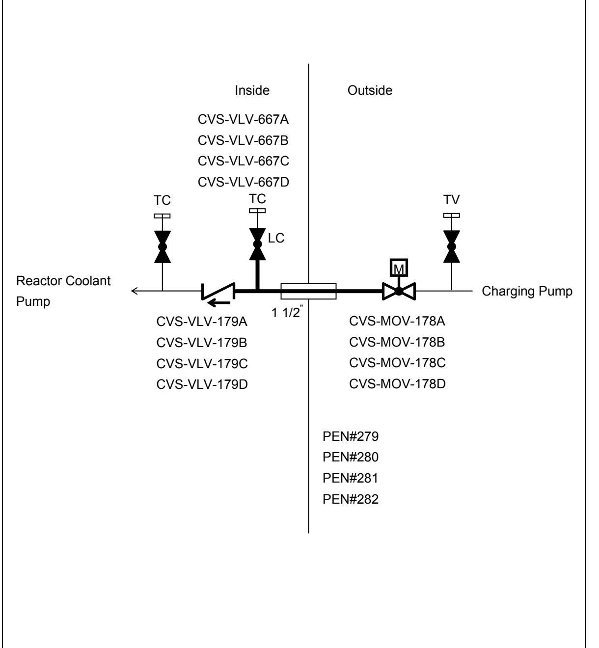
Figure 6.2.4-1 Containment Isolation Configurations (Sheet 7 of 51)
