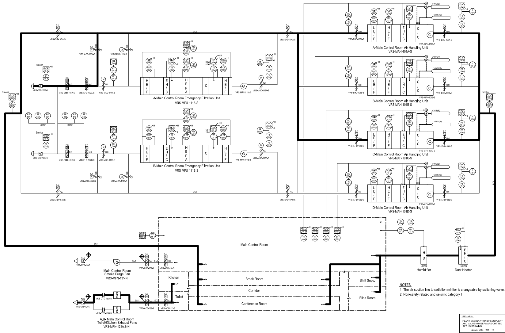
Figure 6.4-2 MCR HVAC System (Normal Operation Mode)
