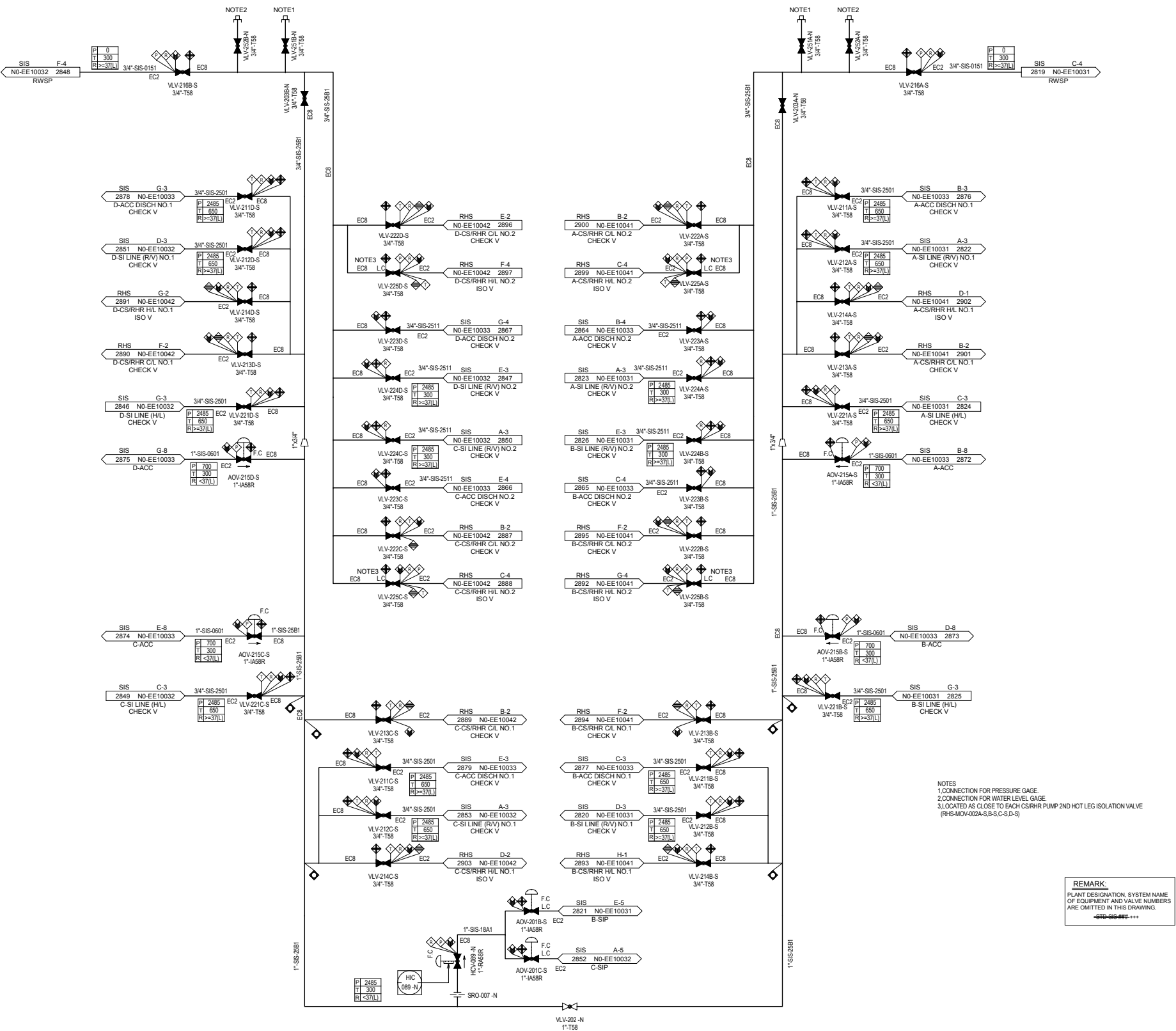
Figure 6.3-2 ECCS Piping and Instrumentation Diagram (Sheet 4 of 4)
