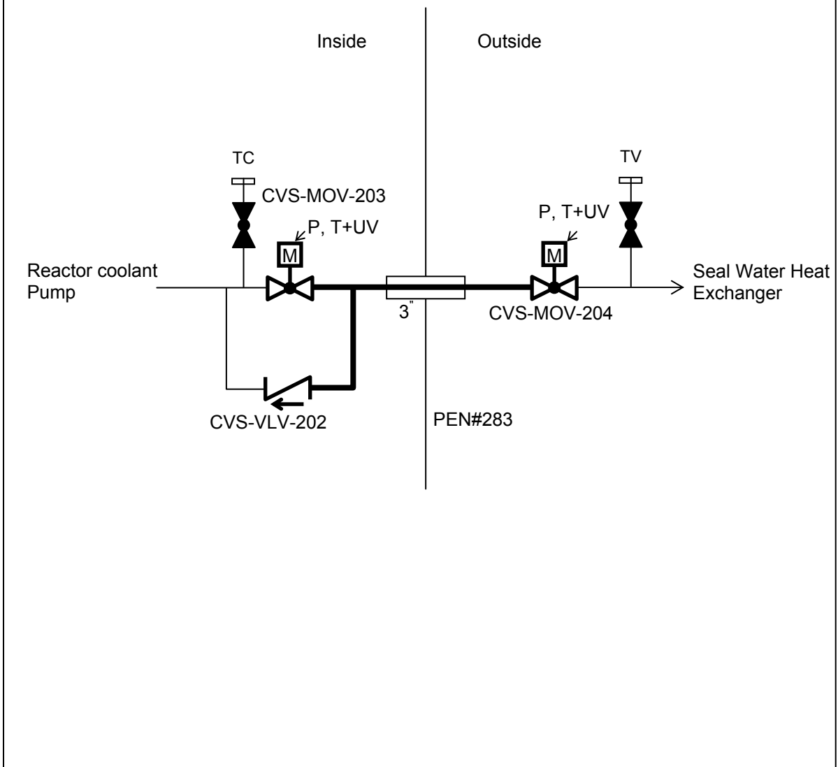
Figure 6.2.4-1 Containment Isolation Configurations (Sheet 8 of 51)
