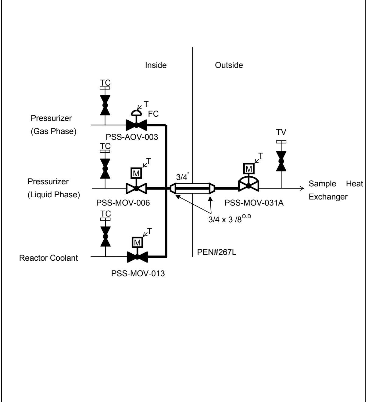
Figure 6.2.4-1 Containment Isolation Configurations (Sheet 27 of 51)
