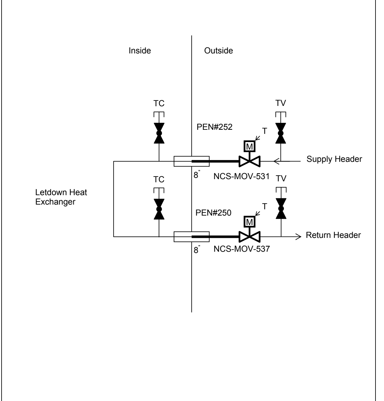
Figure 6.2.4-1 Containment Isolation Configurations (Sheet 22 of 51)
