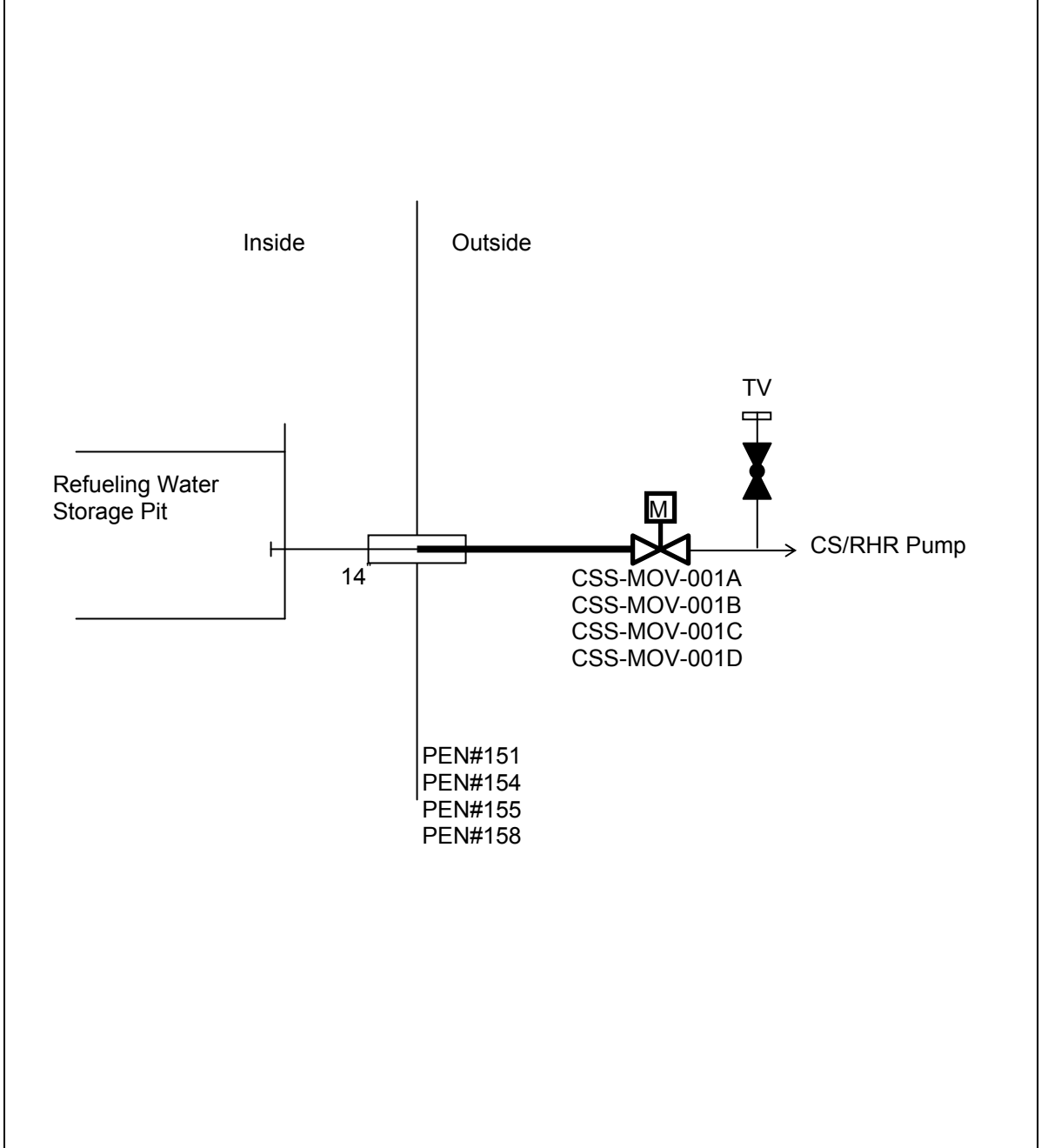
Figure 6.2.4-1 Containment Isolation Configurations (Sheet 18 of 51)
