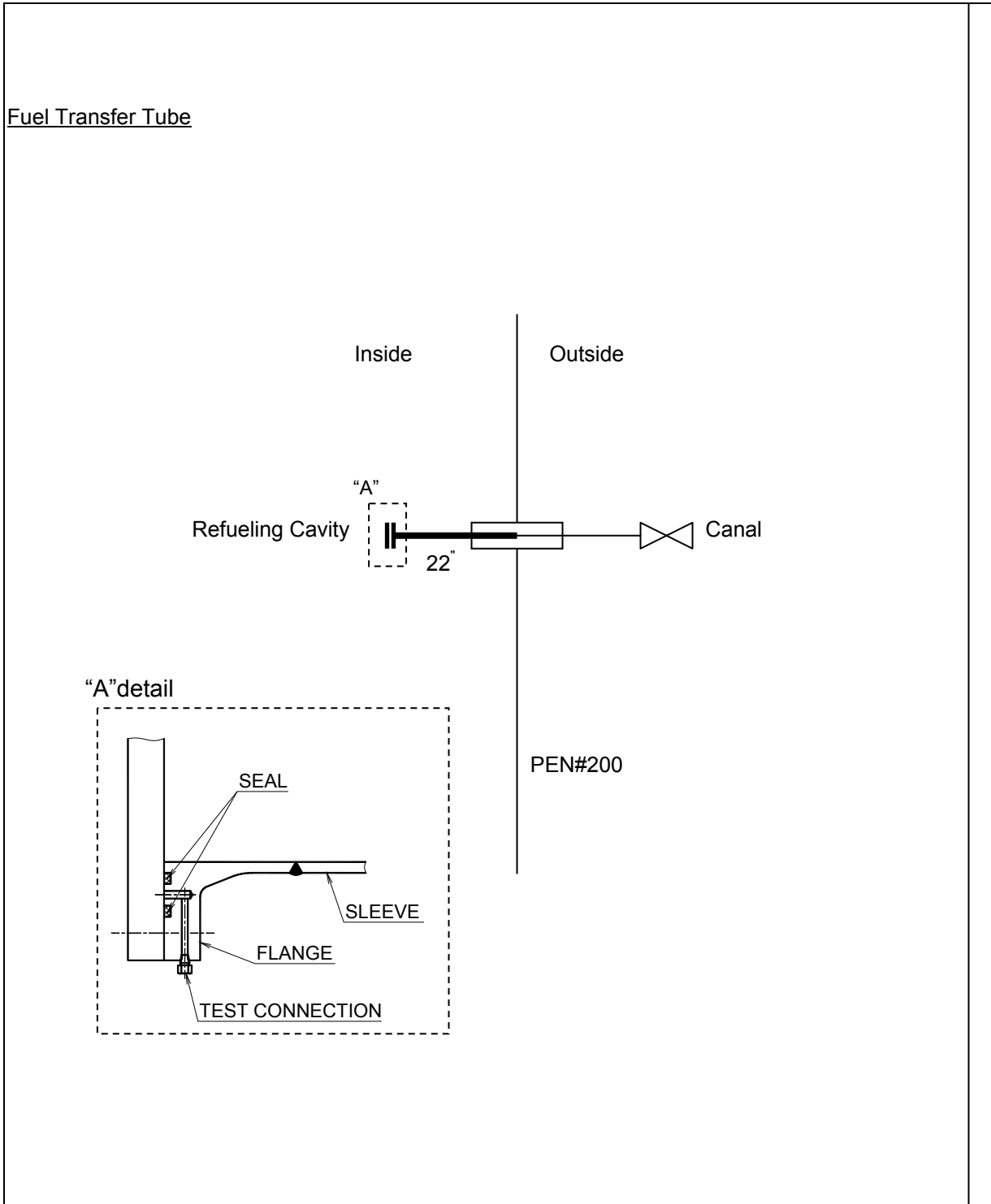
Figure 6.2.4-1 Containment Isolation Configurations (Sheet 39 of 51)
