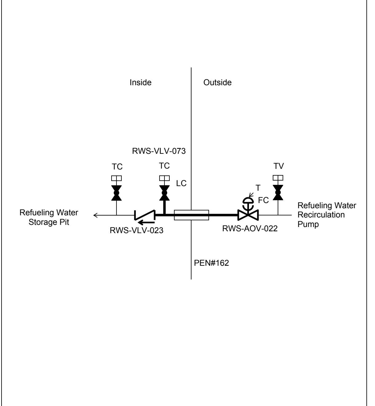
Figure 6.2.4-1 Containment Isolation Configurations (Sheet 33 of 51)
