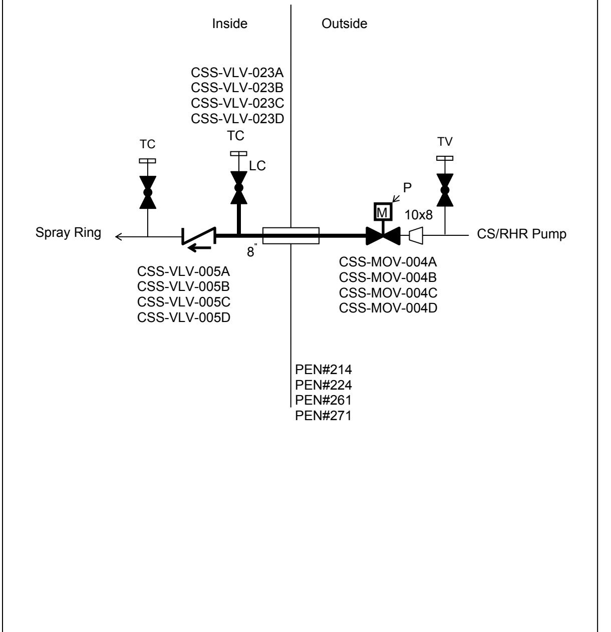
Figure 6.2.4-1 Containment Isolation Configurations (Sheet 16 of 51)
