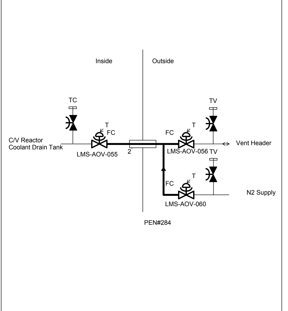
Figure 6.2.4-1 Containment Isolation Configurations (Sheet 24 of 51)
