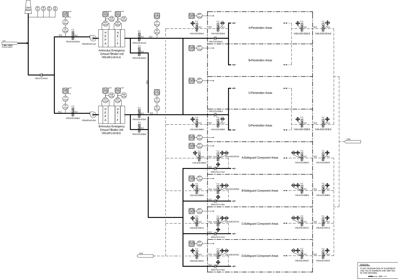
Figure 6.5-1 Annulus Emergency Exhaust System - Simplified Flow Diagram
