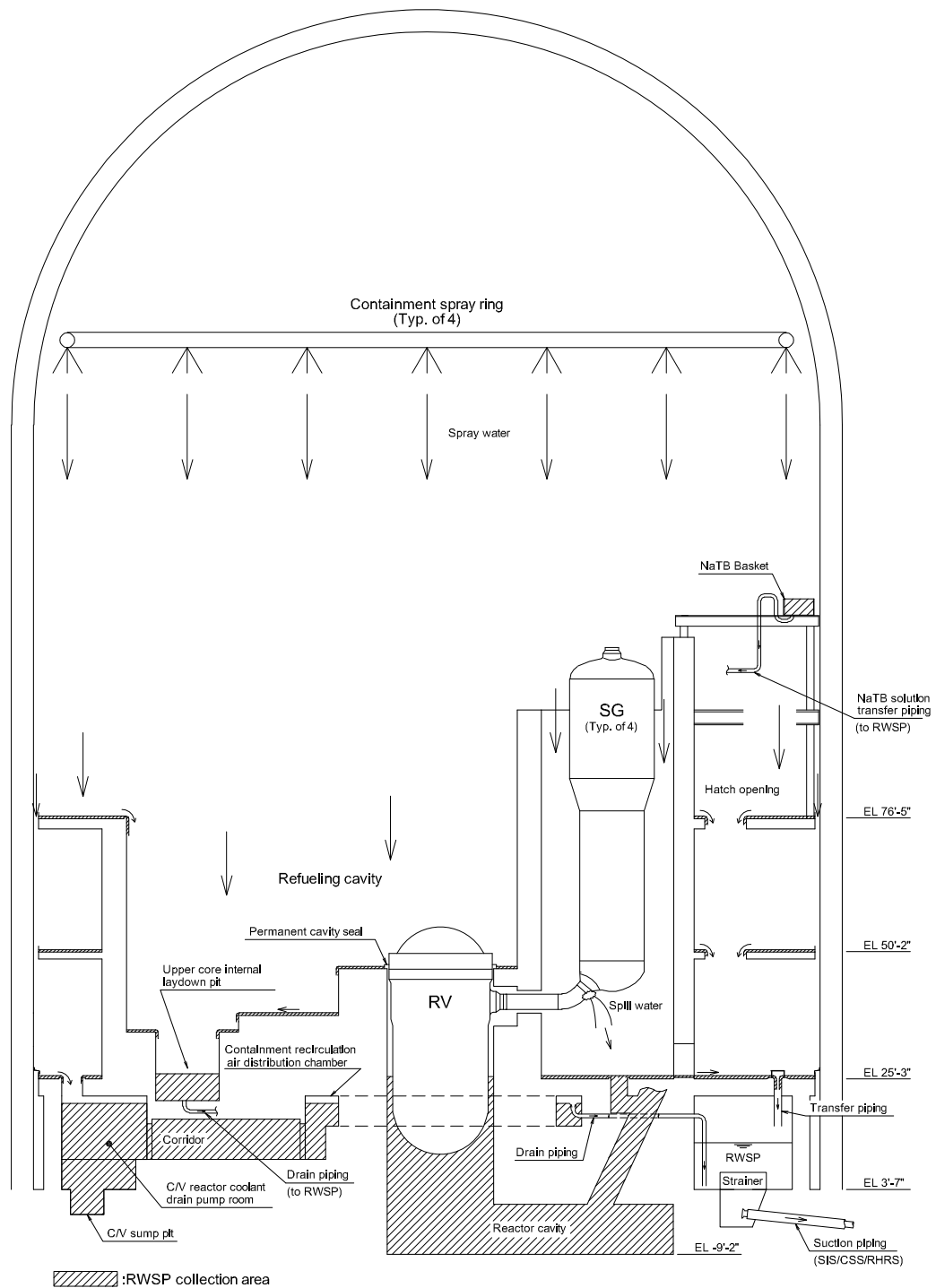
Figure 6.2.1-9 Outline of Paths that Solutions from the ECCS and CSS would follow in the Containment to the RWSP
