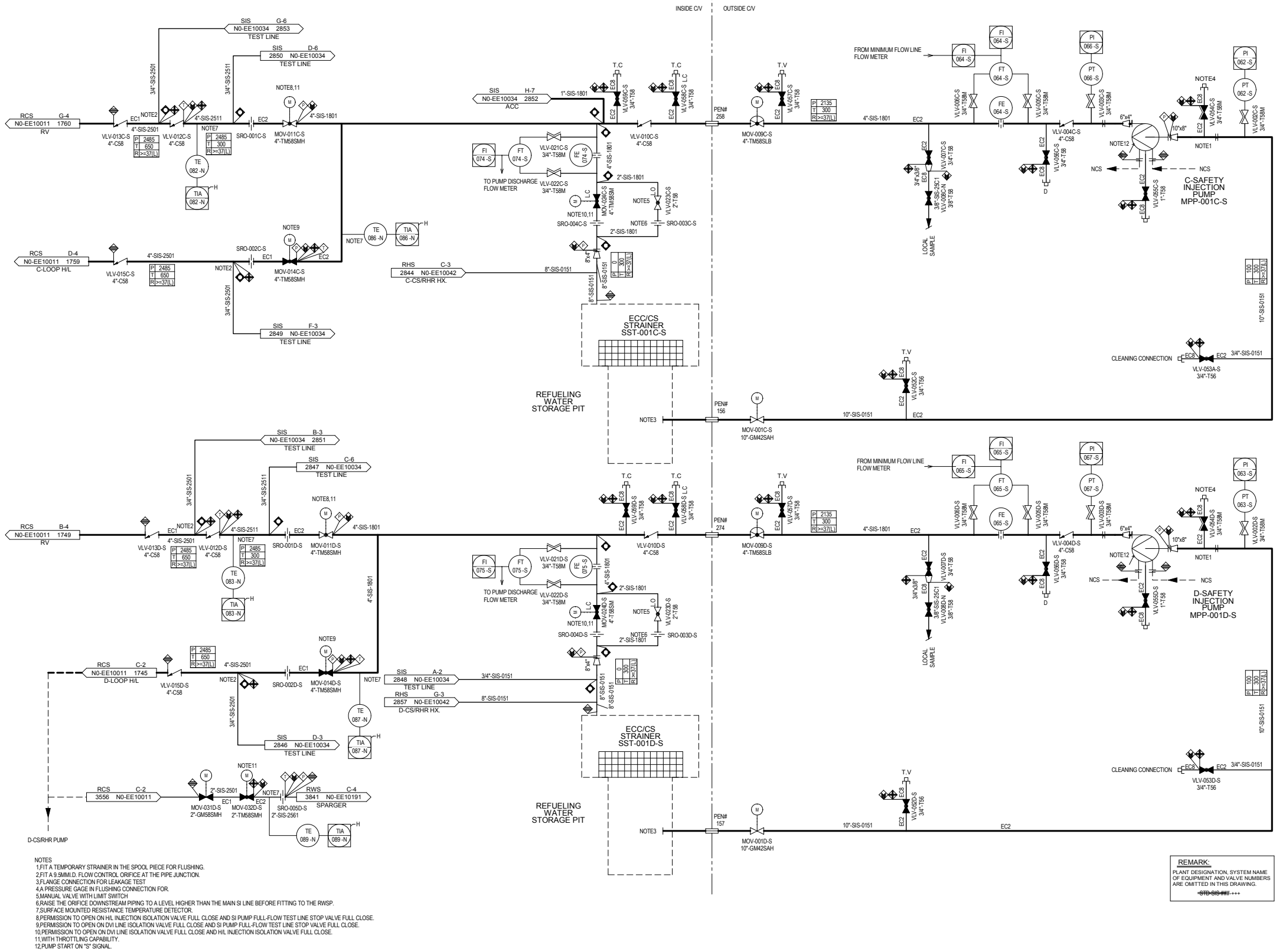
Figure 6.3-2 ECCS Piping and Instrumentation Diagram(Sheet 2 of 4)
