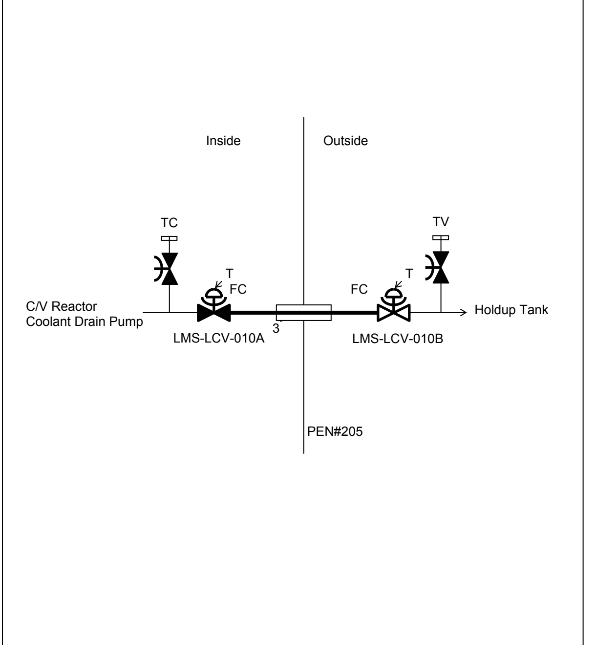
Figure 6.2.4-1 Containment Isolation Configurations (Sheet 25 of 51)
