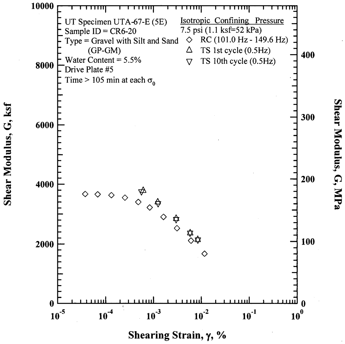
Figure E.11 Comparison of the Variation in Shear Modulus with Shearing Strain at an Isotropic Confining Pressure of 7.5 psi (1.1 ksf=52 kPa) from Combined RCTS Tests of Specimen UTA-67-E (5E)
