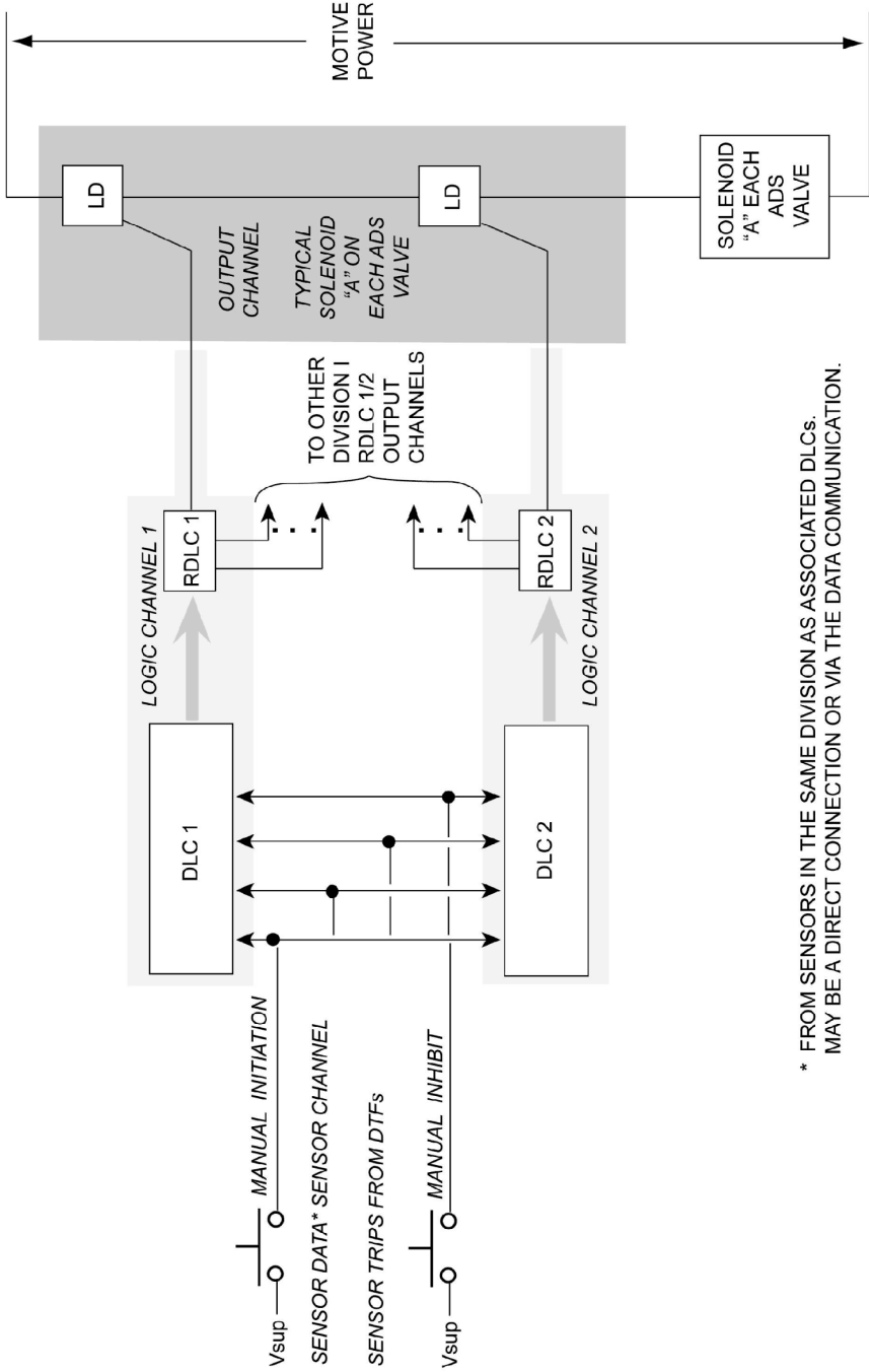
FIGURE B3.3.1.4-4 ESF ACTUATION CHANNEL STRUCTURE FOR ADS
