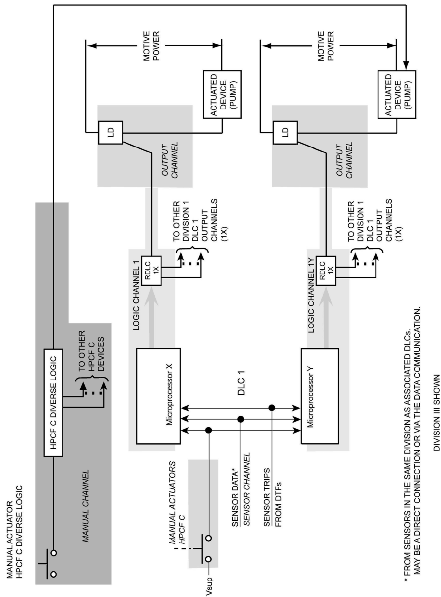
FIGURE B3.3.1.4-3 ESF ACTUATION CHANNEL STRUCTURE FOR HPCF C
