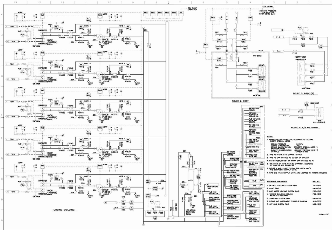
Figure 9.2-2 – Hvac Normal Cooling Water System P&ID
