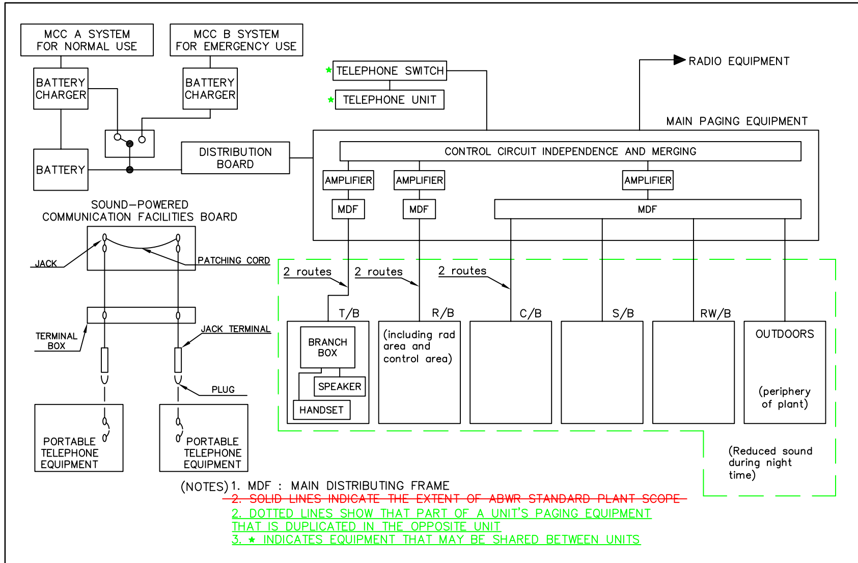
Figure 9.5-2 Outline - Telephonic Communication System for Single Unit of STP 3 or 4
