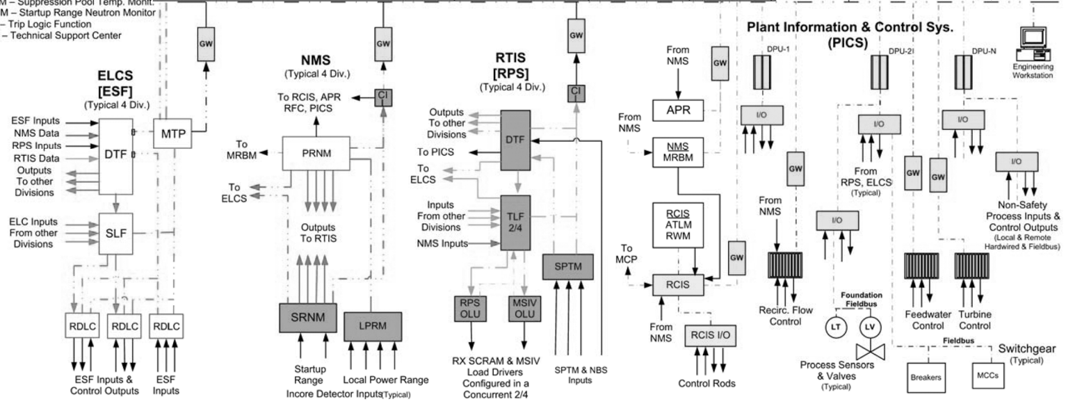
Figure 7.9S-1 Data Communication Interfaces
