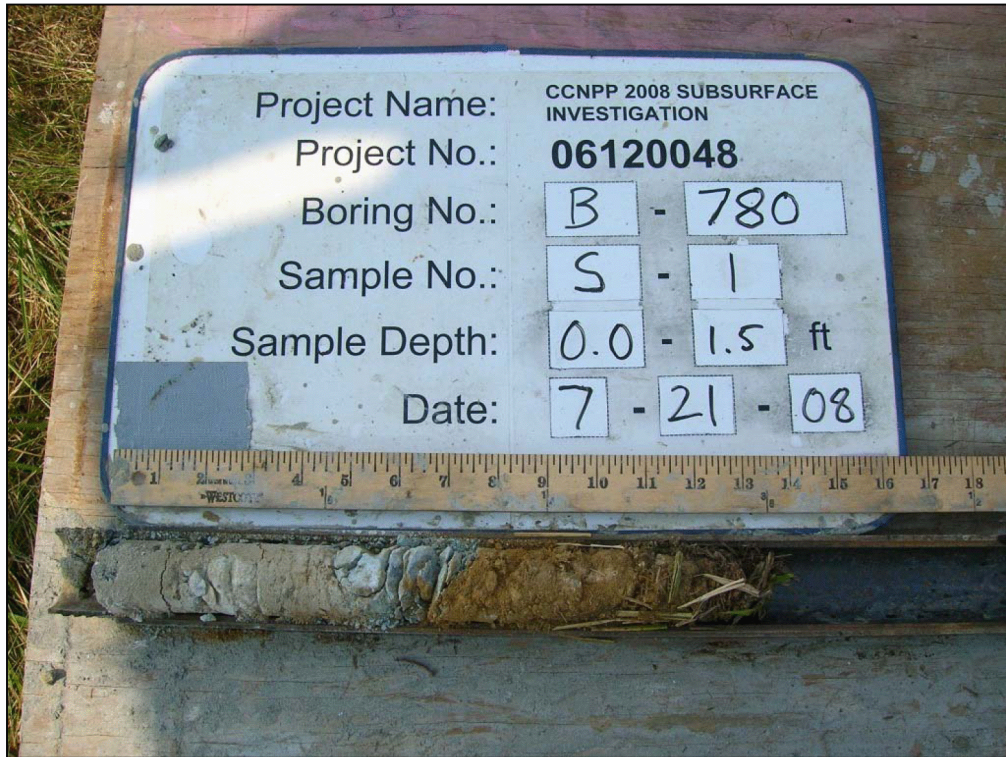
B-780; S-1 0.0 – 1.5 ft
