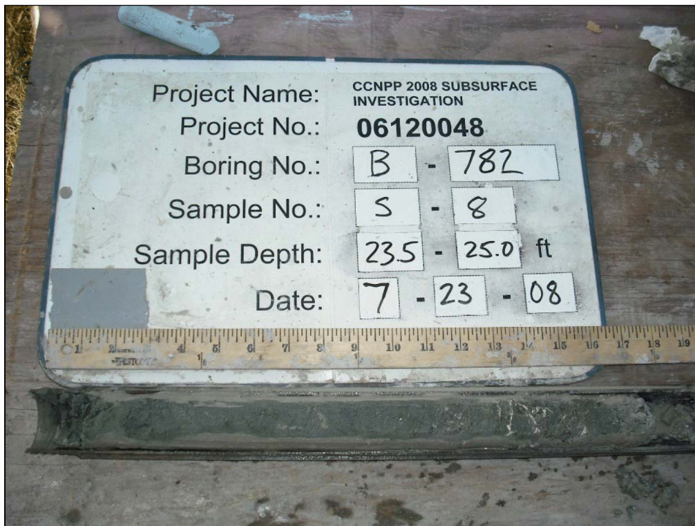
B-782; S-8 23.5 – 25.0 ft
