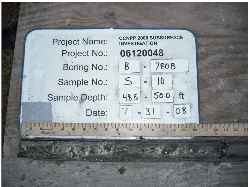
B-780B; S-10 48.5 – 50.0 ft
