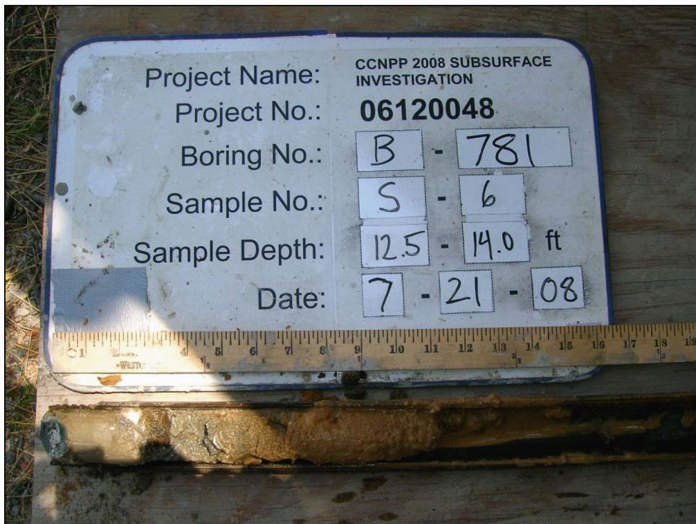
B-781; S-6 12.5 – 14.0 ft
