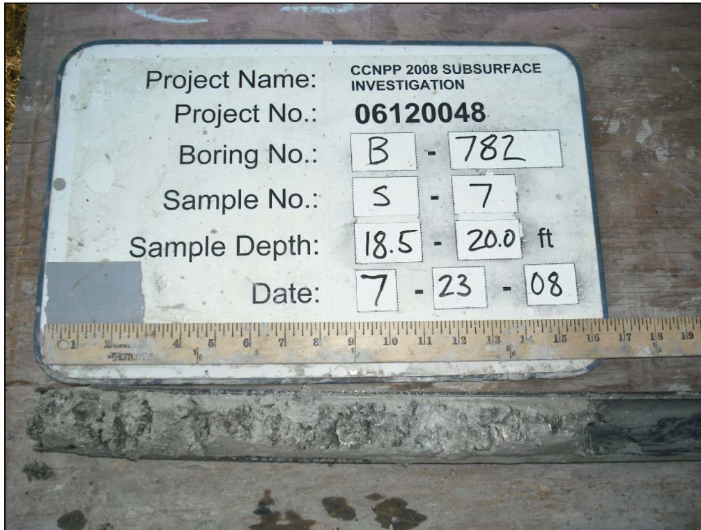
B-782; S-7 18.5 – 20.0 ft
