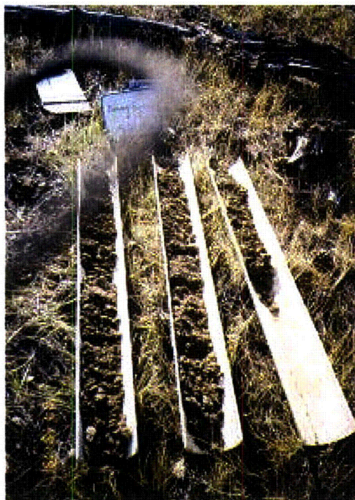
Photo 41: Hole 79 Profile
