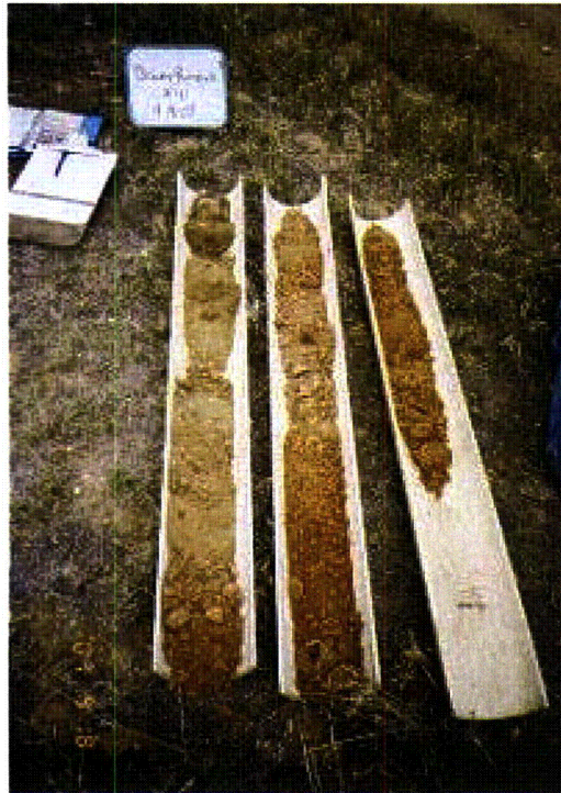
Photo 11: Hole 41 Profile
