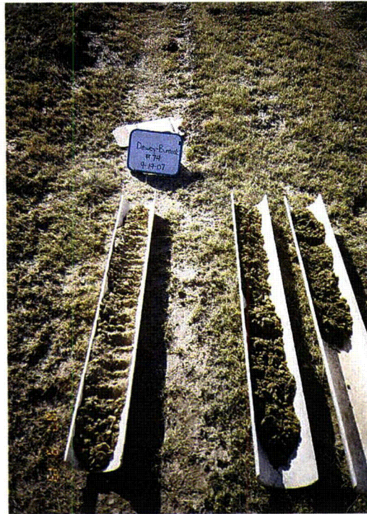
Photo 33: Hole 74 Profile
