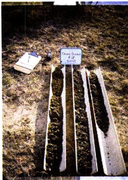
Photo 3: Hole 27 Profile
