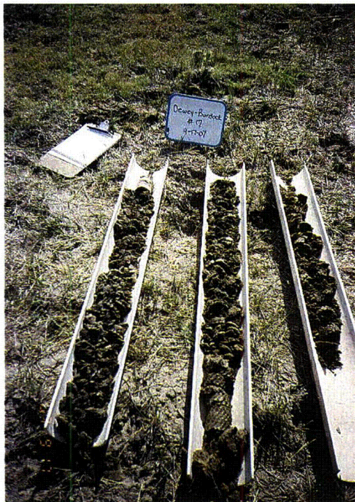
Photo 1: Hole 17 Profile
