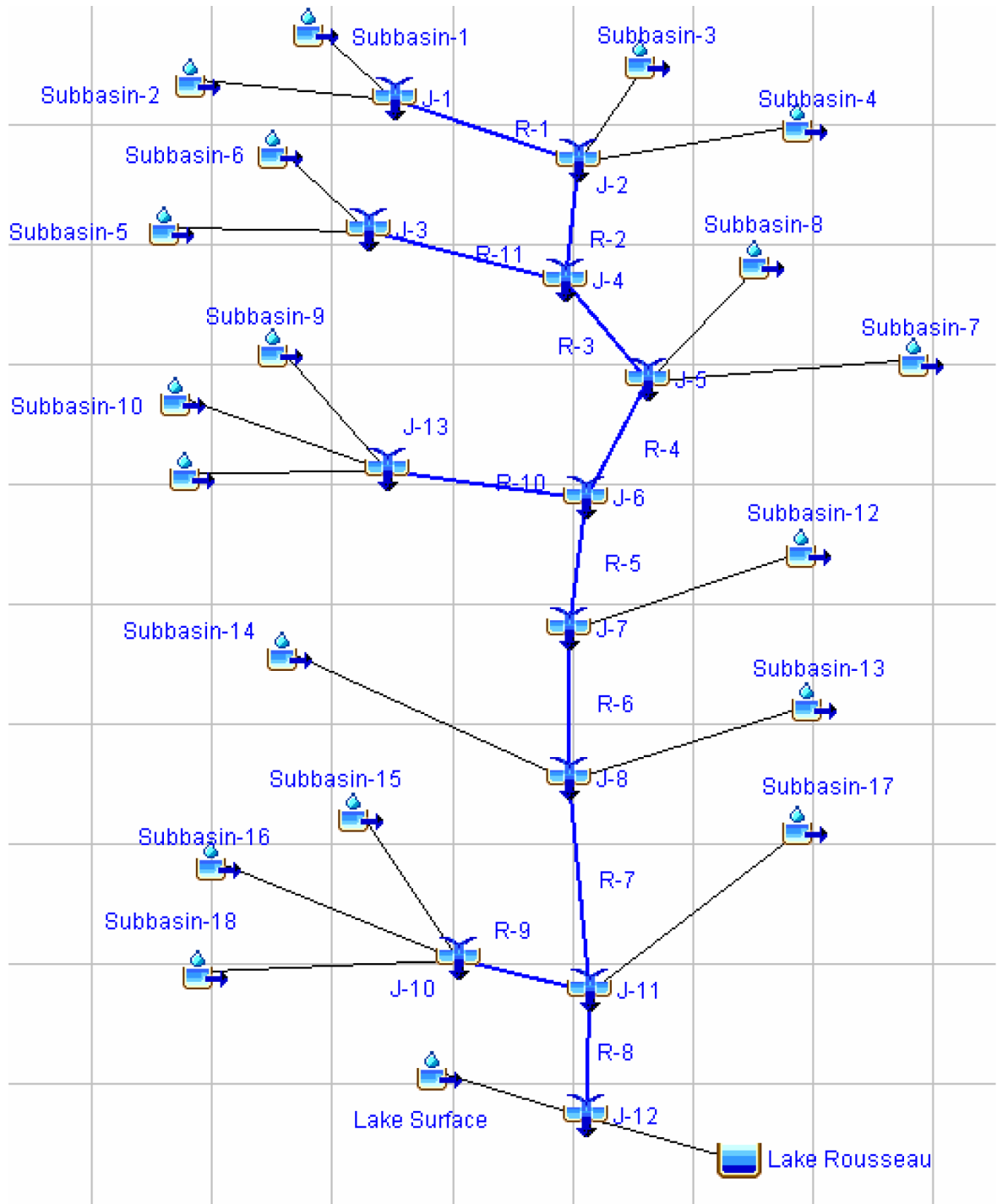
Progress Energy Florida Levy Nuclear Plant Units 1 and 2 Part 2, Final Safety Analysis Report Schematic of Basin Elements and their Connectivity FIGURE 2.4.3-214 Rev 0
