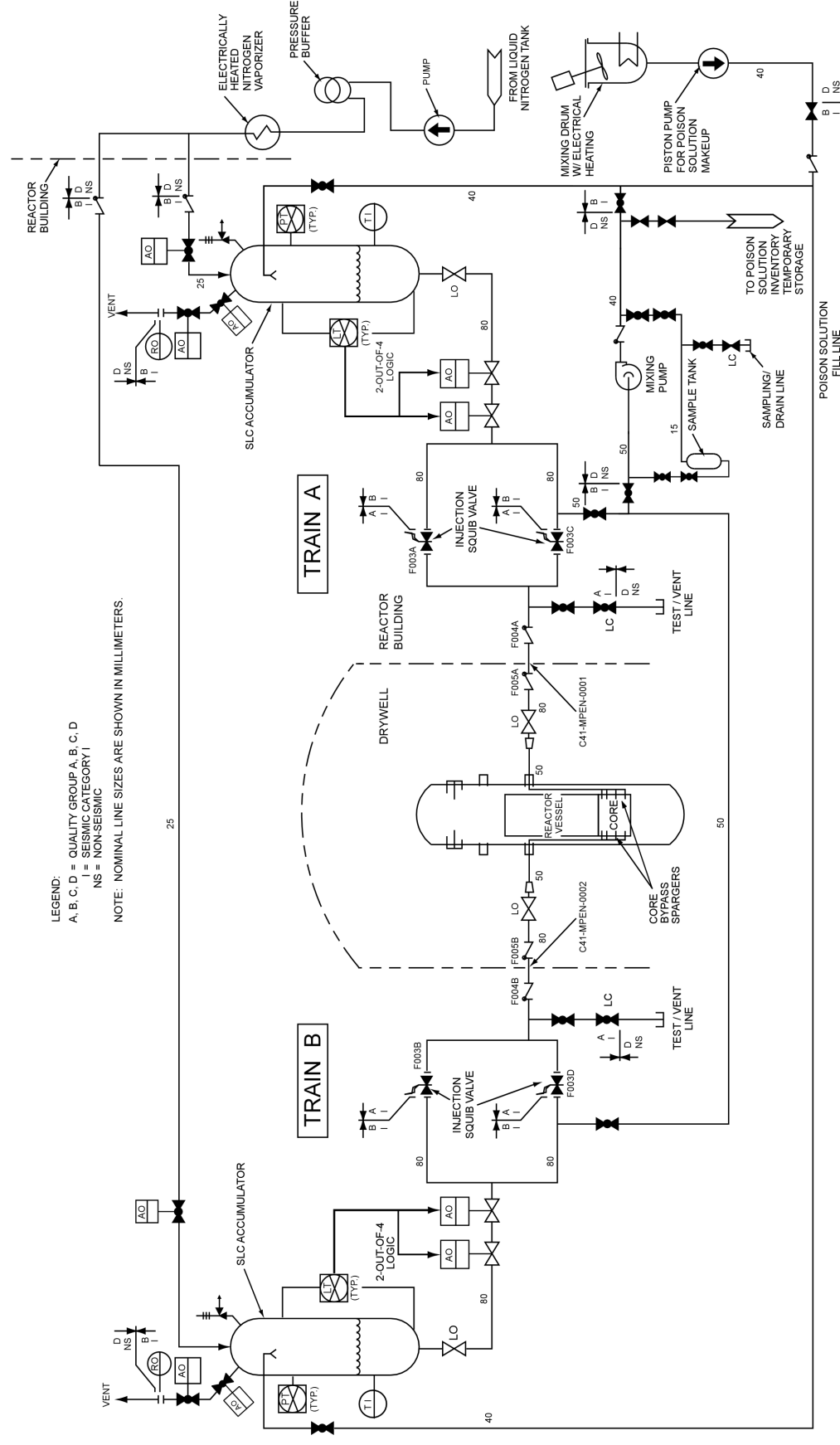
Figure 9.3-1. Standby Liquid Control System Simplified Diagram
