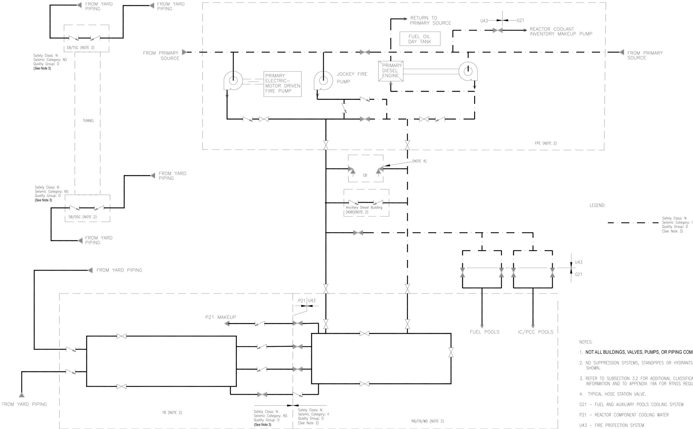
Figure 9.5-1. Fire Protection System Simplified Diagram
