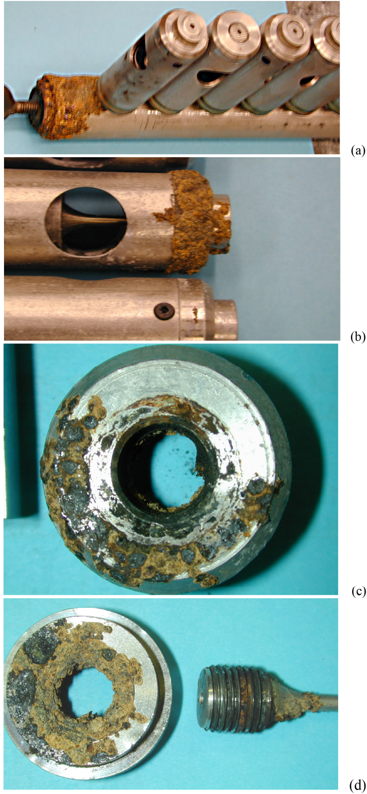
Figure 2-7. Severe corrosion and encrustation was observed (a) at the top of the manifold and (b) - (d) on several module components and 304SS specimens after running the autoclave at 125°C.
