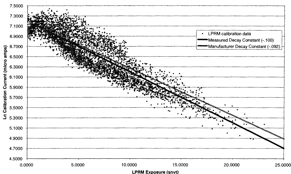
Figure 1. LaSalle Station LPRM Decay Constant
