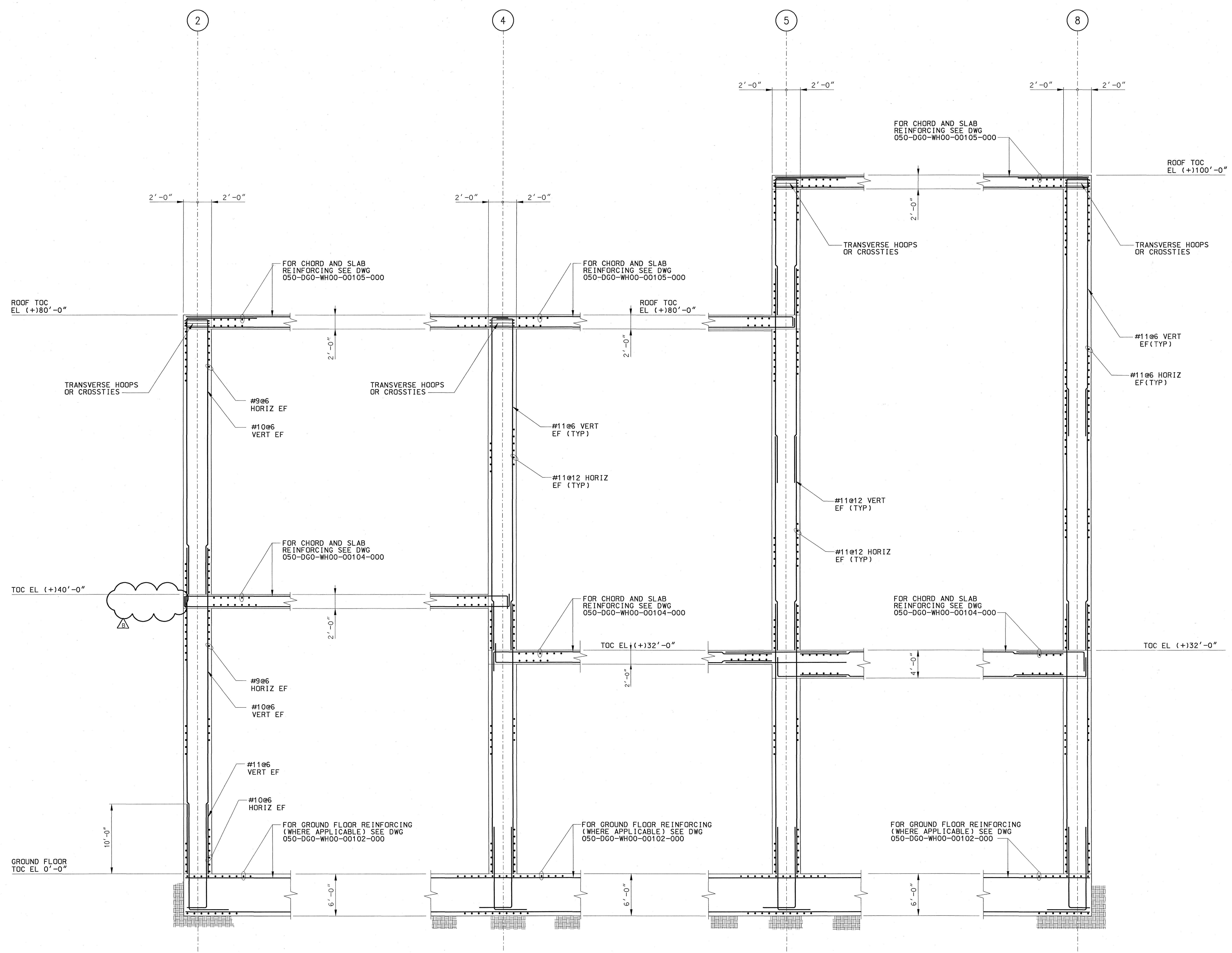
SECTION A 00102
