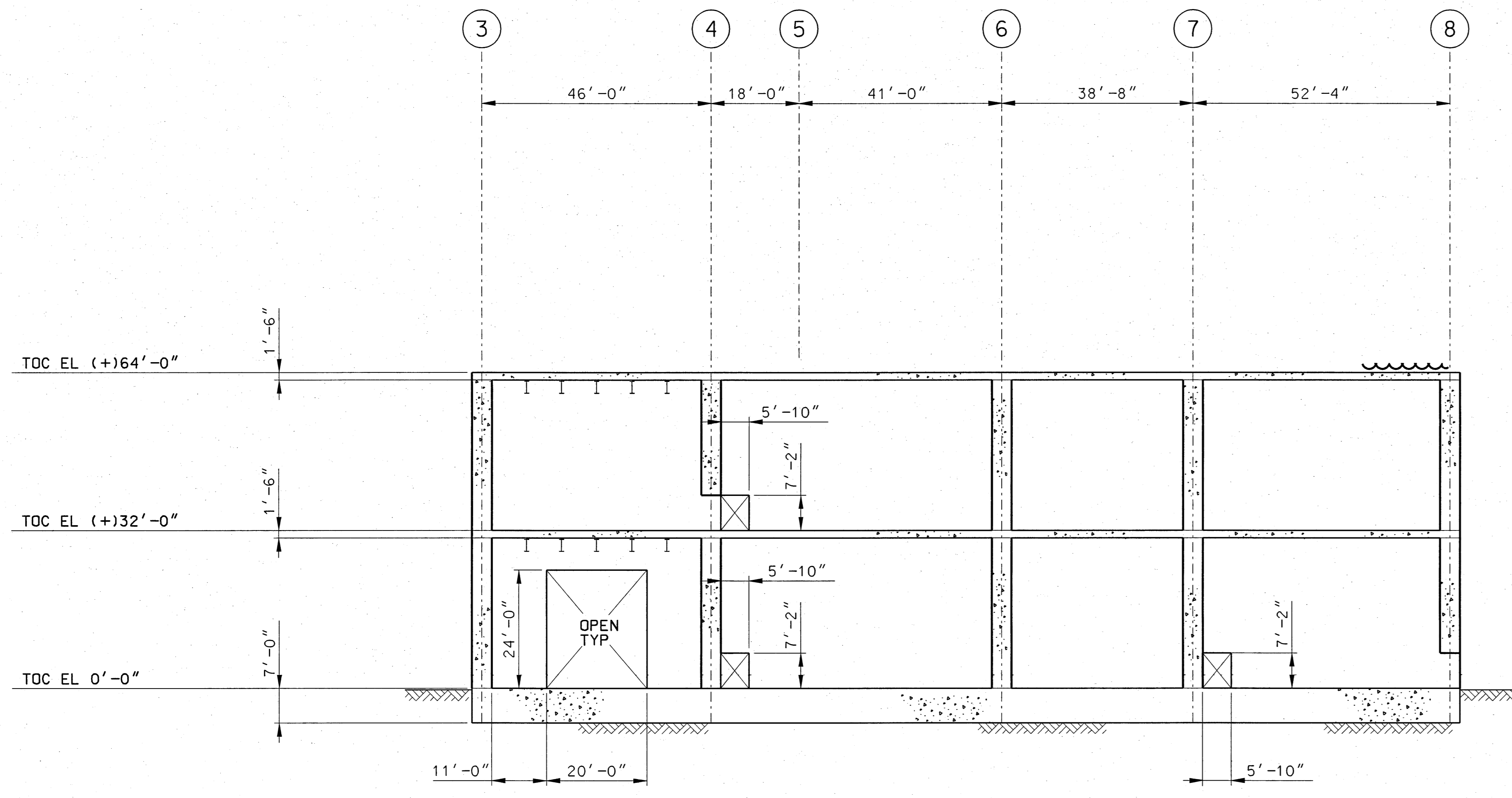
ELEVATION ALONG COLUMN "A" (LOOKING NORTH)
