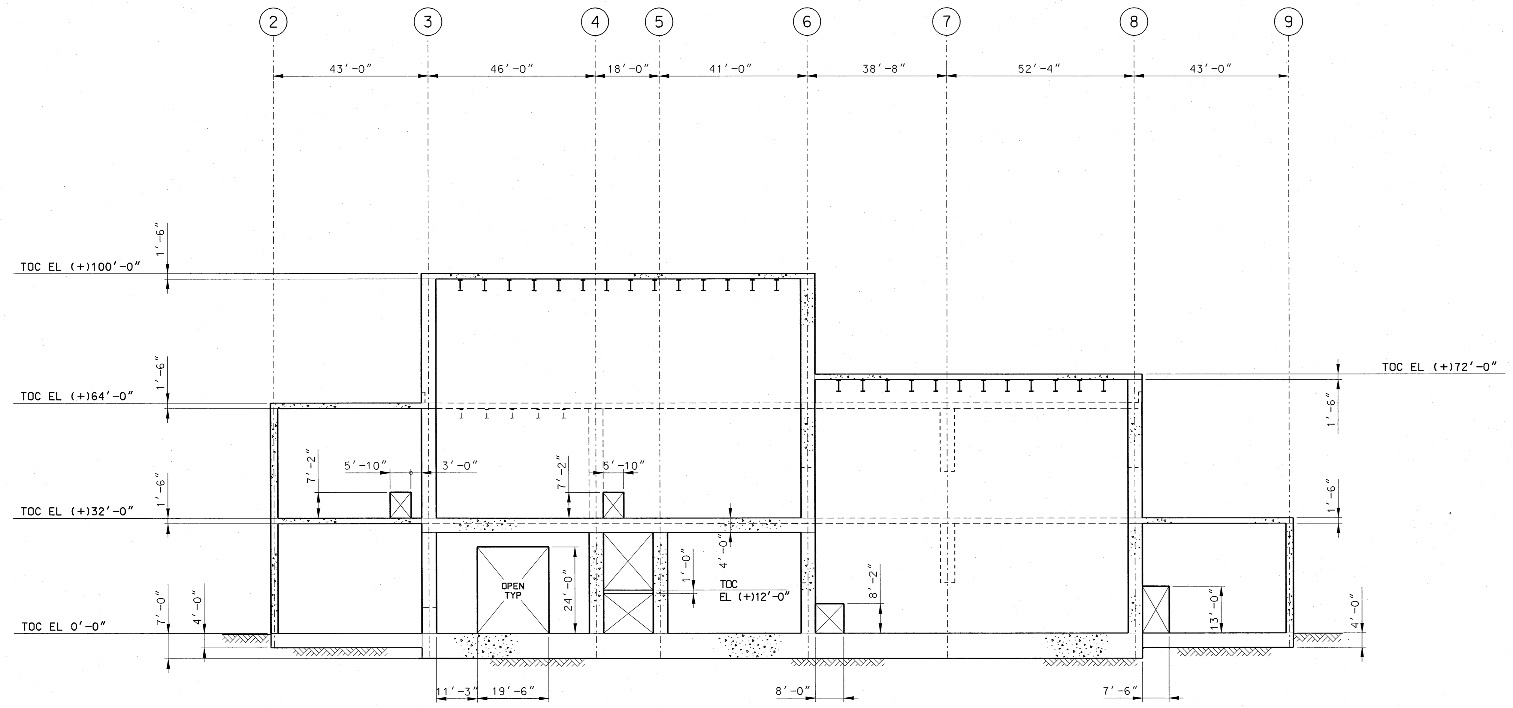
ELEVATION ALONG COLUMN "C" (LOOKING NORTH)
