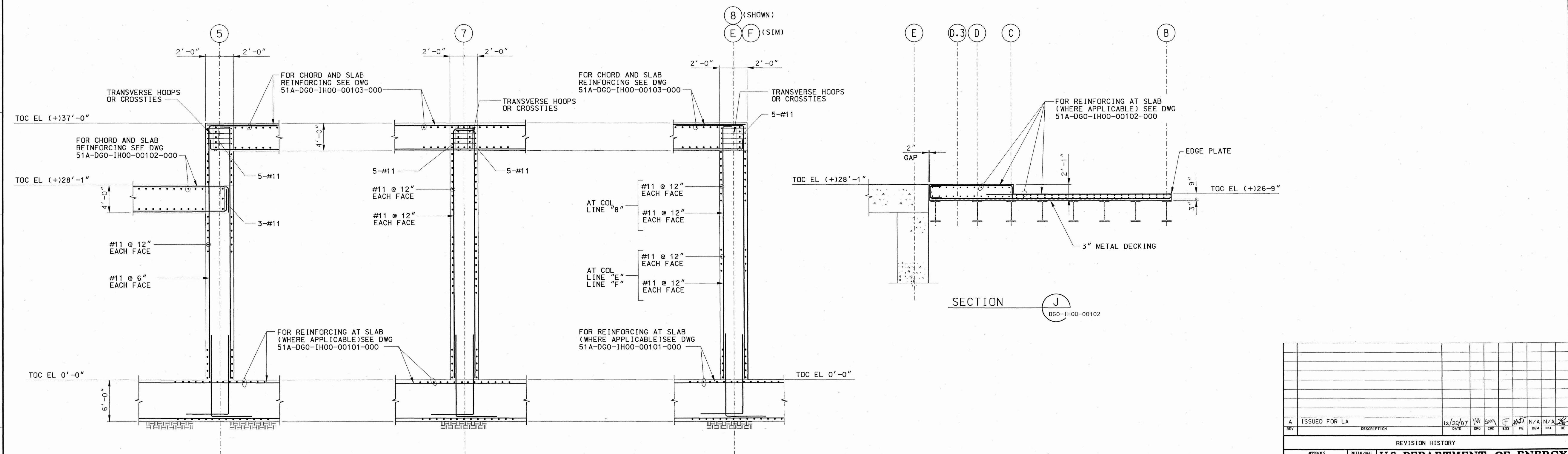
SECTION F DGO-IH00-00101, 00102, 00103 SECTION G DGO-IH00-00101, 00102, 00103 SECTION H DGO-IH00-00101, 00102, 00103 SECTION J DGO-IH00-00102
