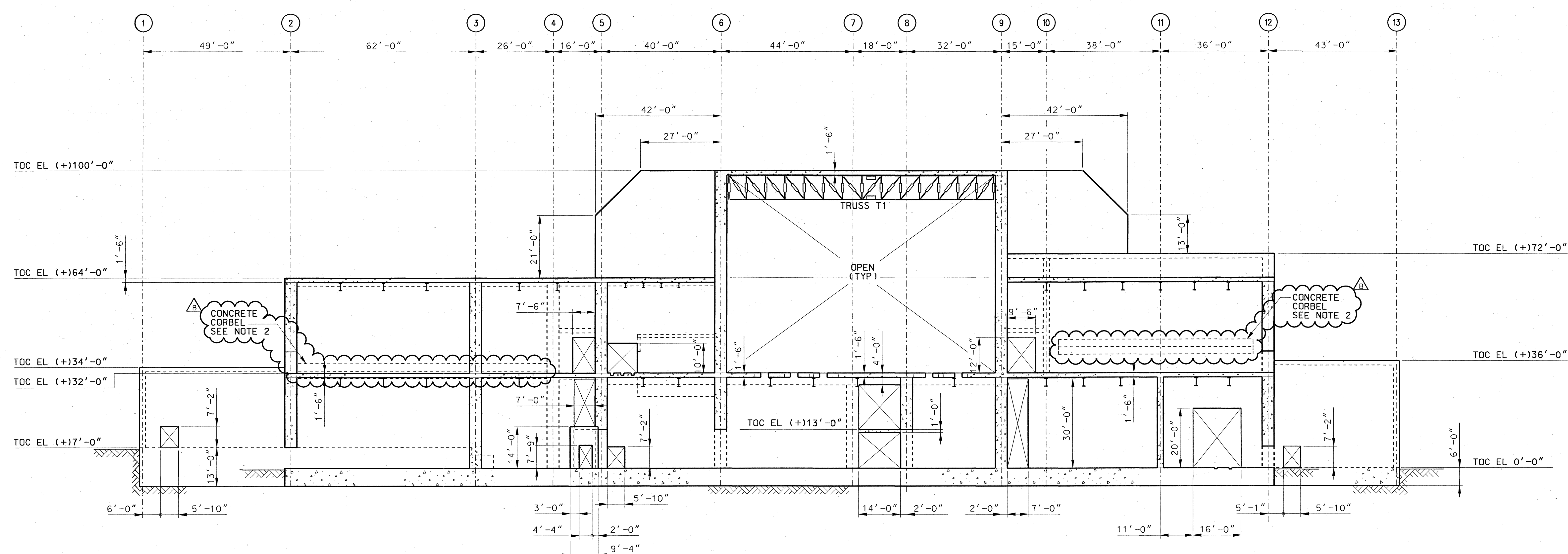
ELEVATION ALONG COLUMN "G" (LOOKING NORTH)
