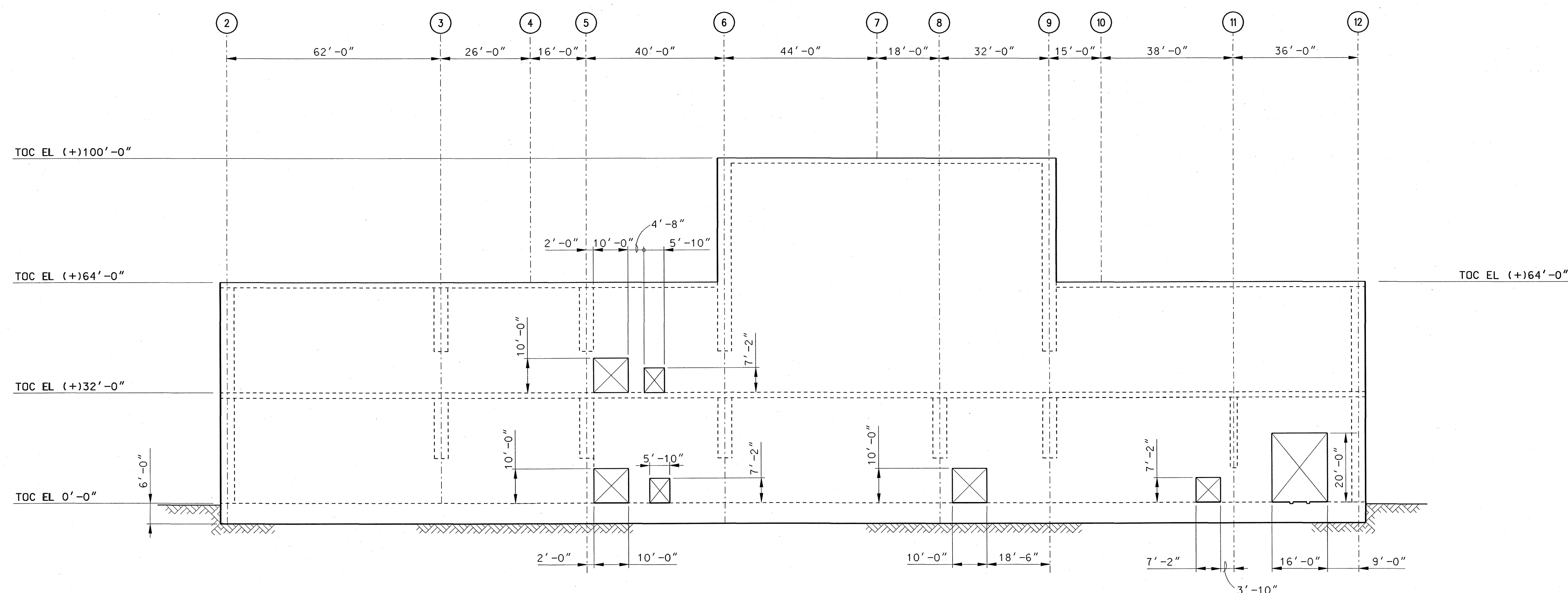
ELEVATION ALONG COLUMN "H" (LOOKING NORTH)
