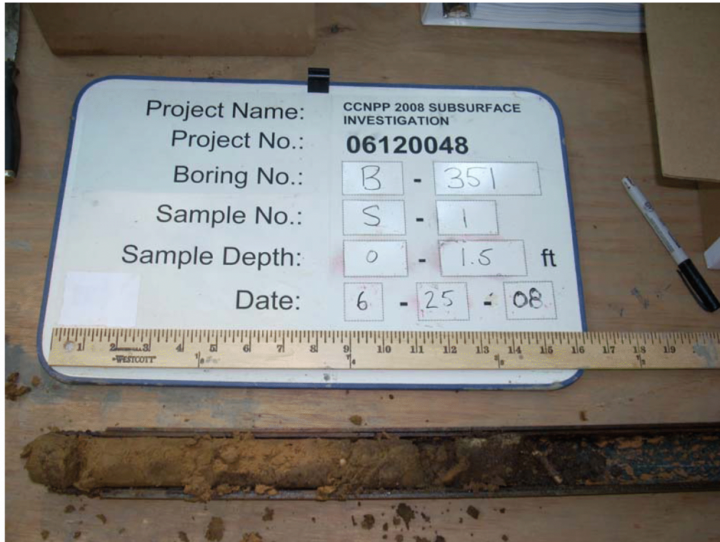
B-351; S-1 0.0 – 1.5 ft
