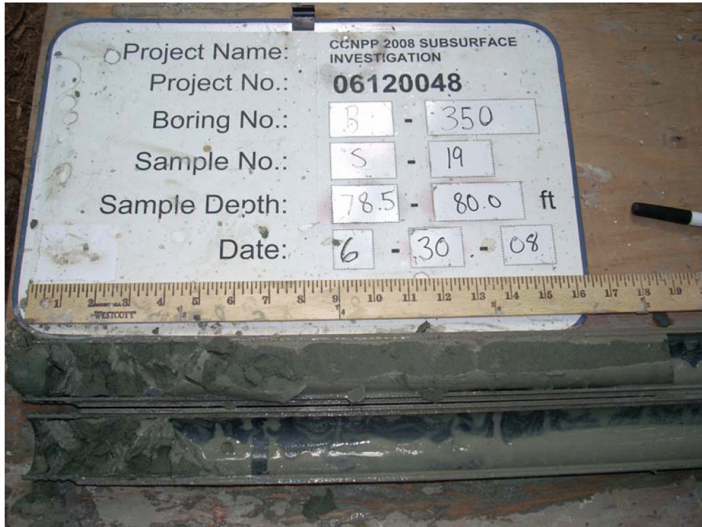
B-350; S-19 78.5 – 80.0 ft
