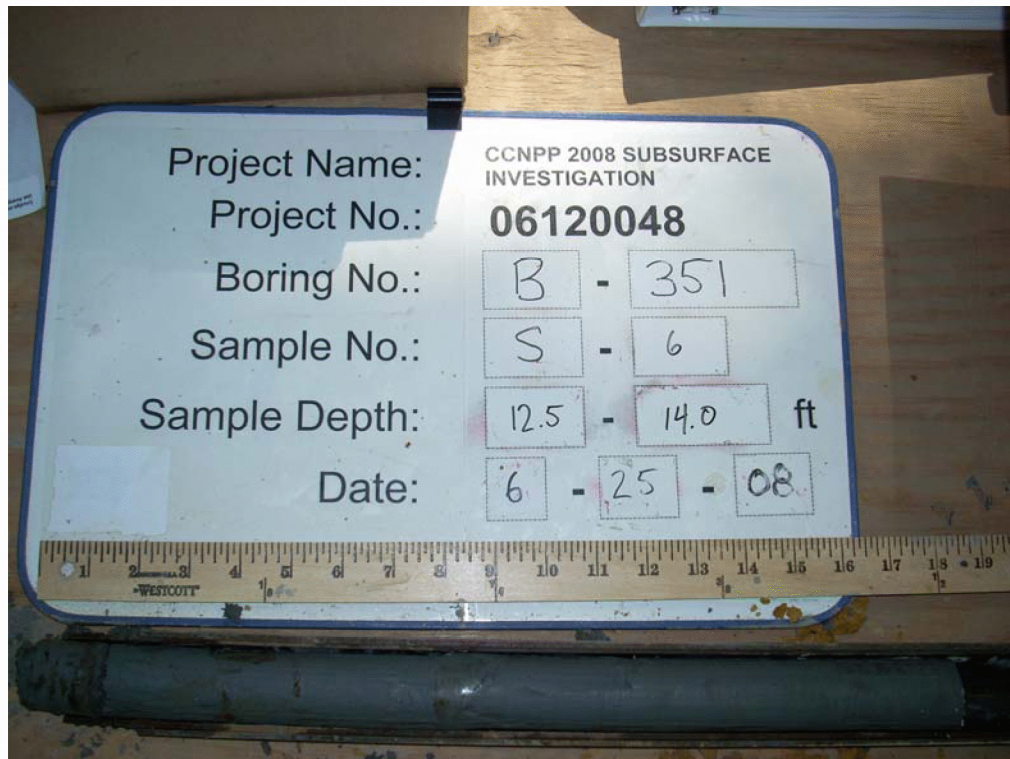
B-351; S-6 12.5 – 14.0 ft
