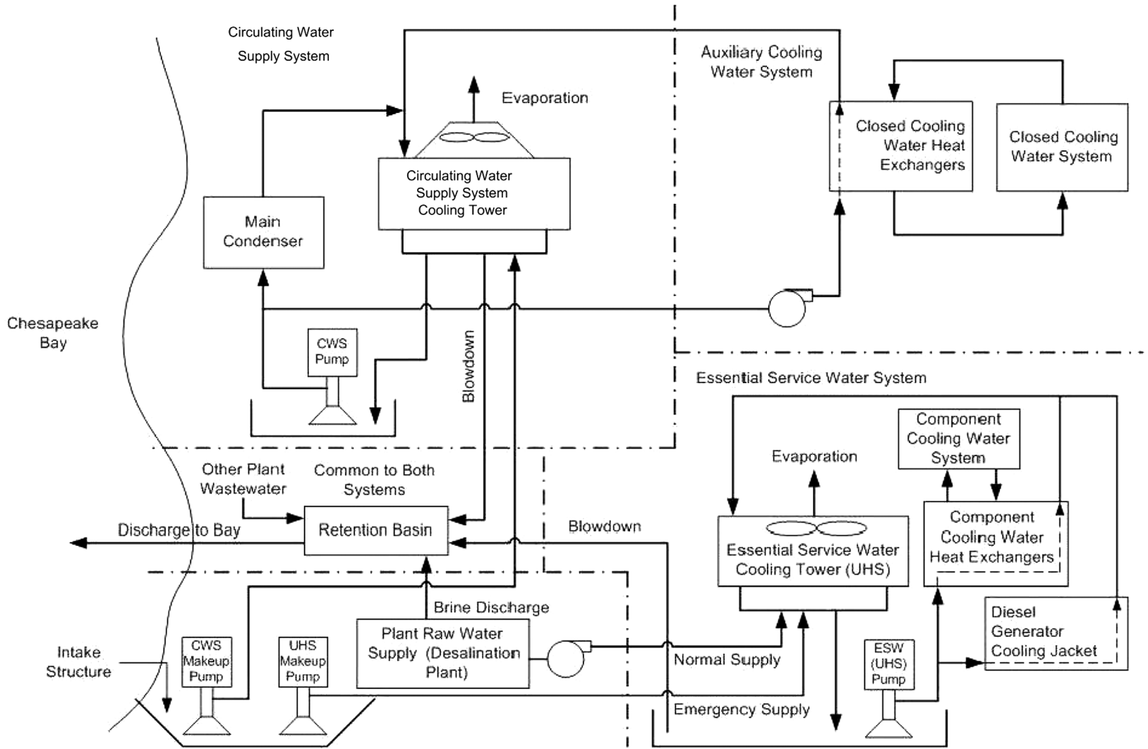
Figure 1.2-3—General Cooling System Flow Diagram for CCNPP Unit 3
