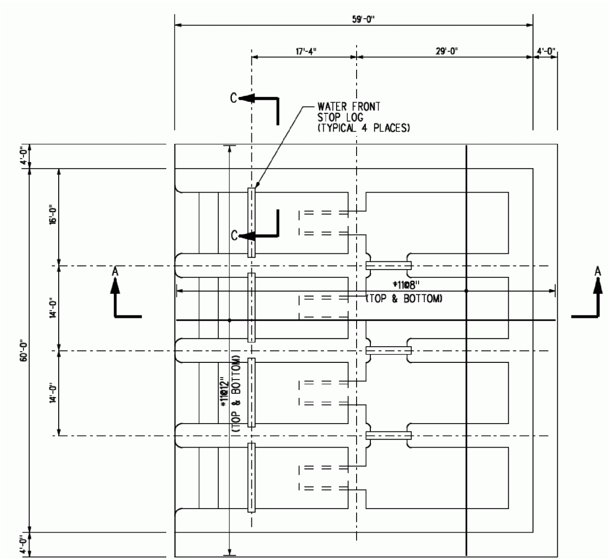
Figure 3E.4-1—{Foundation Plan for the UHS Makeup Water Intake Structure @ Elevation -20.5 -22.5 ft ( -6.25 -6.86 m)}
