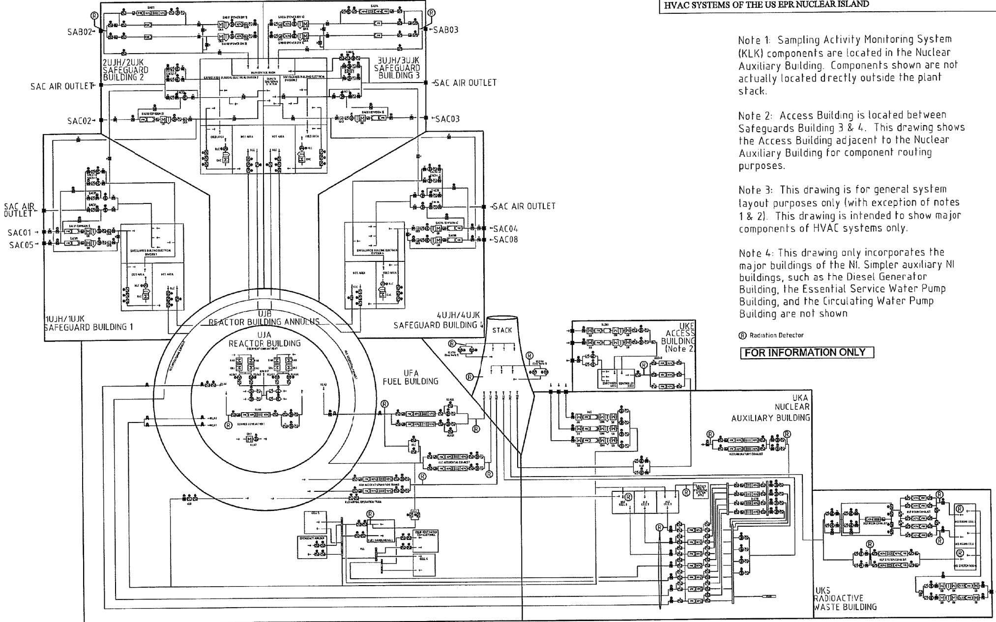
FIGURE B-1 HVAC Systems of the US EPR Nuclear Island
