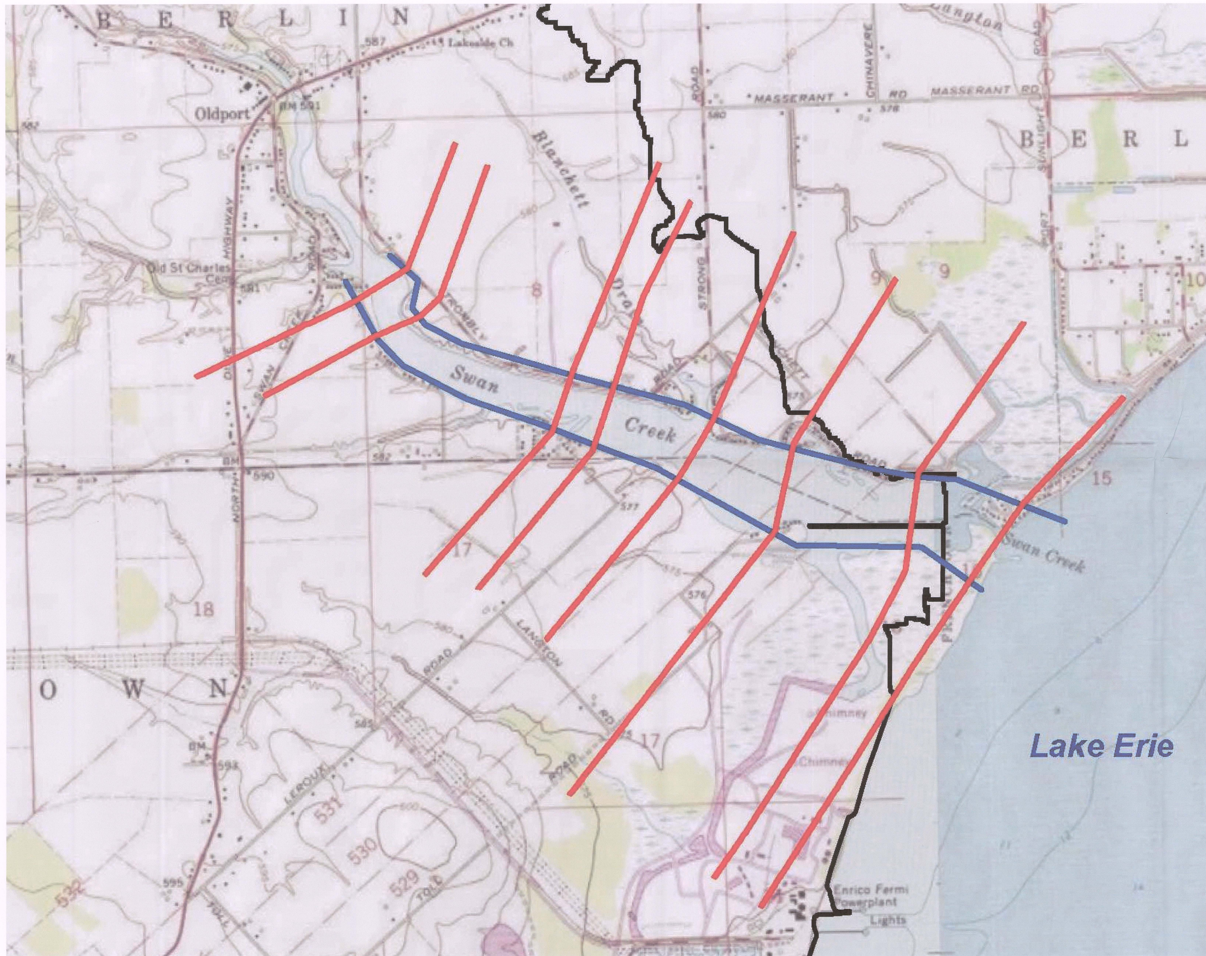
Drawing #4 Swan Creek with HEC-RAS Cross Sections Shown (Focused on Swan Creek Area)
