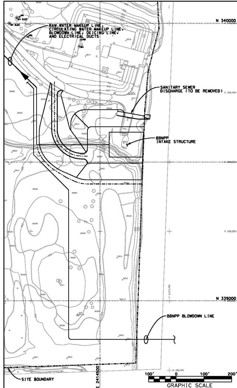
Figure 3.4-3 Circulating Water System Intake/Discharge Structure Location Plan
