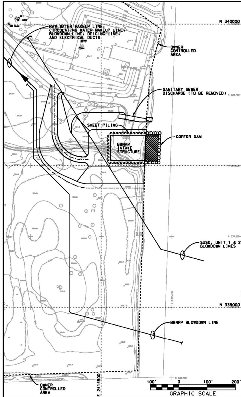
Figure 3.4-11 CWS Makeup Water Intake Structure Construction Cofferdam
