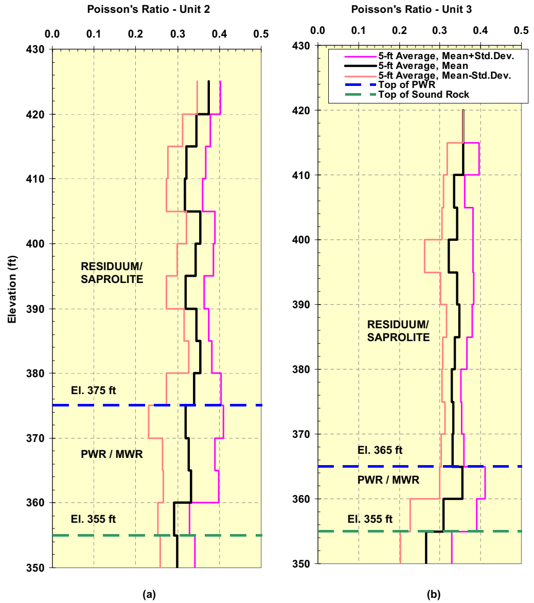
Figure 2.5.4-232. Poisson's Ratio of Layers I, II, III and IV with 5-feet Vertical Distance Averaging
