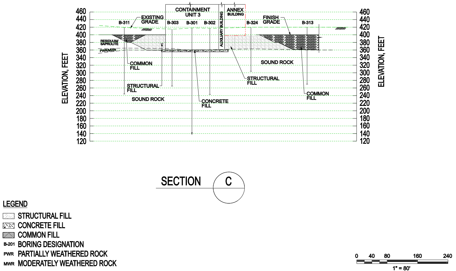
Figure 2.5.4-222. Cross-Section of Structure Foundations C-C
