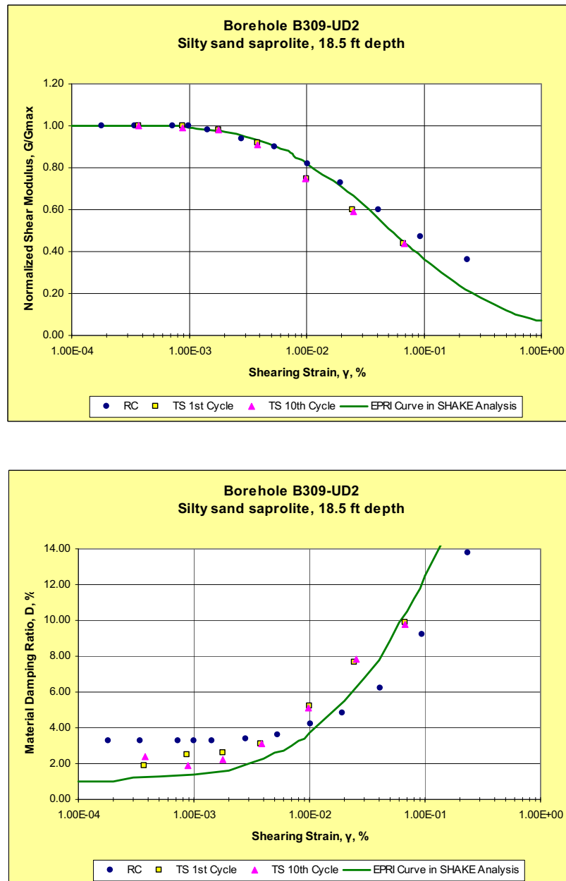
Figure 2.5.4-240. EPRI Curves for G/G_{MAX} and D Versus Shear Strain Superimposed on RCTS Results (Sheet 1 of 5)
