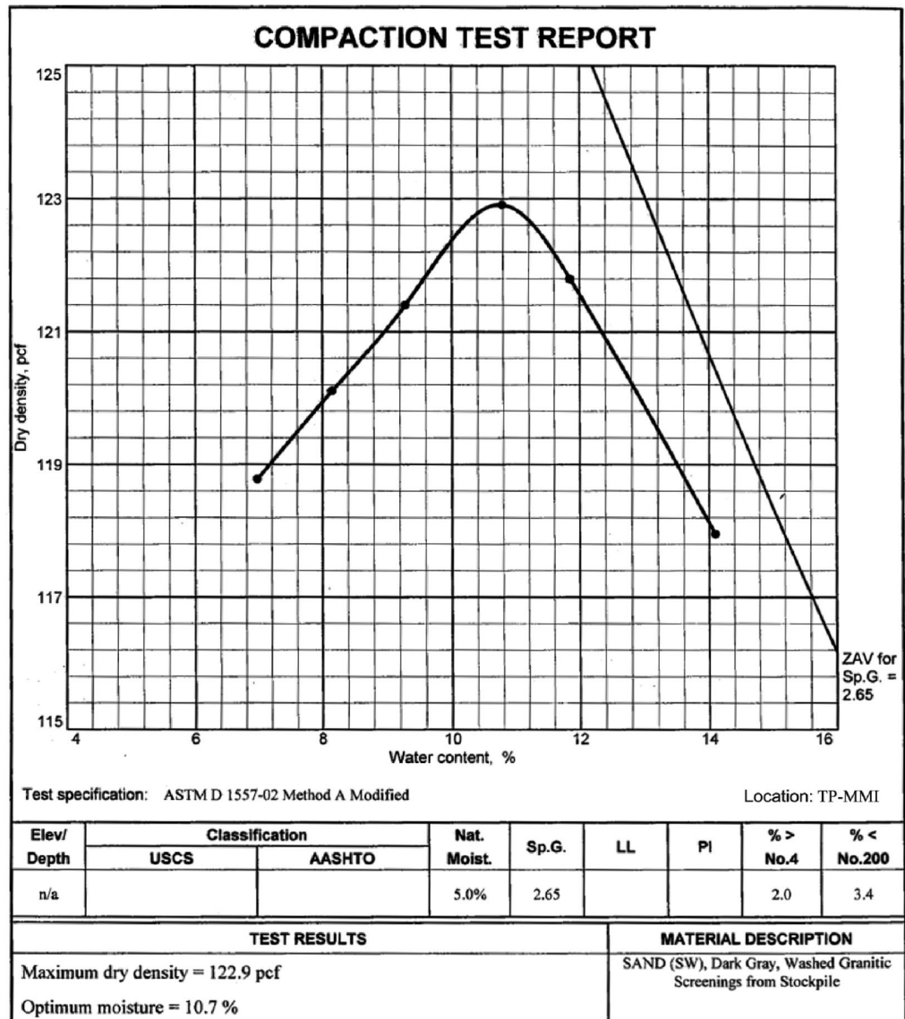
Figure 2.5.4-235. Modified Proctor Compaction on Fill Samples (Sheet 1 of 2)
