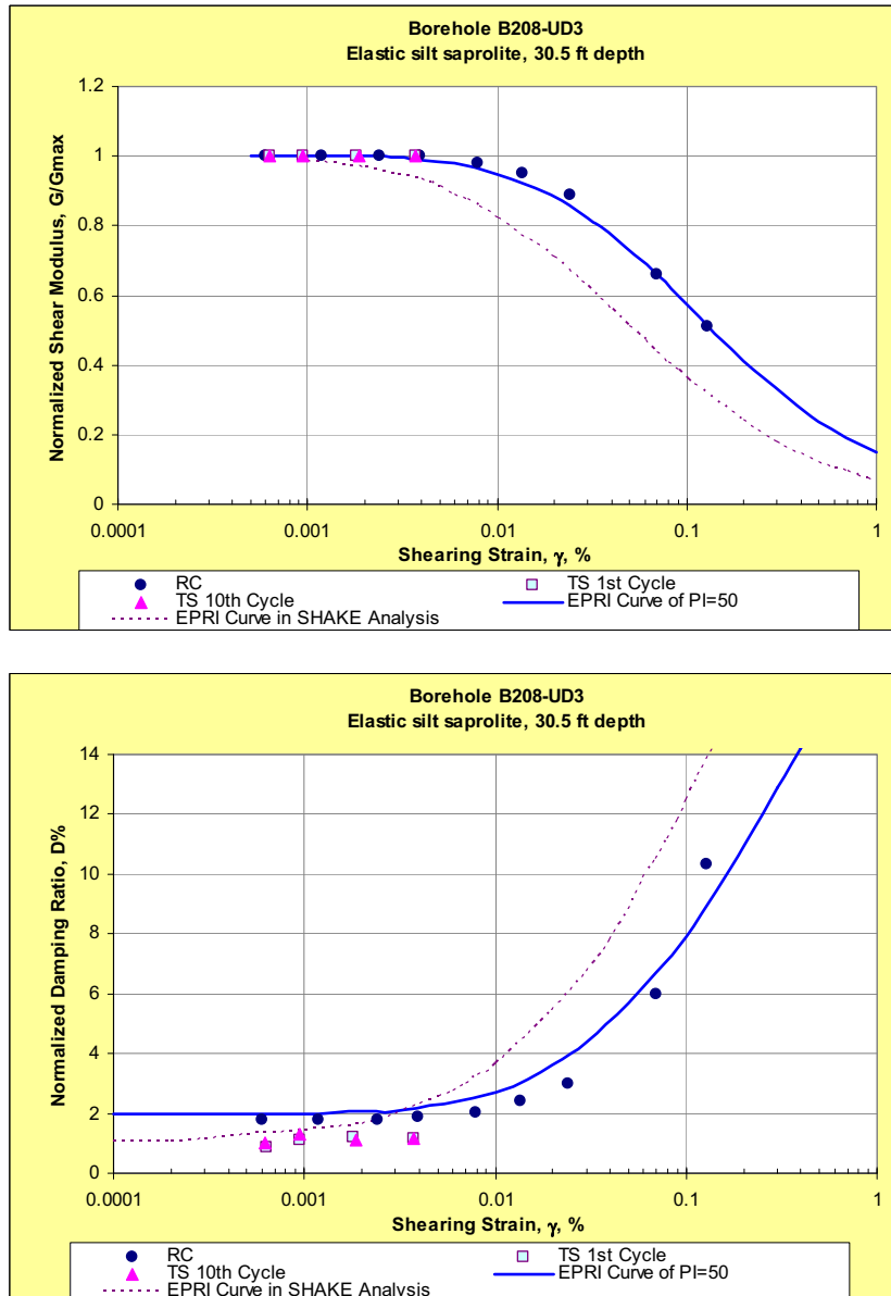
Figure 2.5.4-240. EPRI Curves for G/G_{MAX} and D versus Shear Strain Superimposed on RCTS Results (Sheet 3 of 5)
