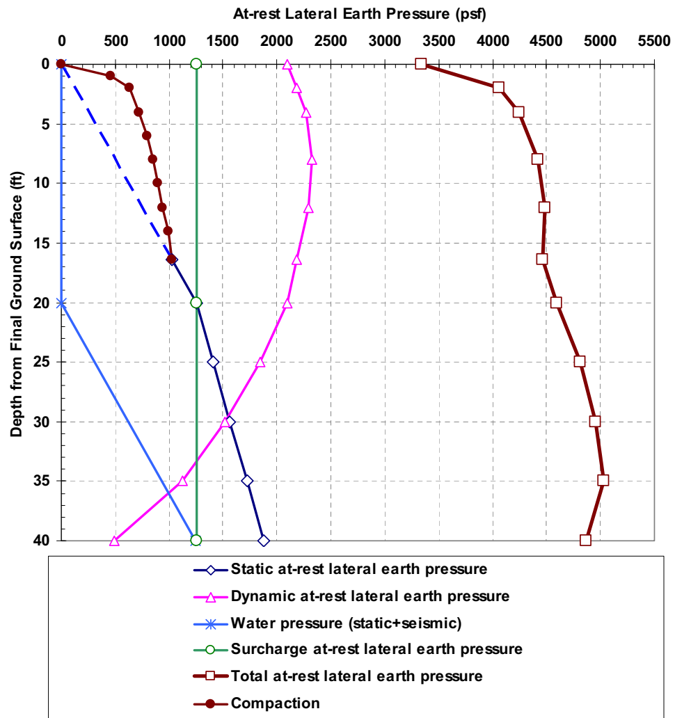
Figure 2.5.4-244. At-Res Rest Lateral Earth Pressure Diagrams
