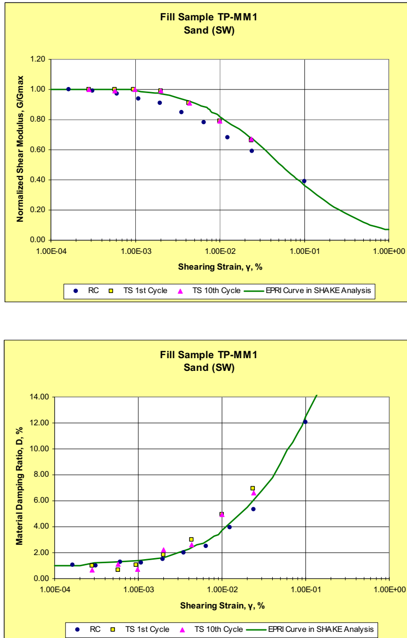
Figure 2.5.4-240. EPRI Curves for G/G_{MAX} and D Versus Shear Strain Superimposed on RCTS Results (Sheet 4 of 5)
