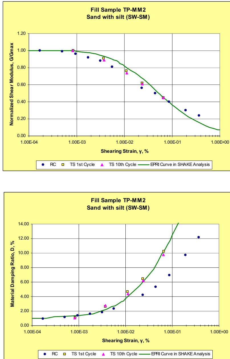
Figure 2.5.4-240. EPRI Curves for G/G_{MAX} and D Versus Shear Strain Superimposed on RCTS Results (Sheet 5 of 5)
