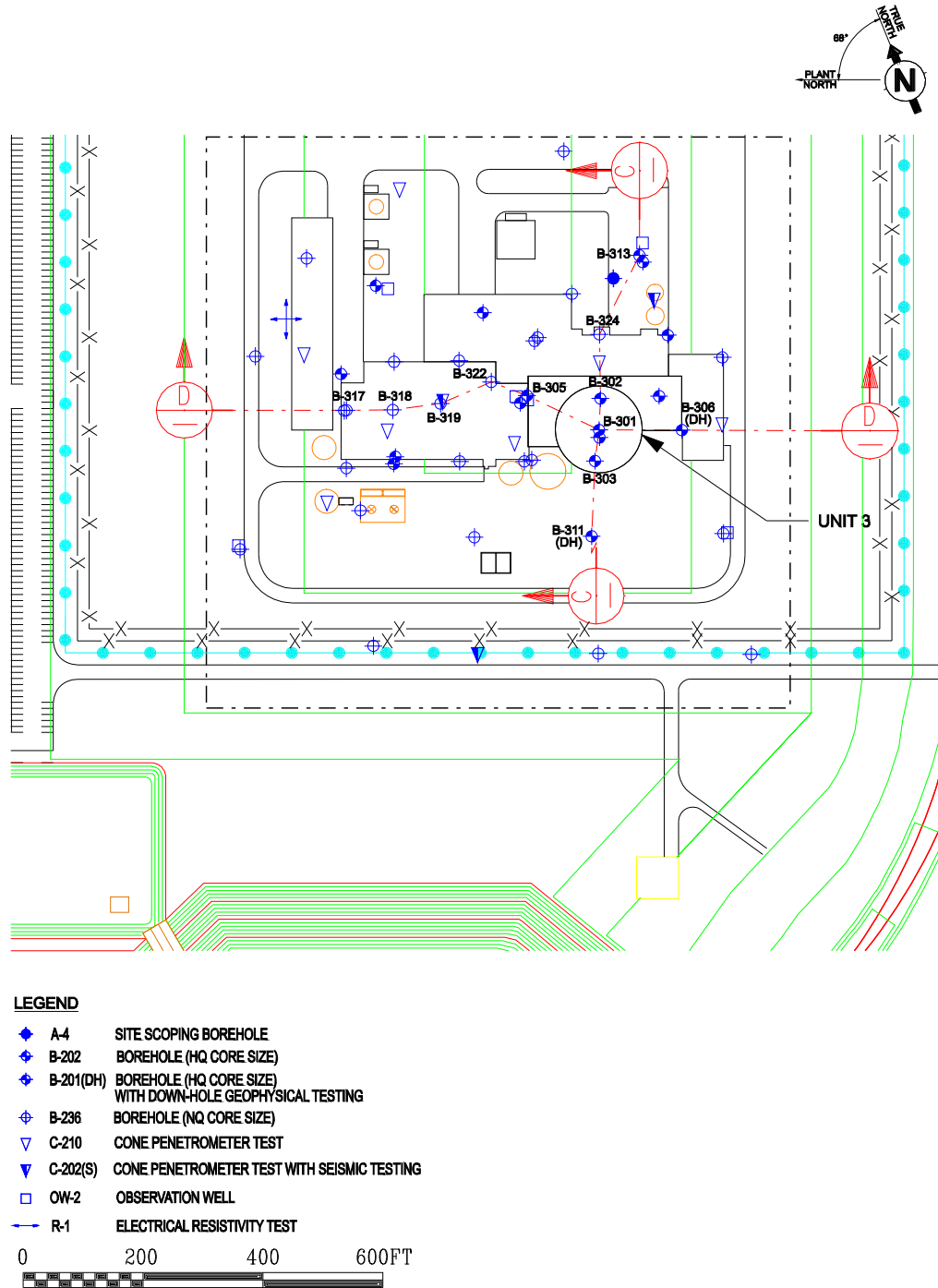
Figure 2.5.4-219. Profile Location Map Showing Excavation Geometry Unit 3 (Sheet 2 of 2)
