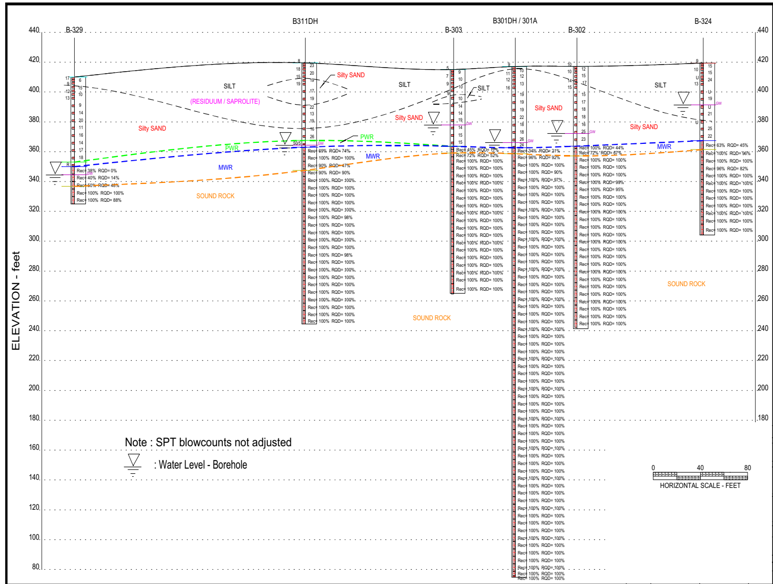
Figure 2.5.4-207. Inferred Subsurface Profiles Unit 3 North-South: J-J (Sheet 2 of 3)
