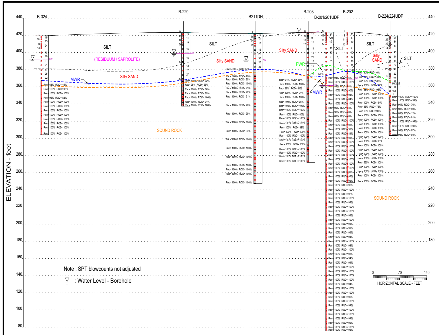
Figure 2.5.4-205. Inferred Subsurface Profiles Unit 2 North-South: F-F (Sheet 2 of 4)
