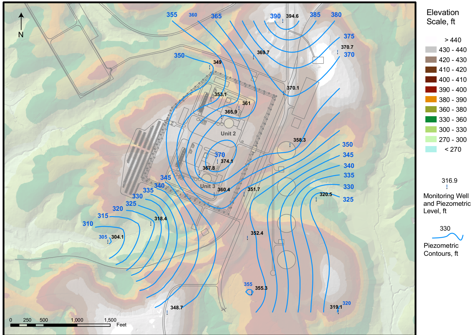
Figure 2.5.4-237. Piezometric Level Contours, 4th Quarter, March 2007 — Units 2 and 3
