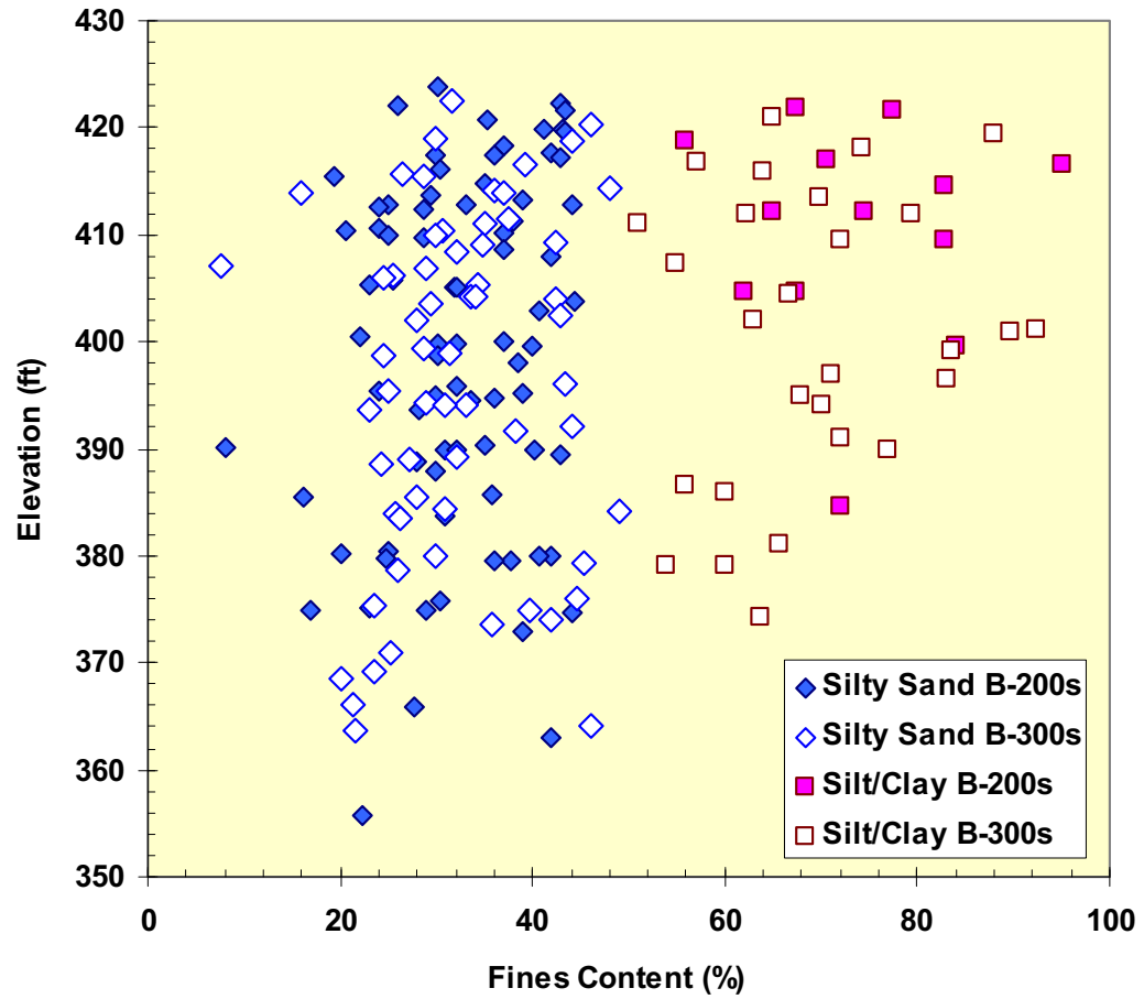
Figure 2.5.4-215. Fines Content
