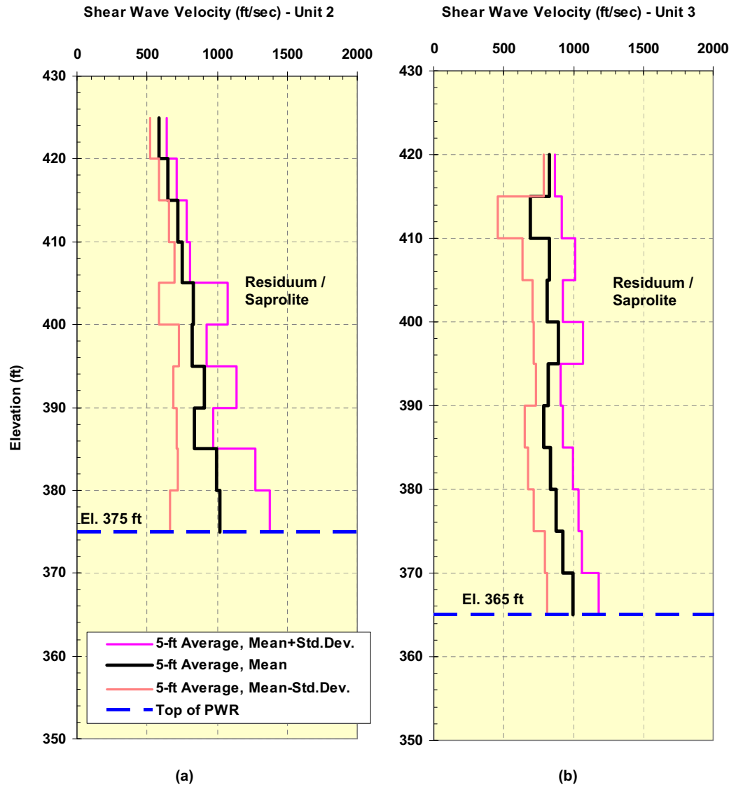
Figure 2.5.4-229. Shear Wave Velocity of Layers I and II with 5-Foot Vertical Distance Averaging
