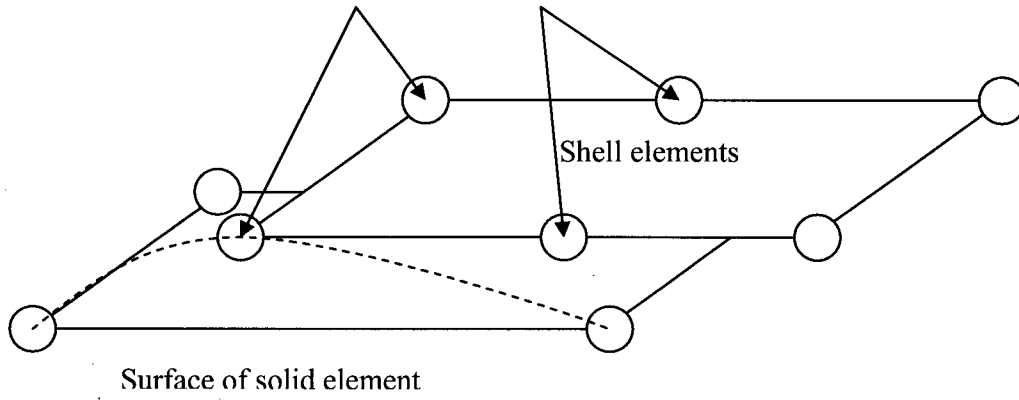
Figure 6a. Face-to-face shell to solid connection.
