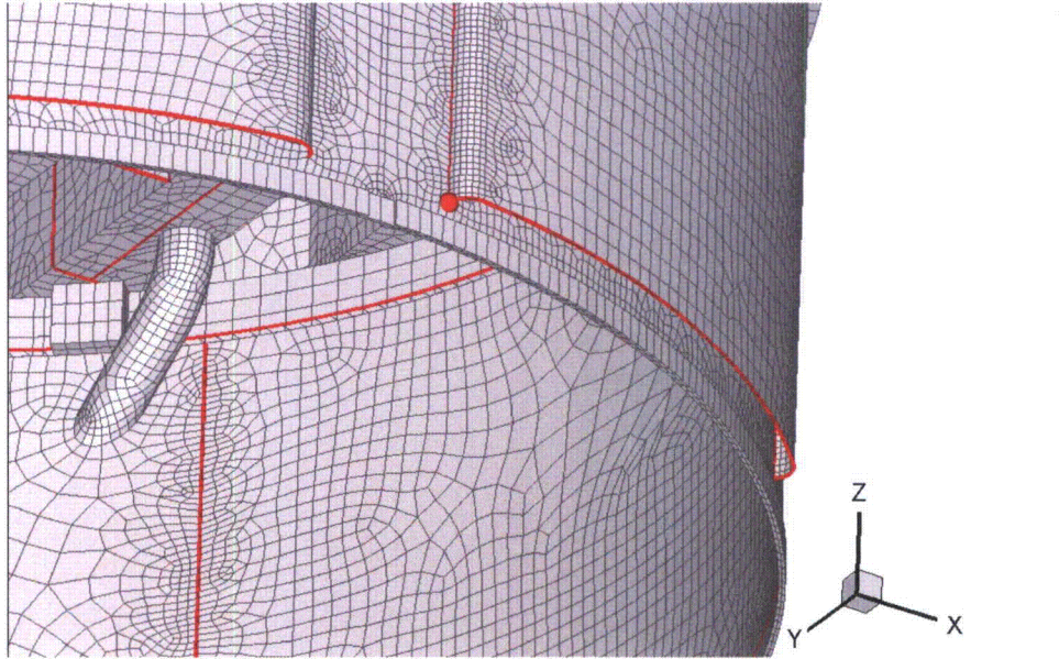
Figure 11a. Location of node on drain channel/skirt weld analyzed with sub-model in [26].
