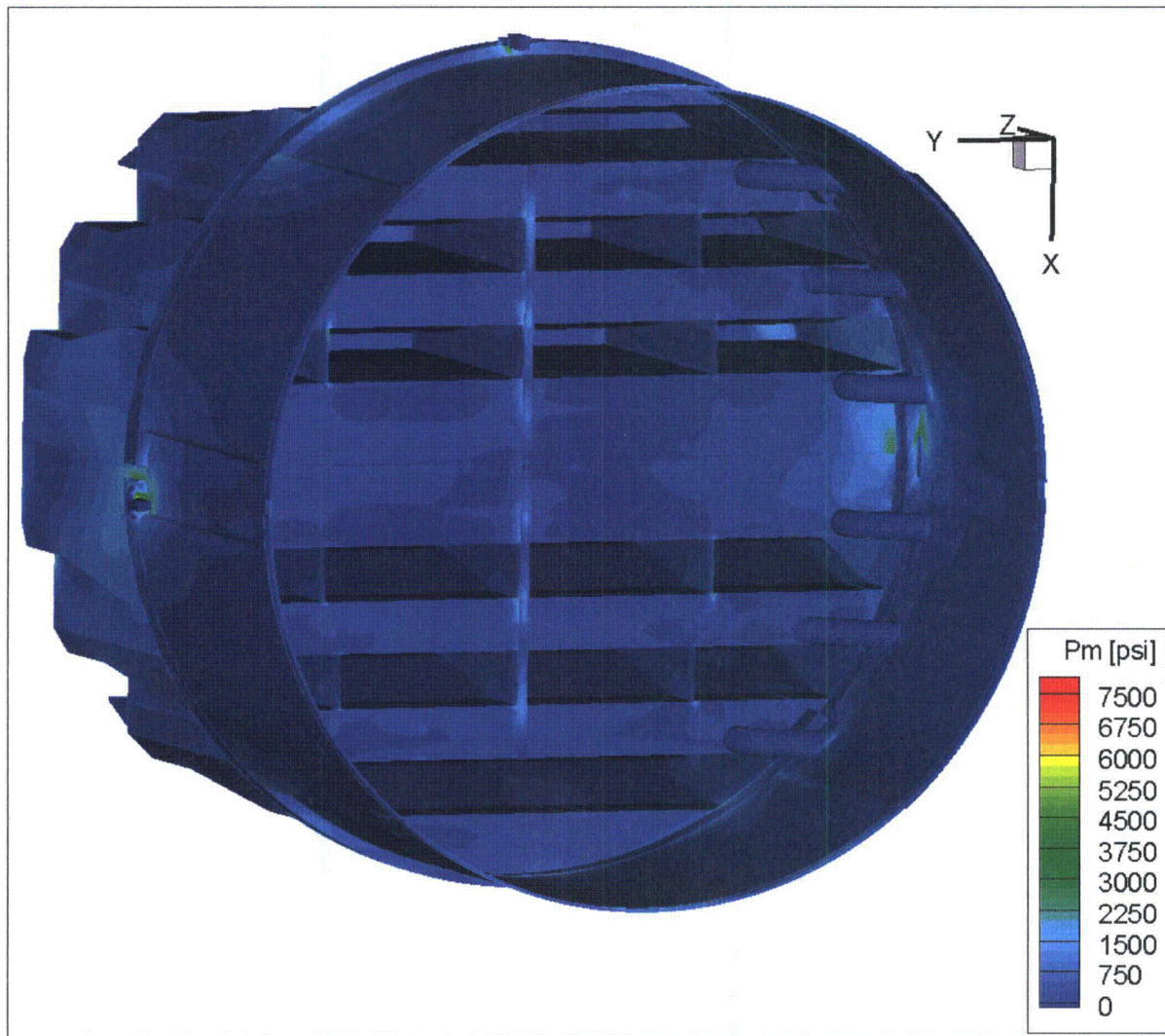
Figure 12b. Contour plot of maximum membrane stress intensity, P_m , for CLTP load. Second view from below.
