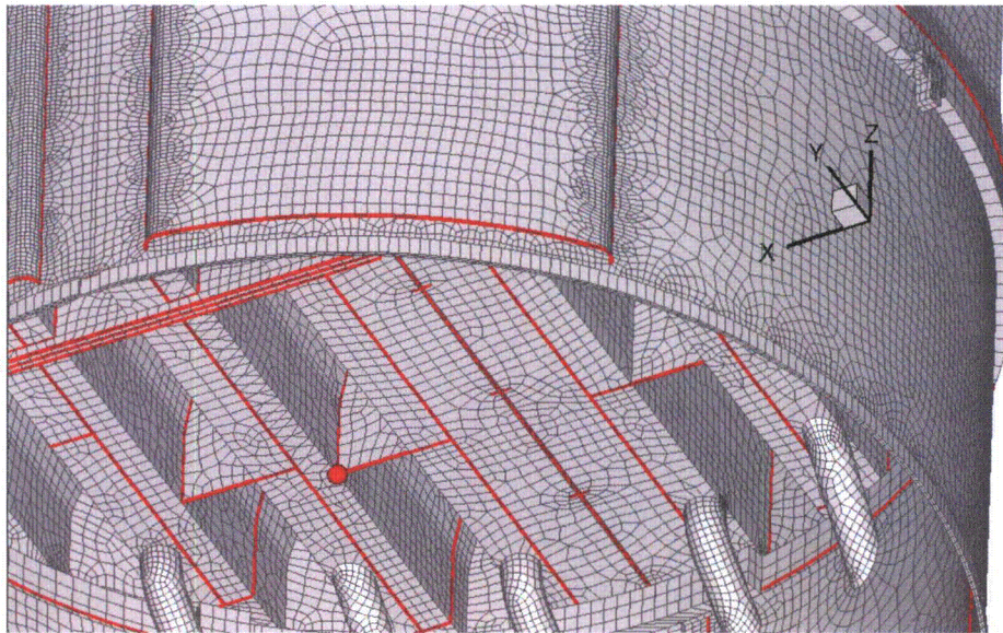
Figure 11b. Location of node on inner hood/hood support/middle base plate weld analyzed with sub-model in [26].
