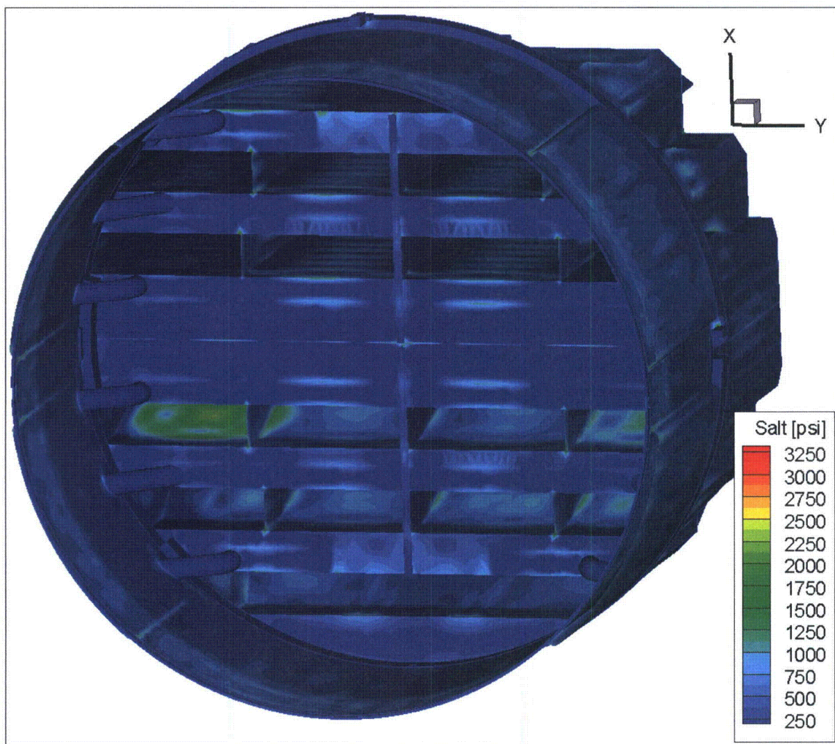
Figure 13g. Contour plot of alternating stress intensity, S_{alt} , for CLTP operation with frequency shifts. The recorded stress at a node is the maximum value taken over all frequency shifts. Third view from below.
