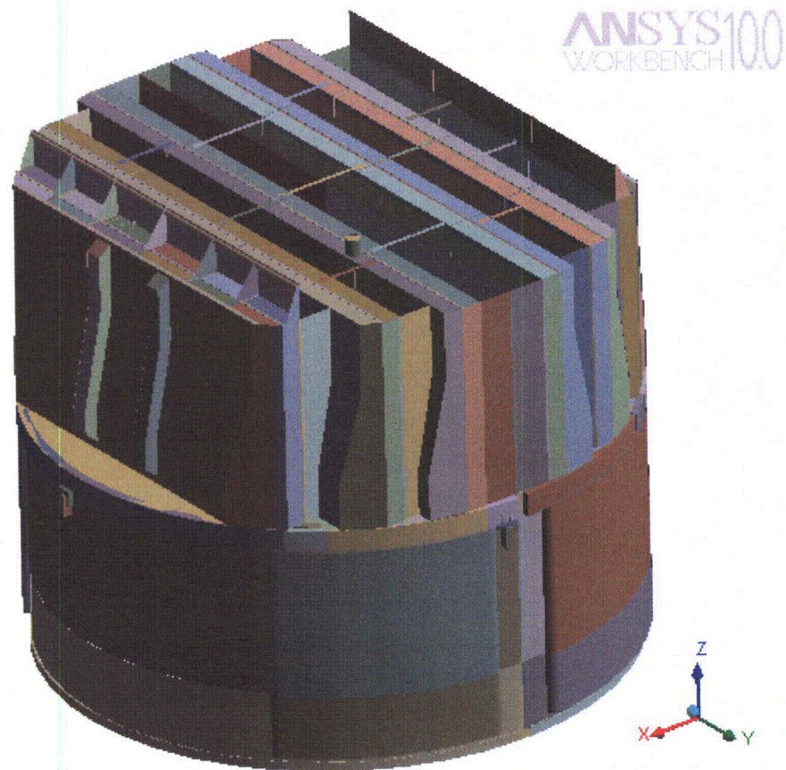
Figure 1. Overall geometry of the Browns Ferry Unit 2 steam dryer model.
