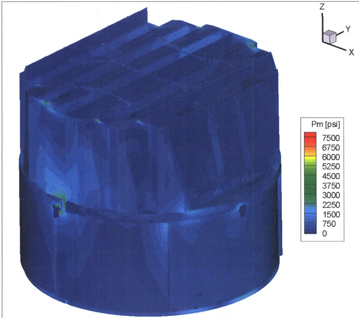
Figure 12a. Contour plot of maximum membrane stress intensity, P_m , for CLTP load. The maximum stress intensity is 7635 psi. First view.
