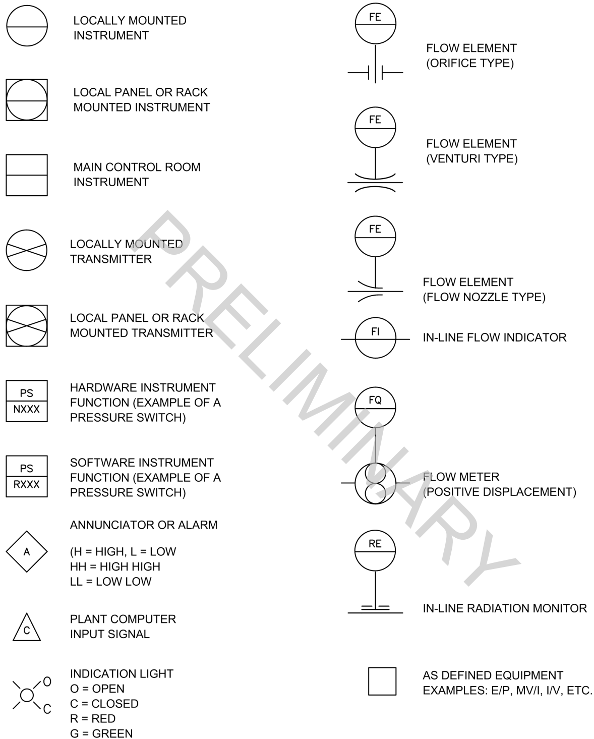
Figure 1.7-2. P&amp;ID Symbols for Instruments
