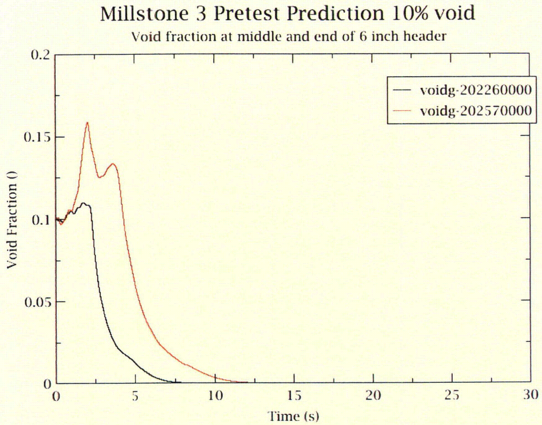
Figure A-3 Void fractions in 6 inch header 10% void case.
