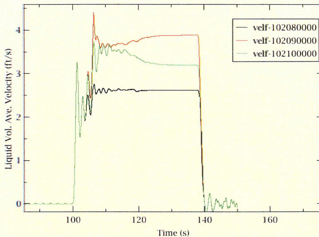
Figure 3-8 Test Case 12 fluid velocity near charging line elbow.
