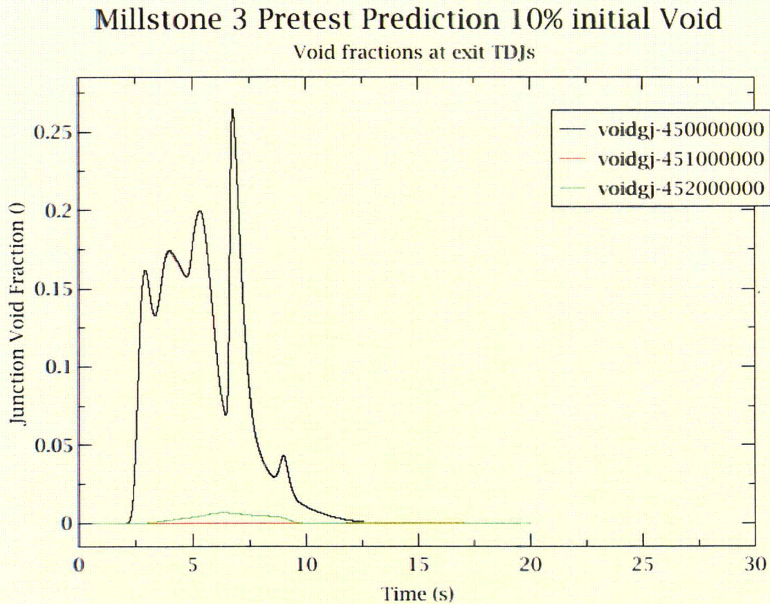
Figure A-4 Void fractions exiting the time dependent junctions – 10% initial void case.
