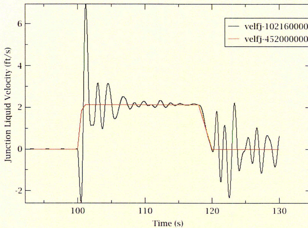
Figure 3-2 Case 1 charging flow velocity.
