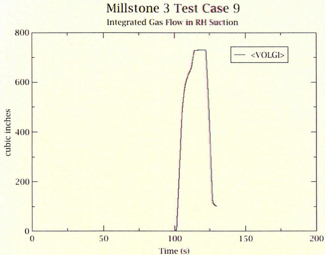
Figure 3-4 Case 9 RH line gas transport.
