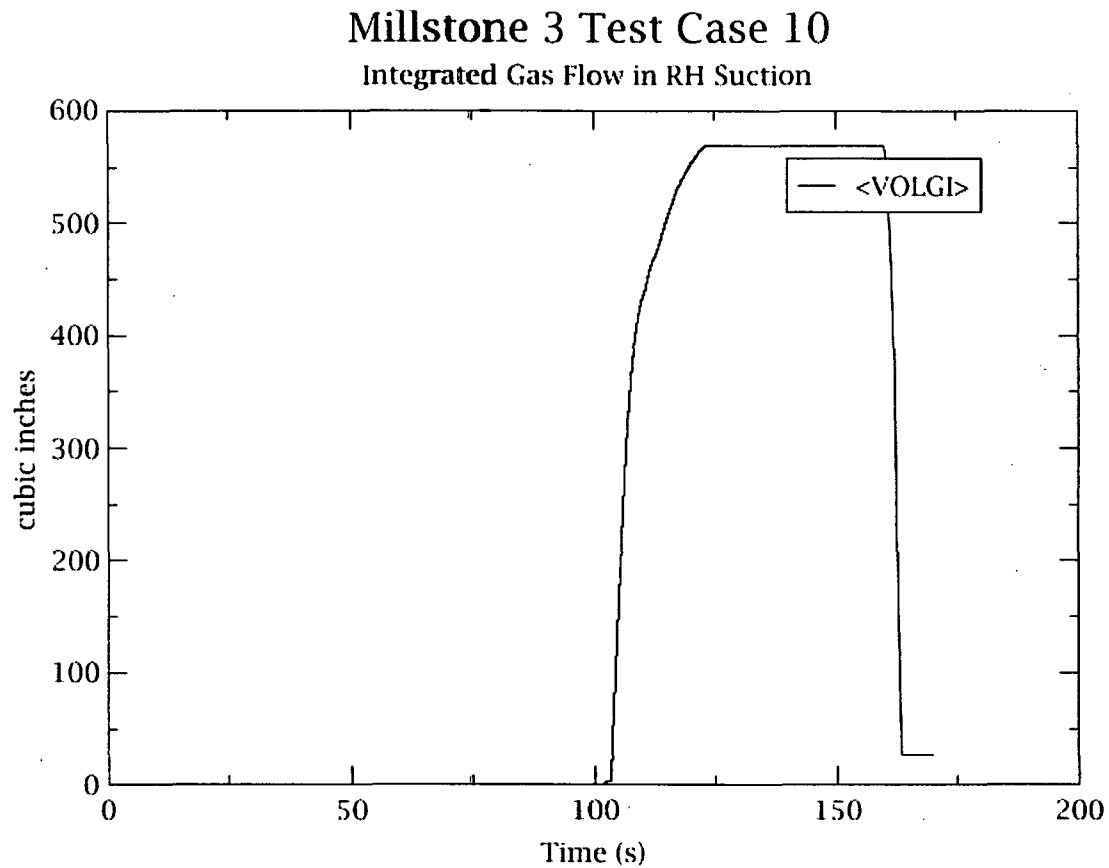
Figure 3-5 Case 10 RH line gas transport.
