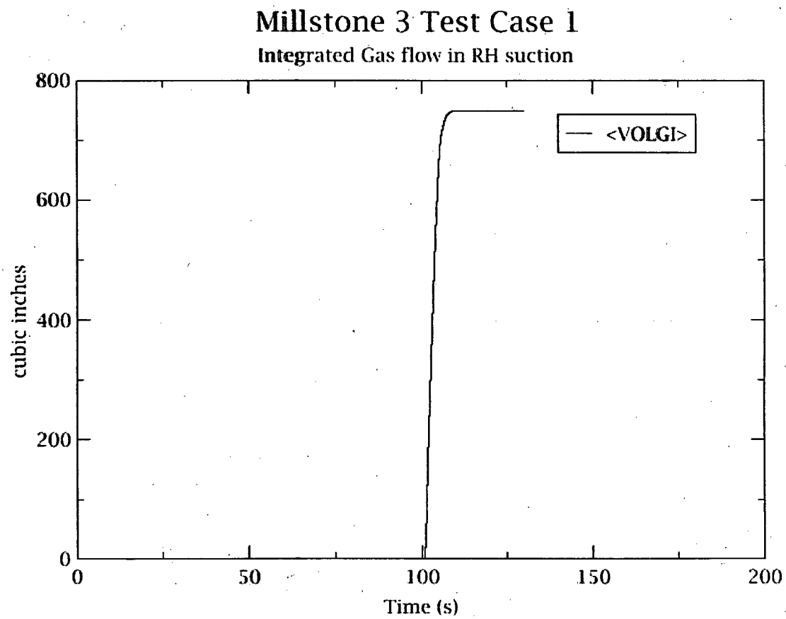
Figure 3-3 Case 1 RH line gas transport.
