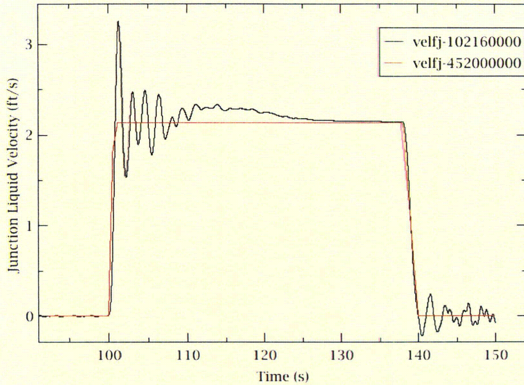
Figure 3-6 Test Case 12 charging line velocity.
