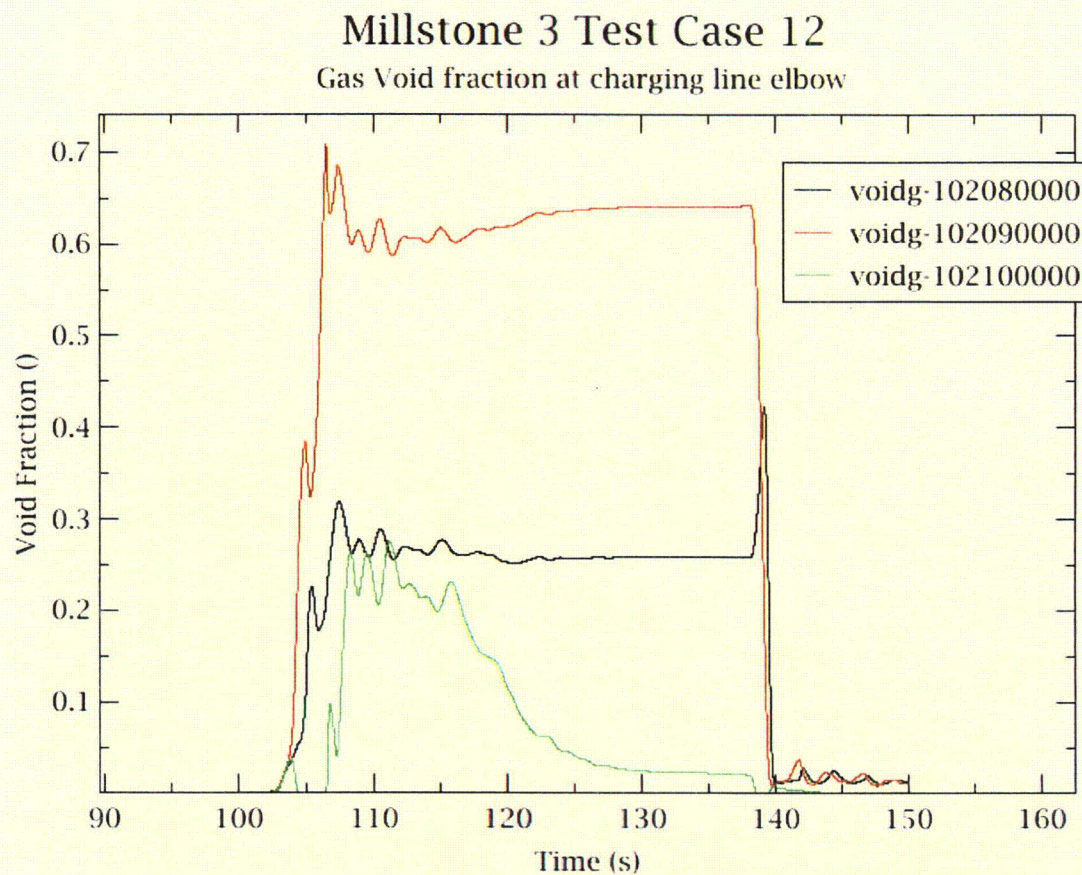
Figure 3-7 Test Case 12 gas void fraction near charging line elbow.
