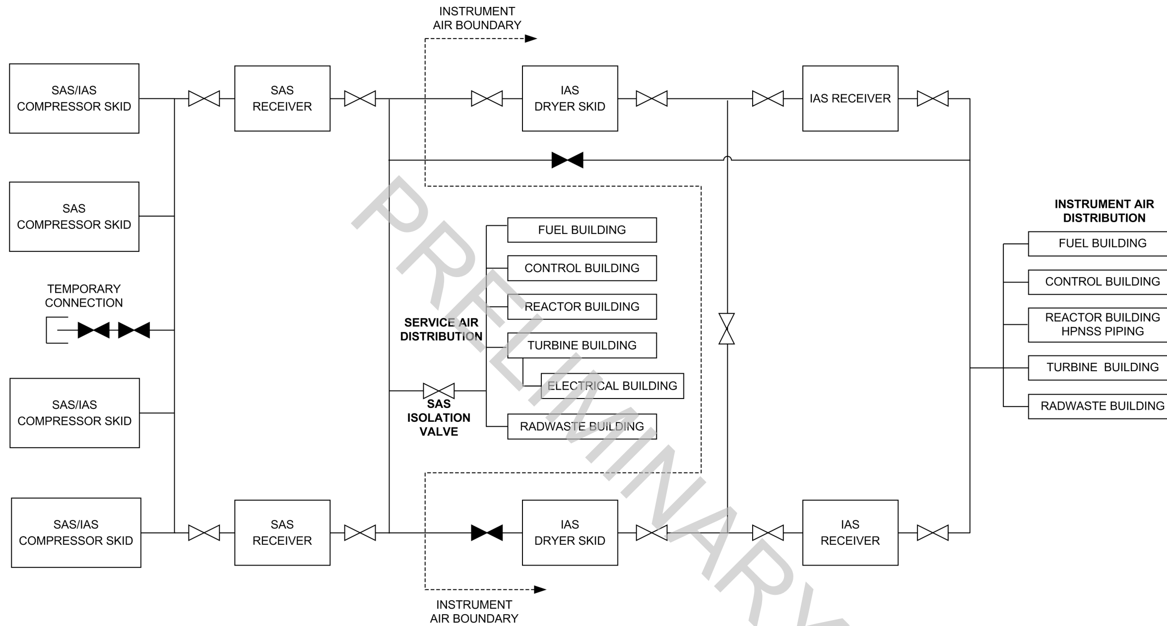
Figure 9.3-3. Service Air and Instrument Air System Simplified Diagram
