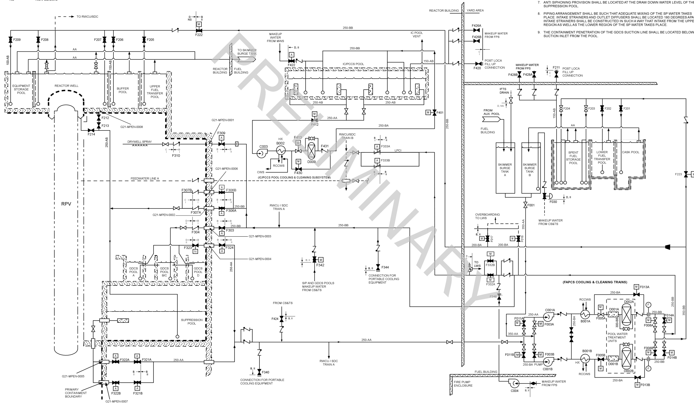
Figure 9.1-1. FAPCS Schematic Diagram
