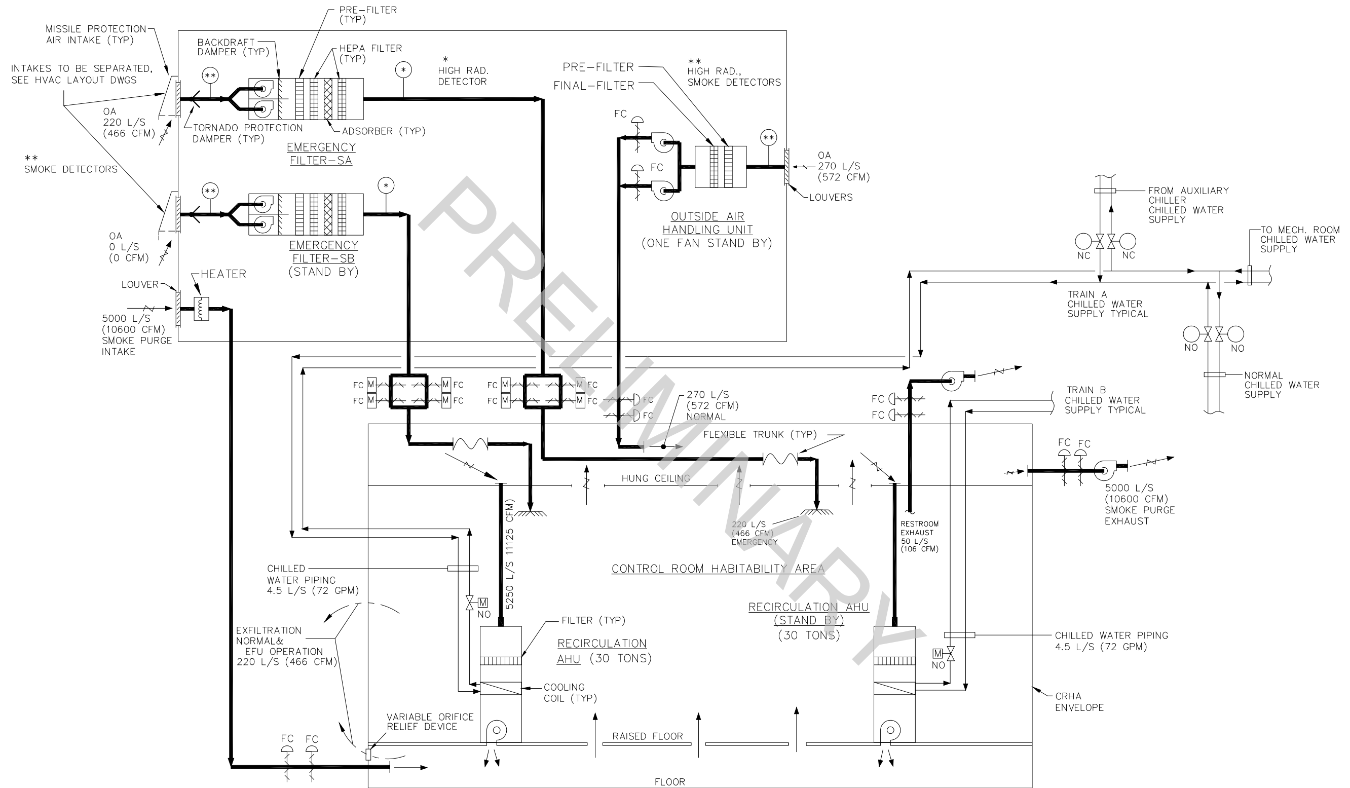
Figure 9.4-1. CRHAVS Simplified System Diagram
