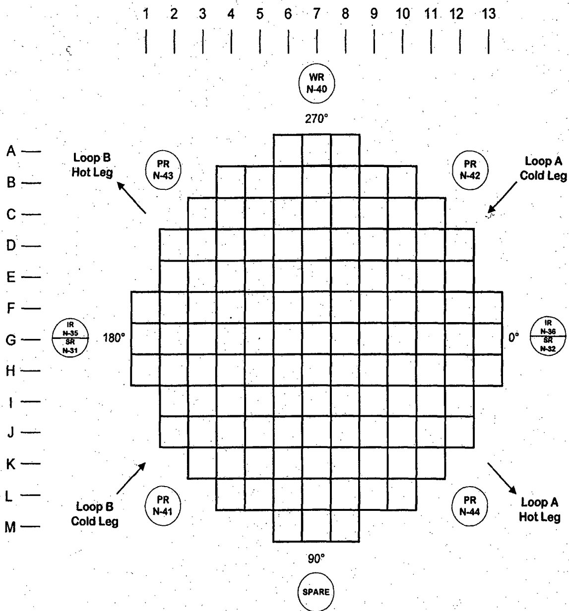
Figure 7.6-3 EX-CORE DETECTOR LOCATIONS RELATIVE TO CORE
