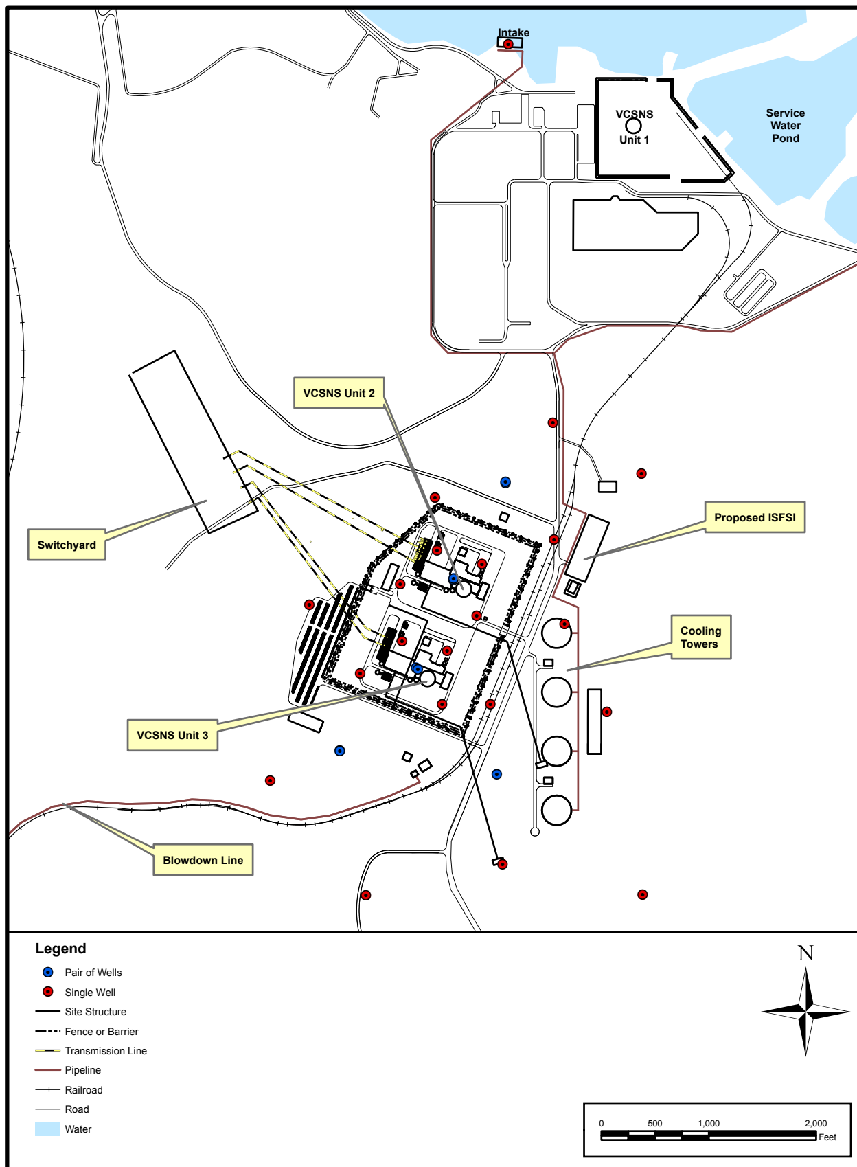
Figure 6.3-1 Observation Wells
