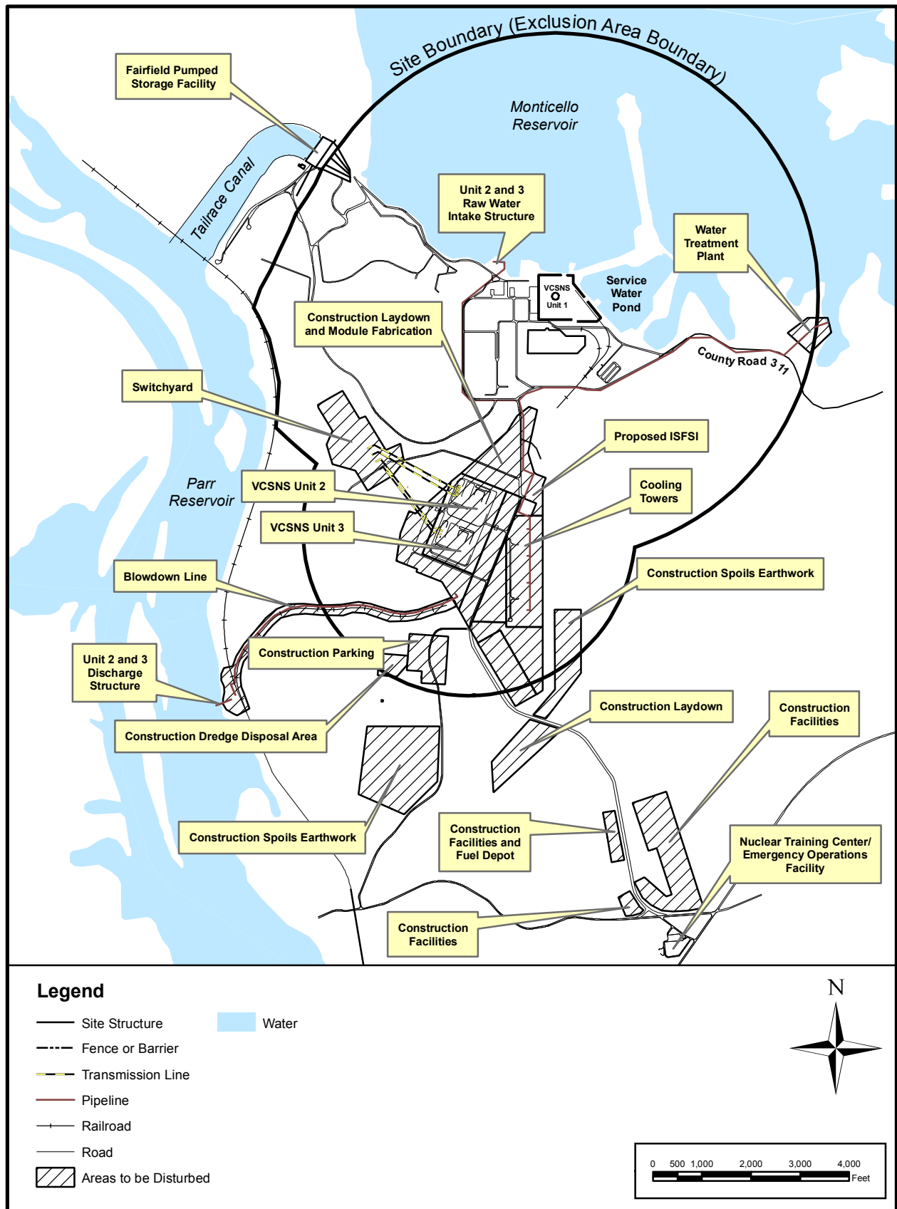
Figure 2.1-1 VCSNS Site and Proposed Plant Footprint
