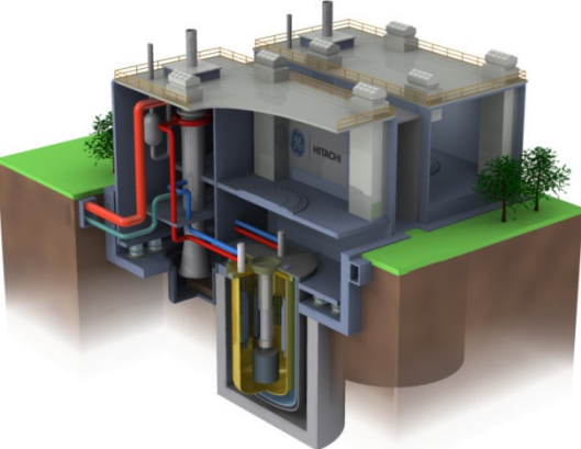
PRISM reactor vessel
