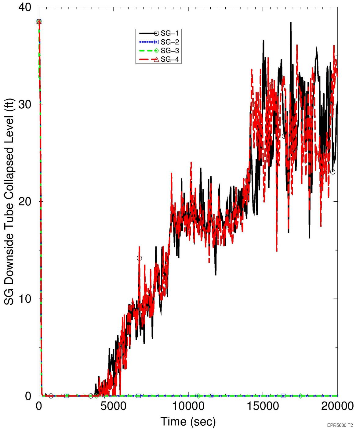
Figure 15.6-85—SBLOCA - 6 inch Break - Steam Generator Downside Collapsed Liquid Level
