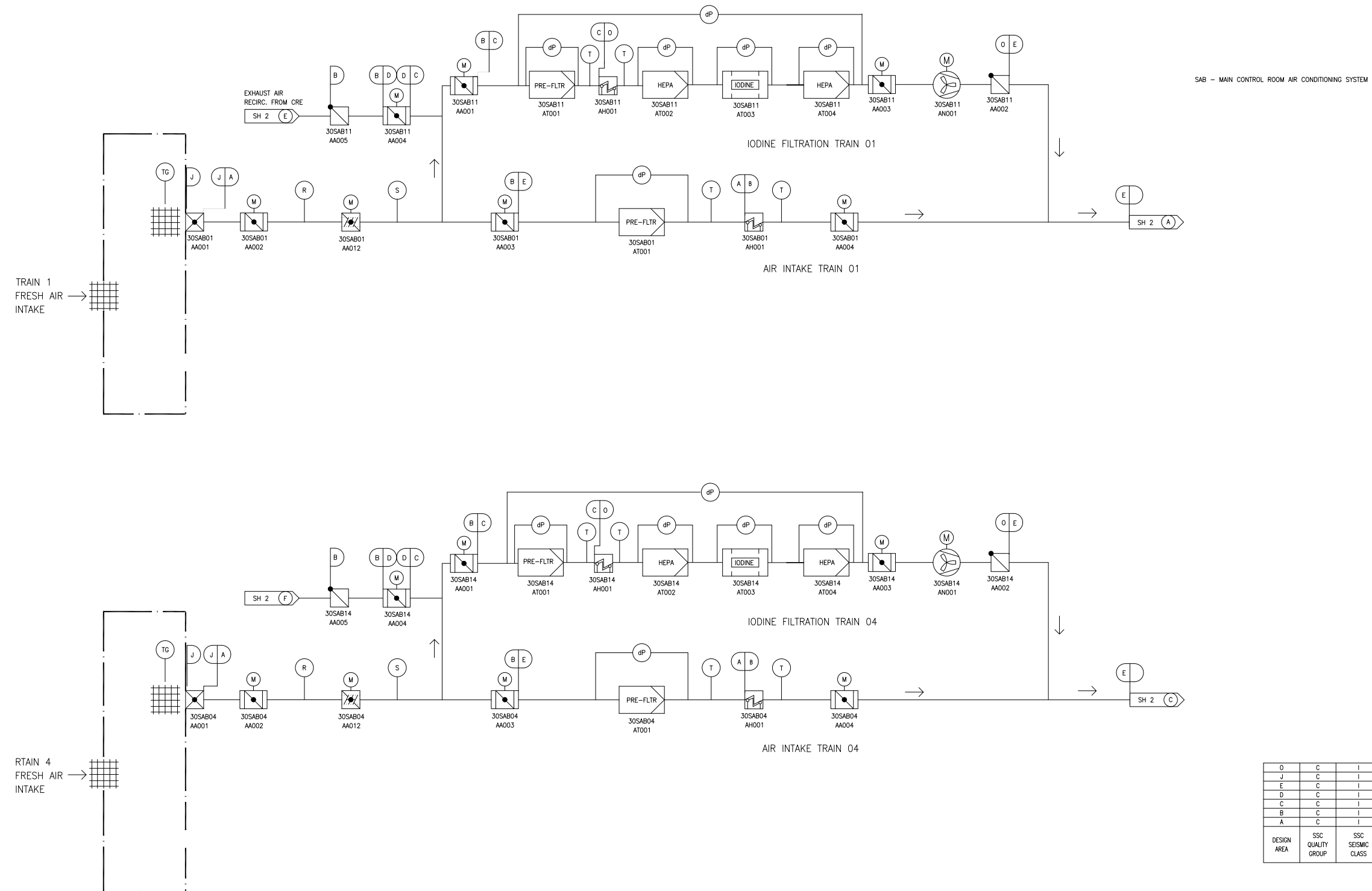
Figure 9.4.1-1—Control Room Air Intake and Iodine Filtration Train Subsystems
