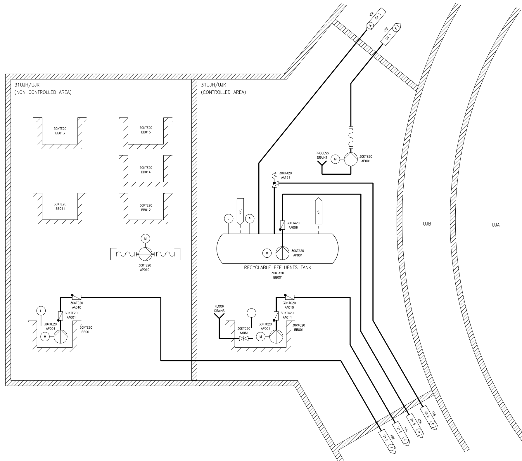
Figure 9.3.3-1—Nuclear Island Drain and Vent System Sheet 2 of 8
