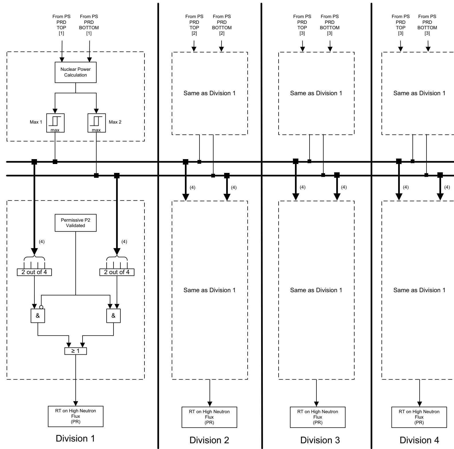
Figure 7.8-1—Reactor Trip on Excore High Neutron Flux
