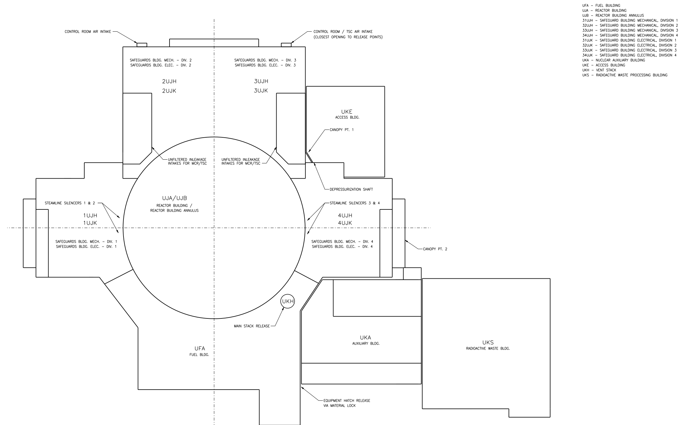
Figure 2.3-1—U.S. EPR Release Points and Control Room Air Intakes
