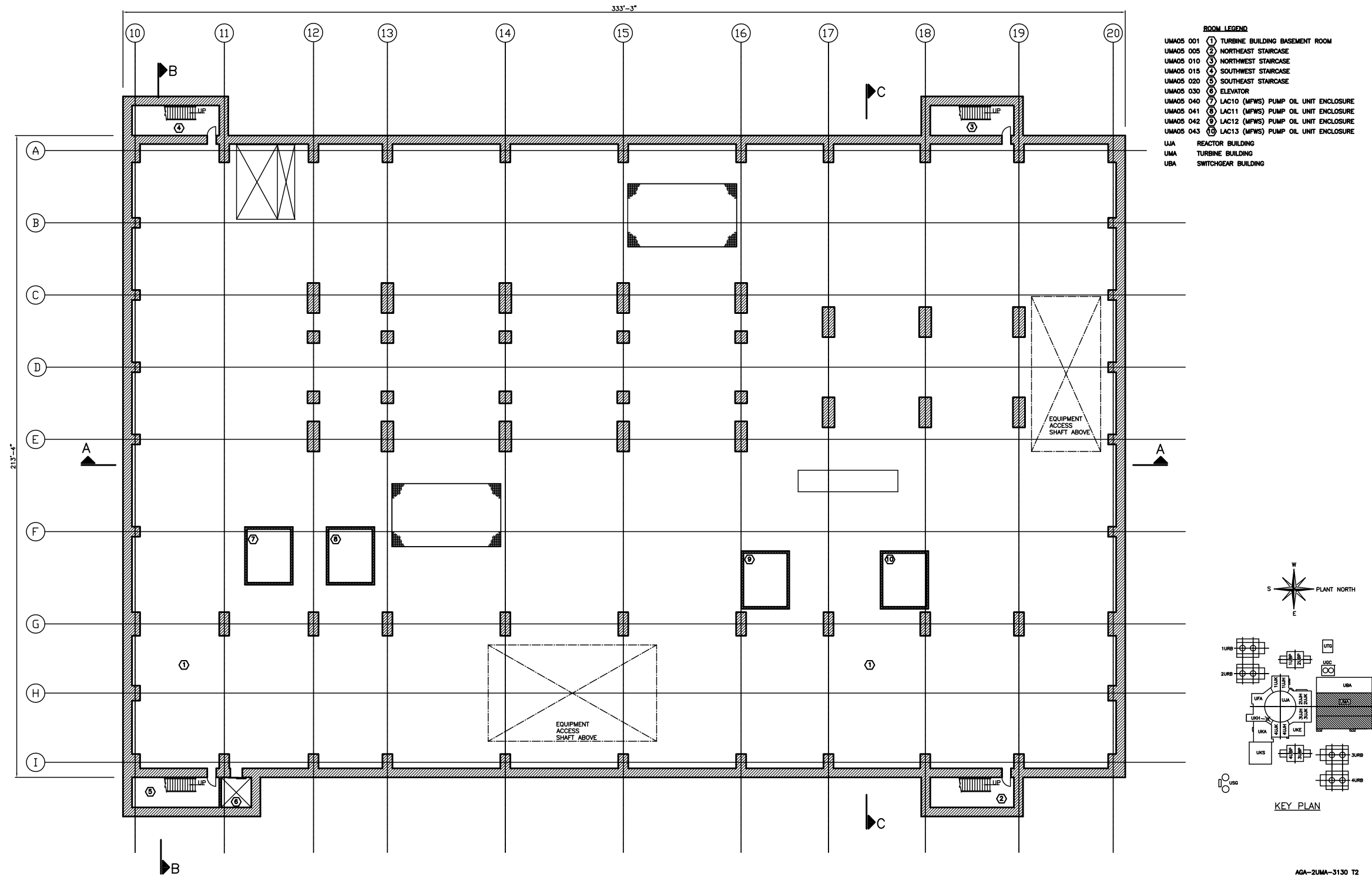
Figure 1.2-30—[[ Turbine Building General Arrangement Plan View Elevation -23'-0" ]]
