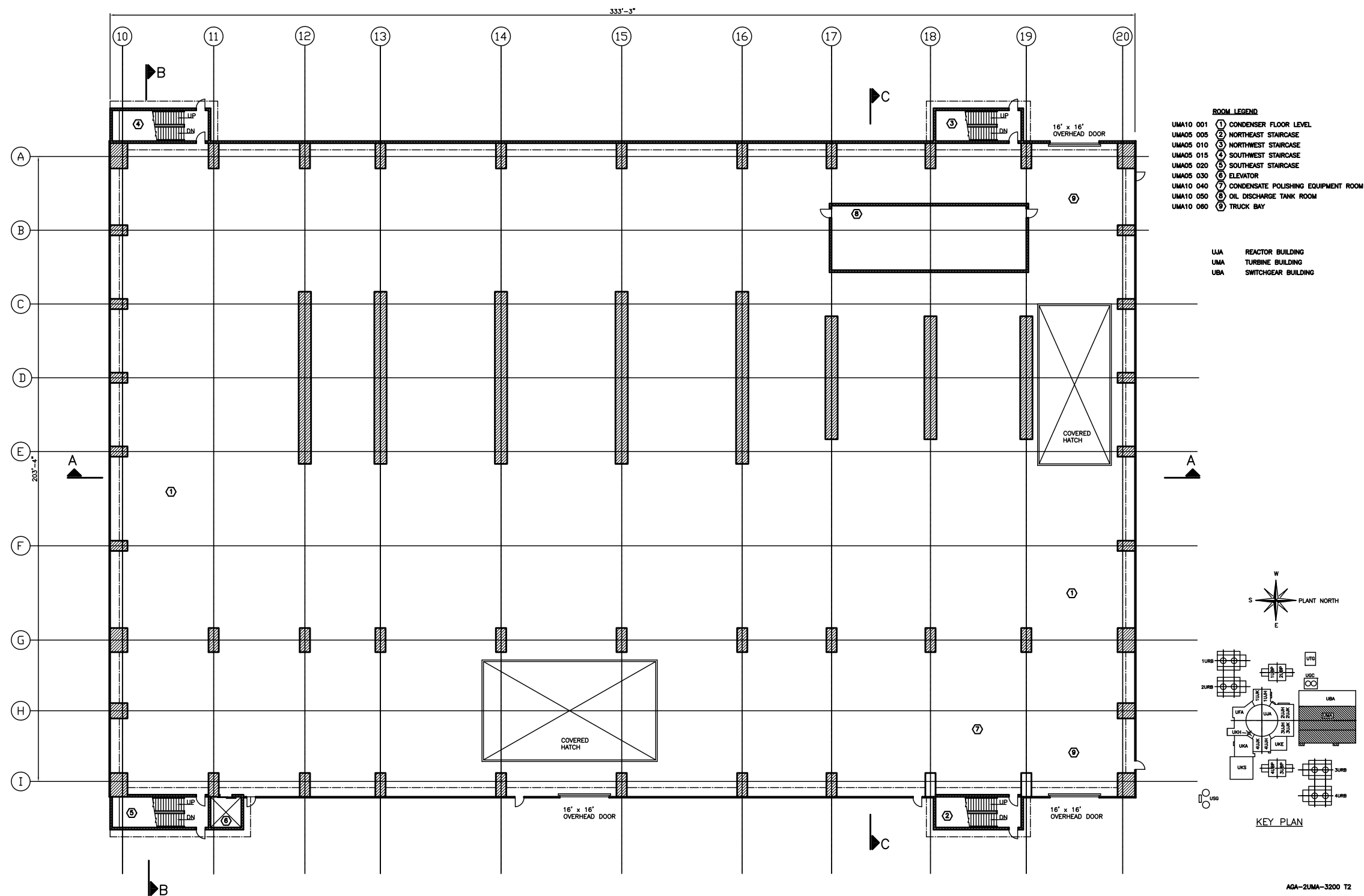
Figure 1.2-32—[[ Turbine Building General Arrangement Plan View Elevation +0'-0" ]]
