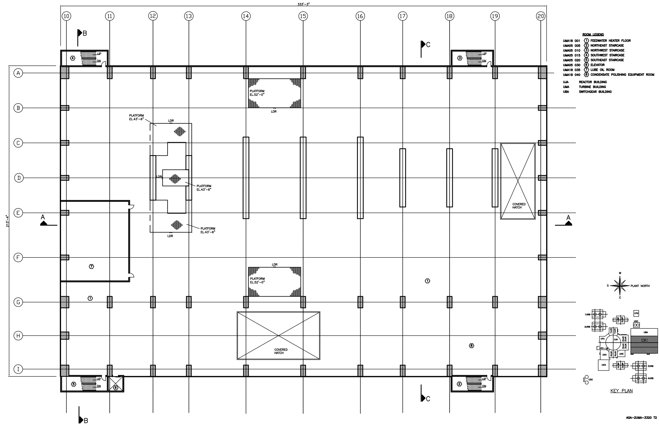
Figure 1.2-34—[[ Turbine Building General Arrangement Plan View Elevation +38'-0" ]]
