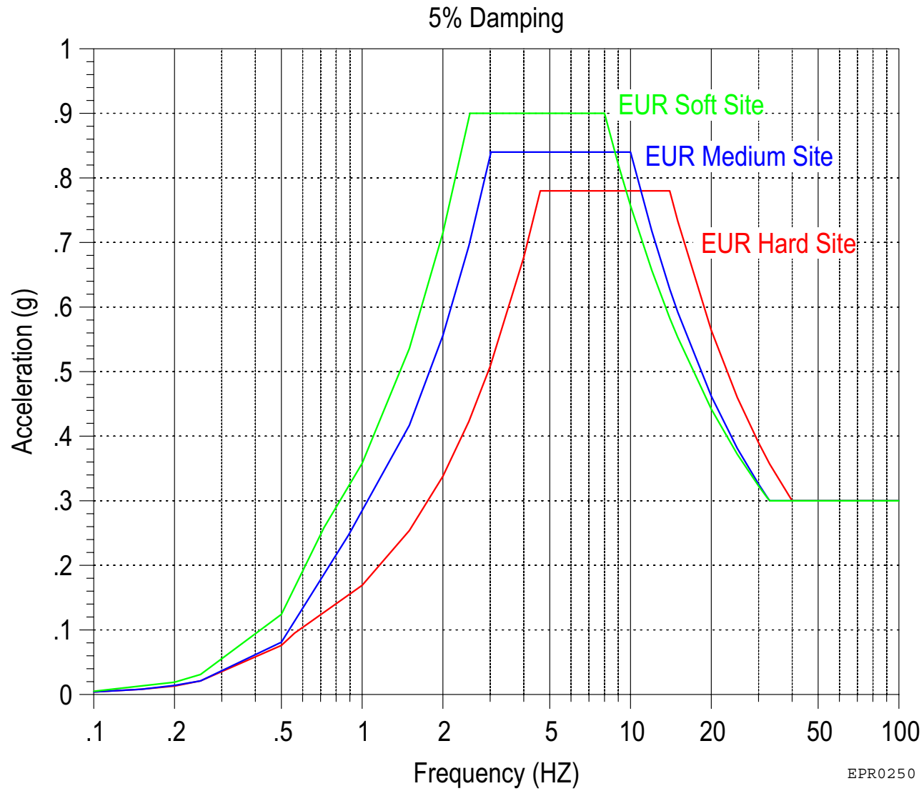
Figure 5.0-1—Design Response Spectra for EUR Control Motions (Hard, Medium and Soft Sites)
