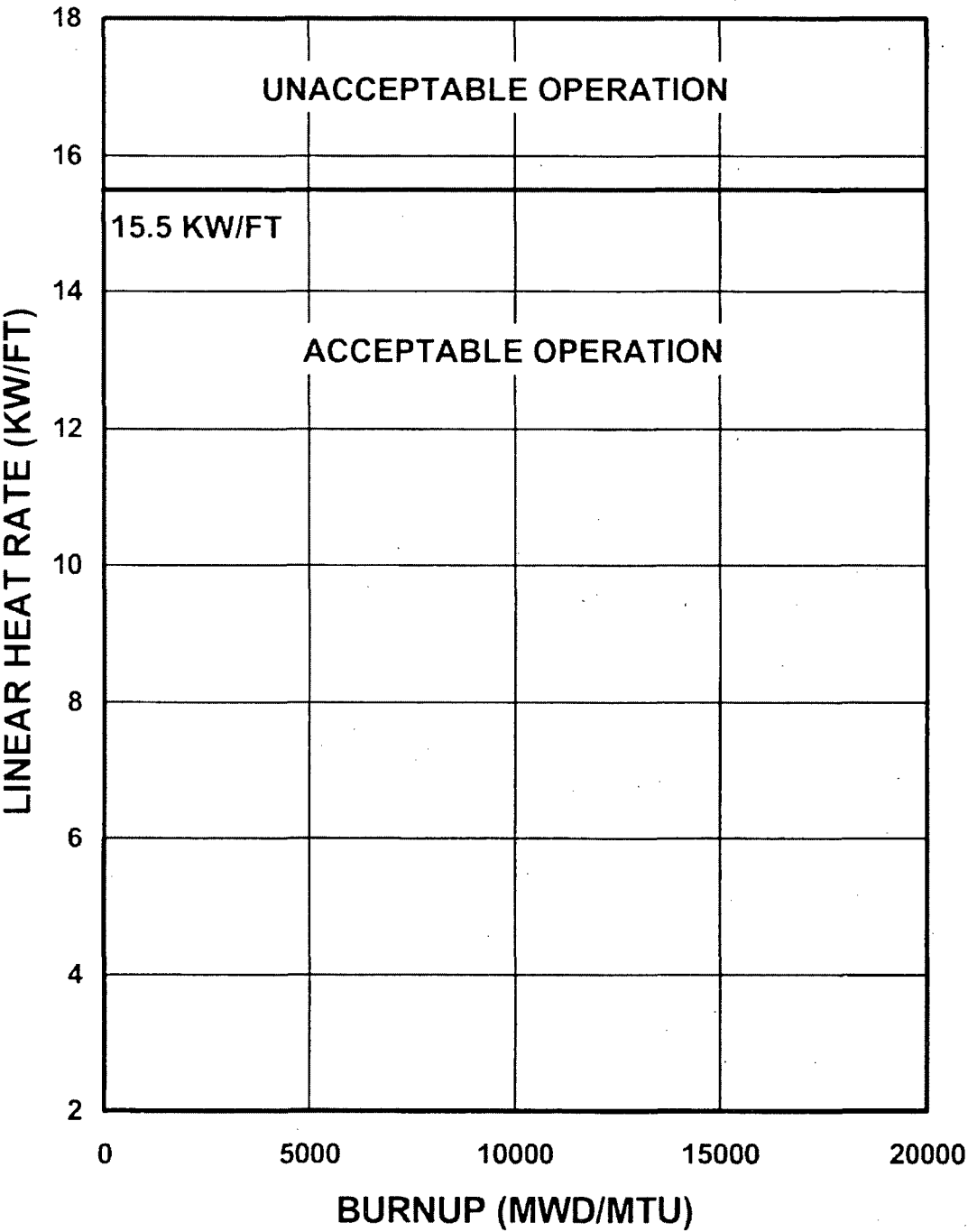
COLR ALLOWABLE PEAK LINEAR HEAT RATE VS. BURNUP FIGURE 3
