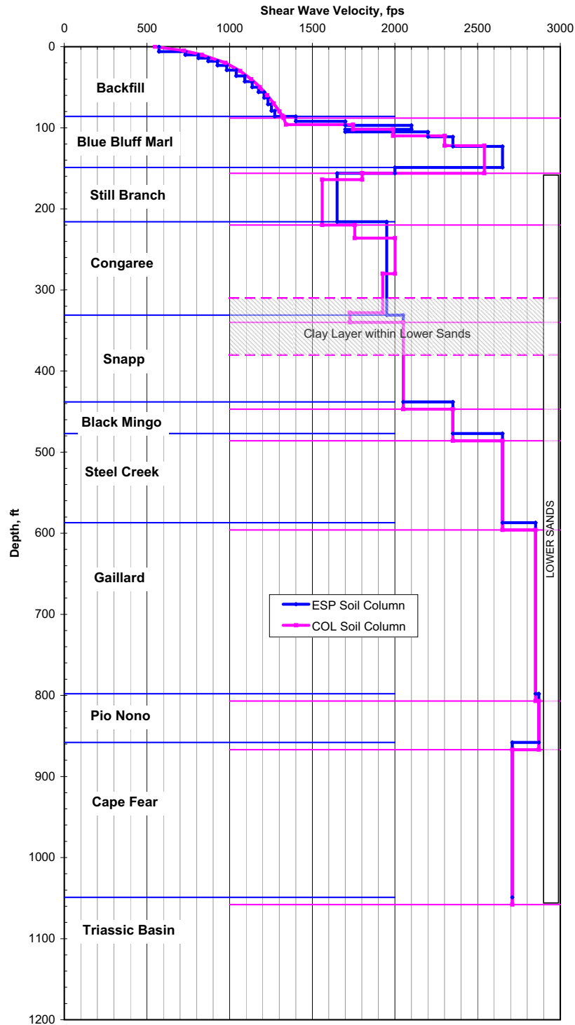
Figure 2.5.4-7a Shear Wave Velocity Profile — ESP and COL Soil Columns
