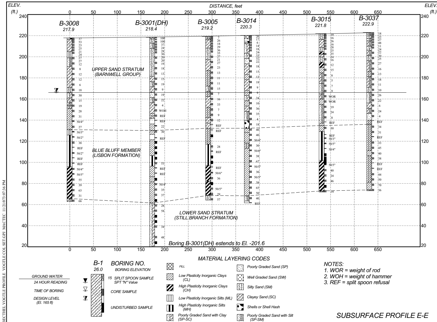
Figure 2.5.4-5a Subsurface Profile E-E'
