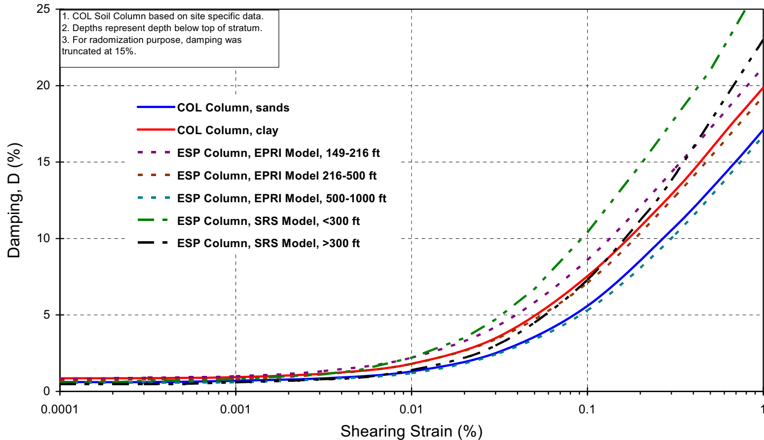
Figure 2.5.4-20c. Comparison of Damping Curves - Lower Sands
