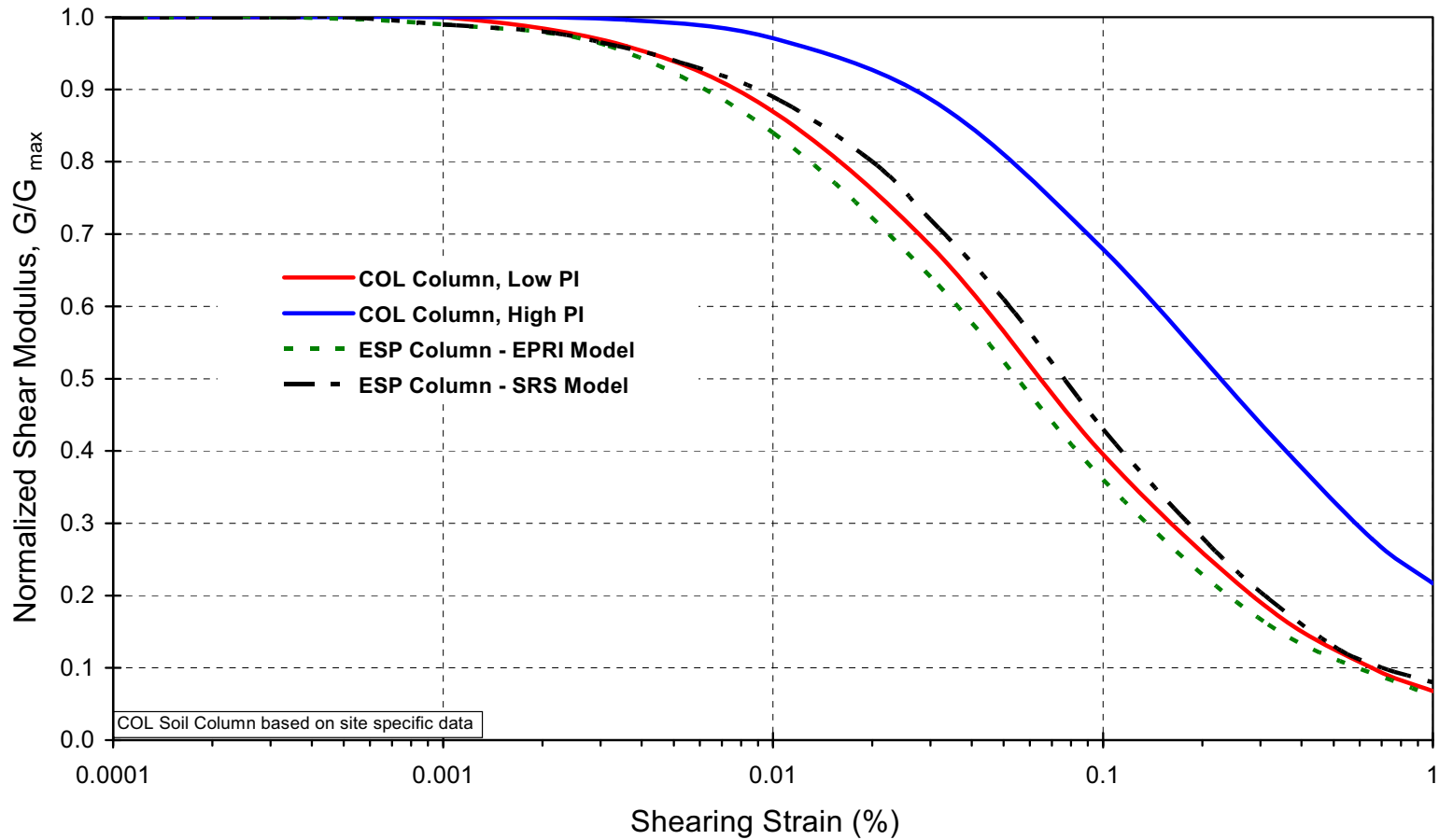
Figure 2.5.4-19b Comparison of Shear Modulus Reduction Curves - Blue Bluff Marl
