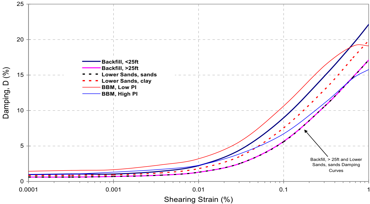
Figure 2.5.4-11a Site-Specific Damping Ratio Curves
