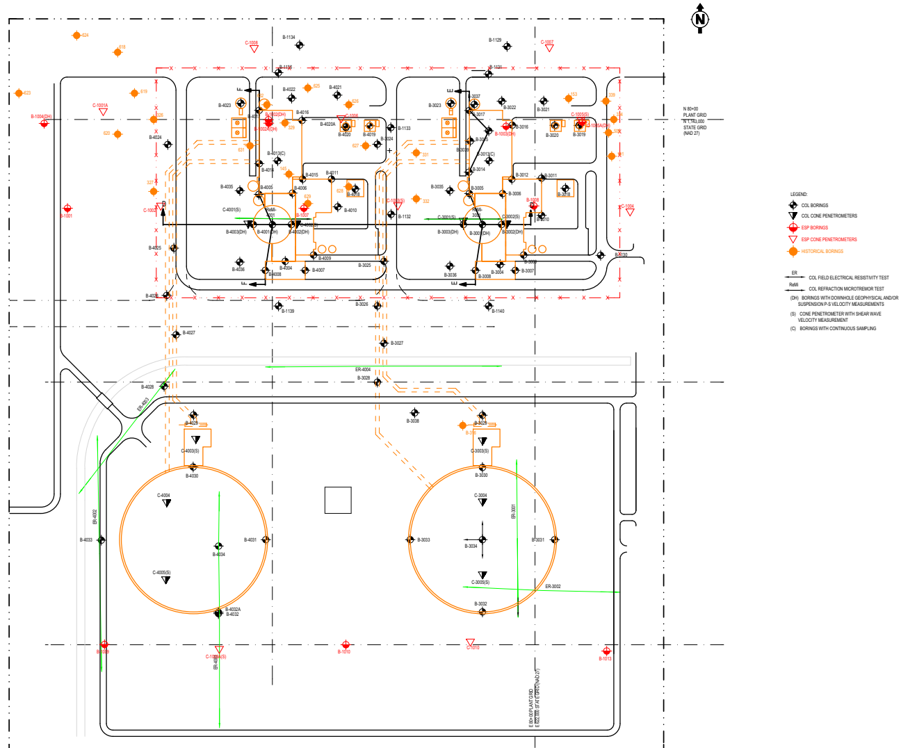
Figure 2.5.4-1b COL Power Block — Cooling Tower Boring Location
