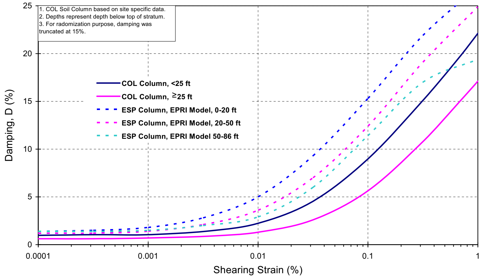
Figure 2.5.4-20a Comparison of Damping Ratio Curves - Backfill Soils
