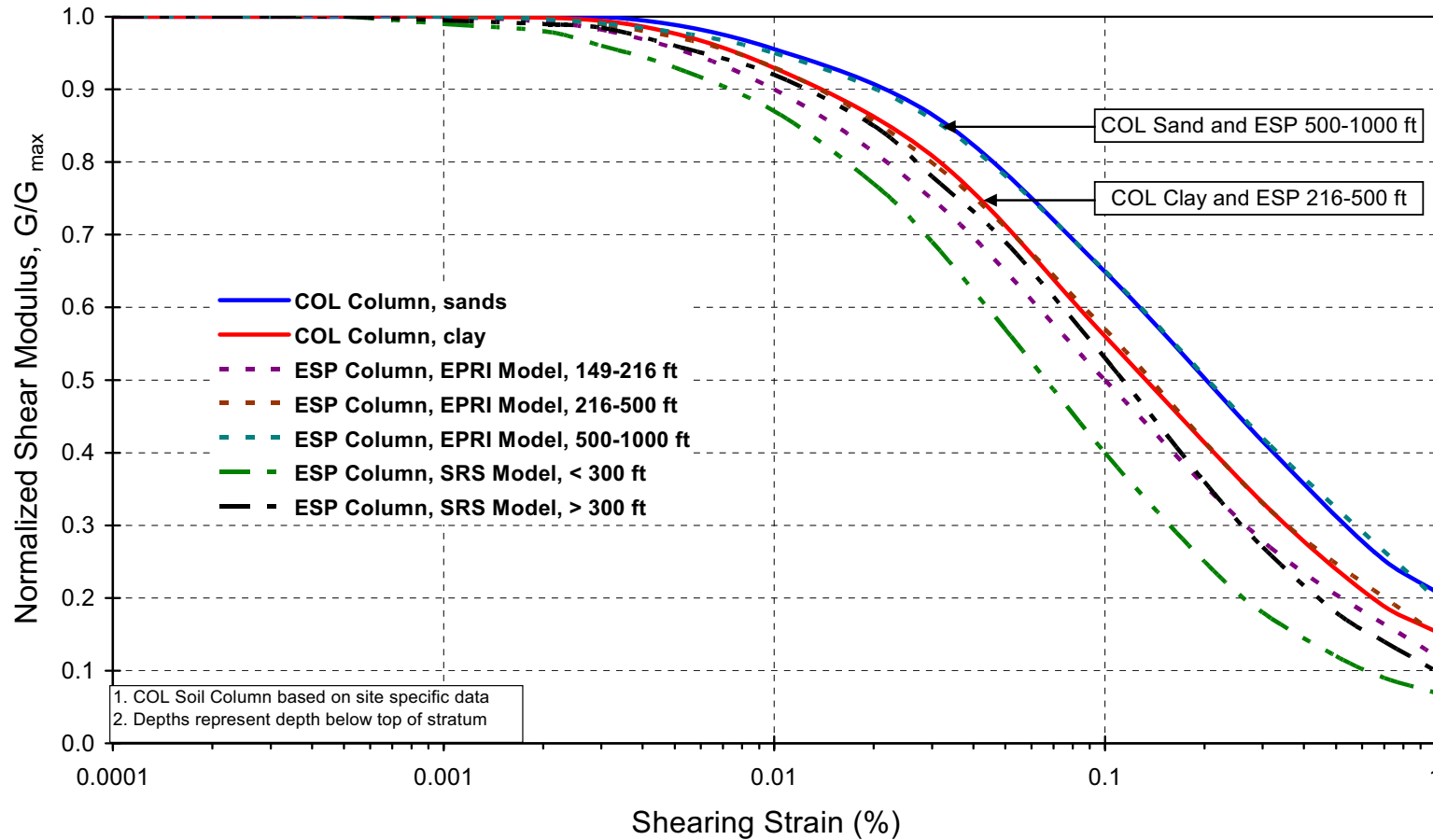
Figure 2.5.4-19c Comparison of Shear Modulus Reduction Curves - Lower Sands
