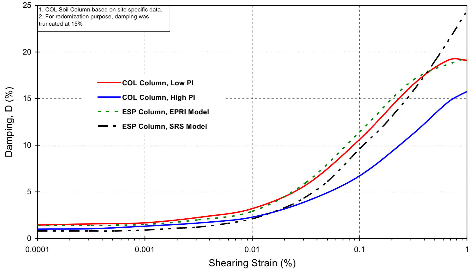
Figure 2.5.4-20b Comparison of Damping Ratio Curves - Blue Bluff Marl
