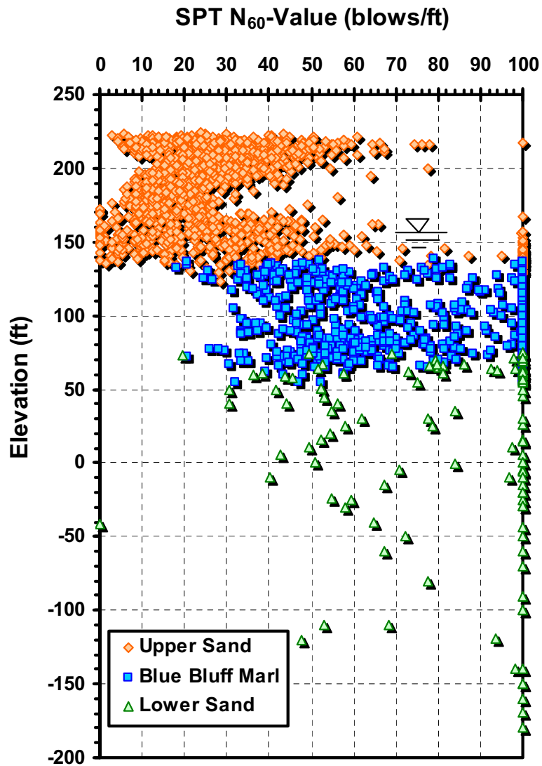
Figure 2.5.4-18 Distribution of SPT N 60 -Value with Elevation (COL)
