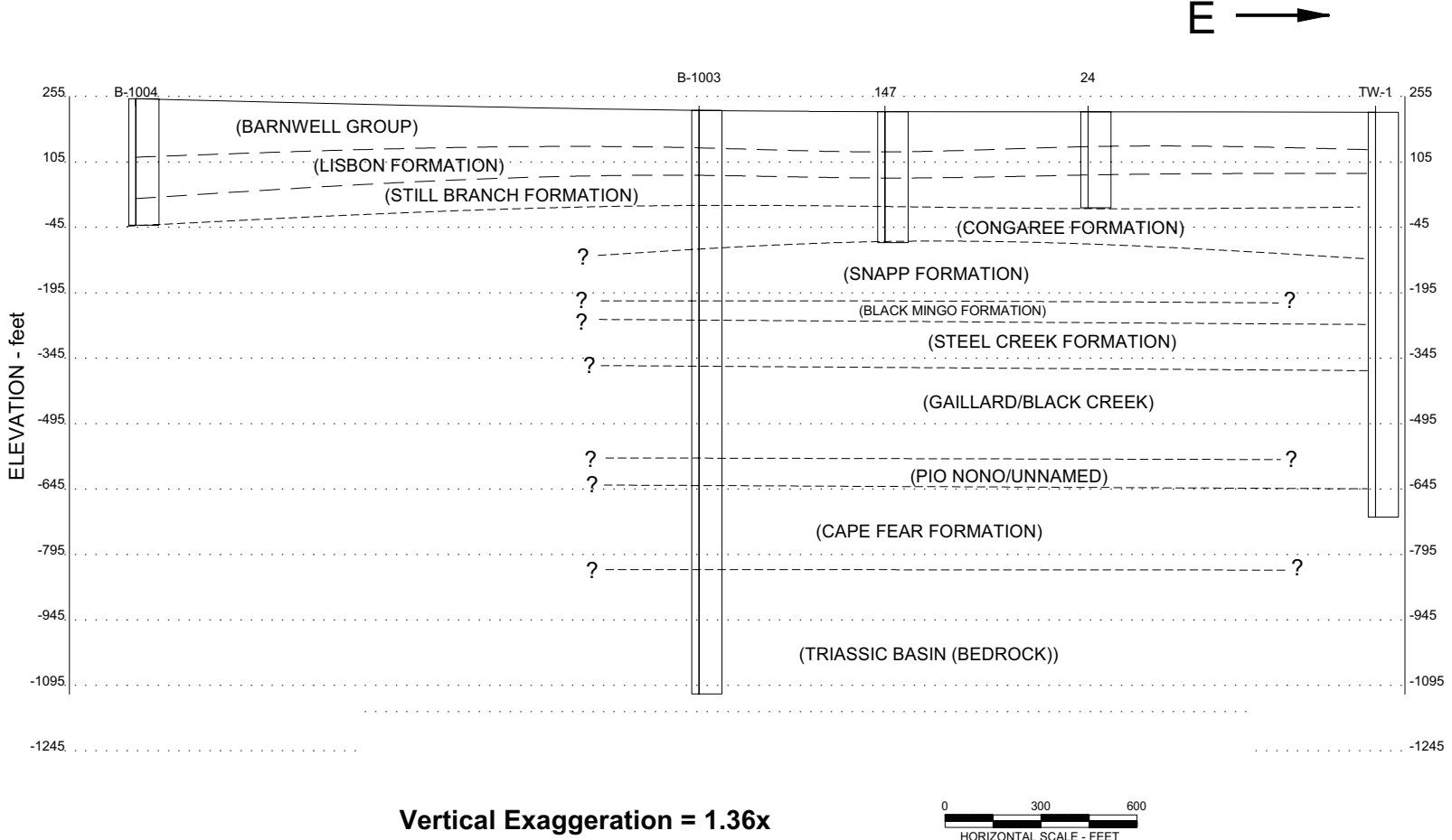
Figure 2.5.4-4 Subsurface Profile B-B'
