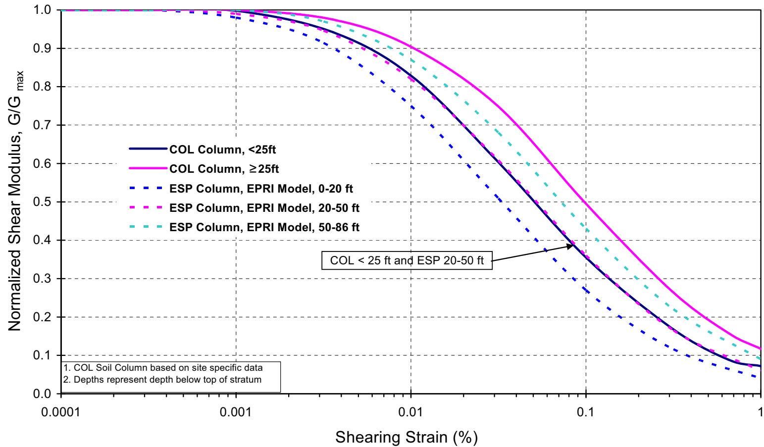
Figure 2.5.4-19a Comparison of Shear Modulus Reduction Curves - Backfill Soils
