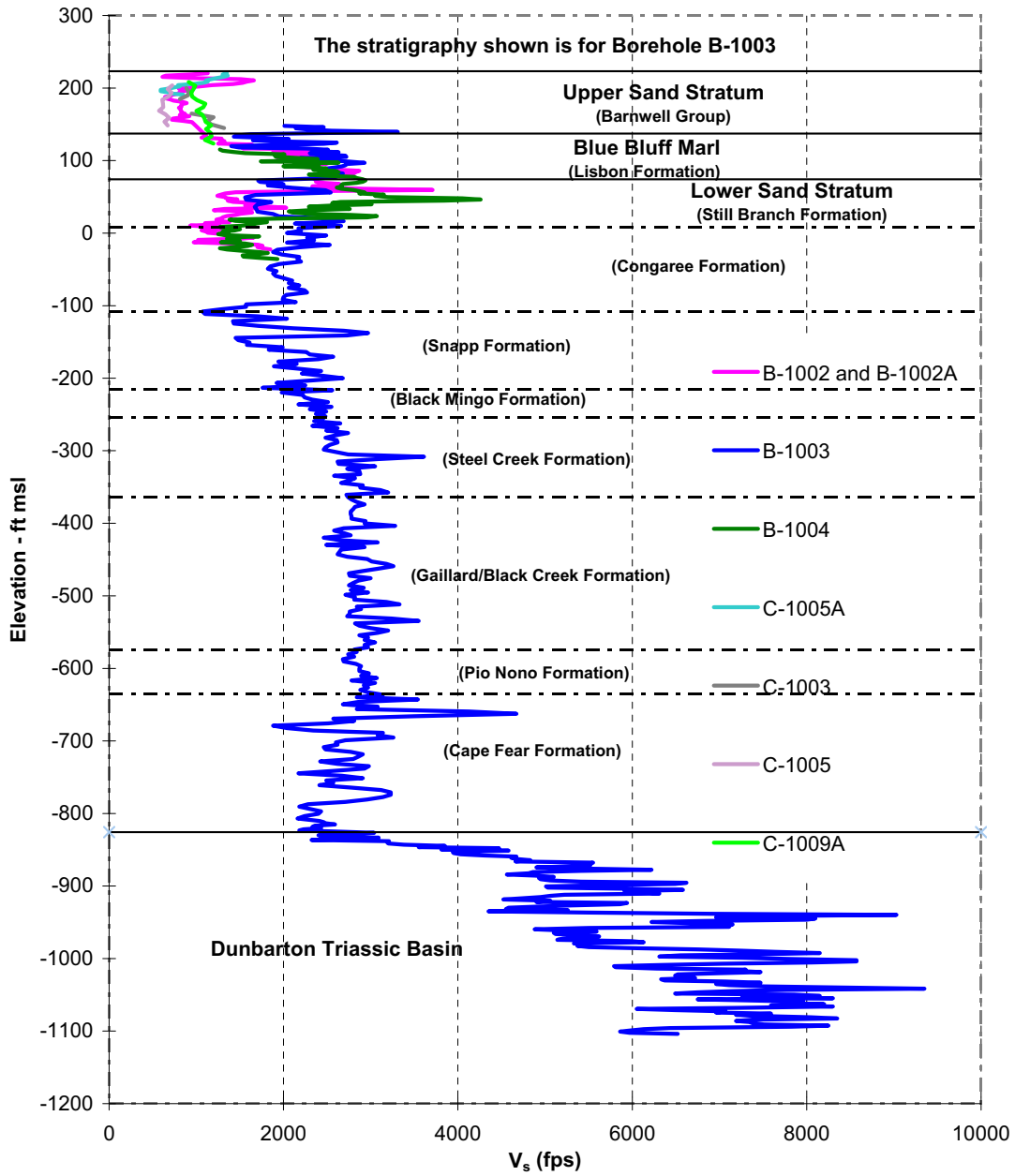
Figure 2.5.4-6 Shear Wave Velocity Measurements
