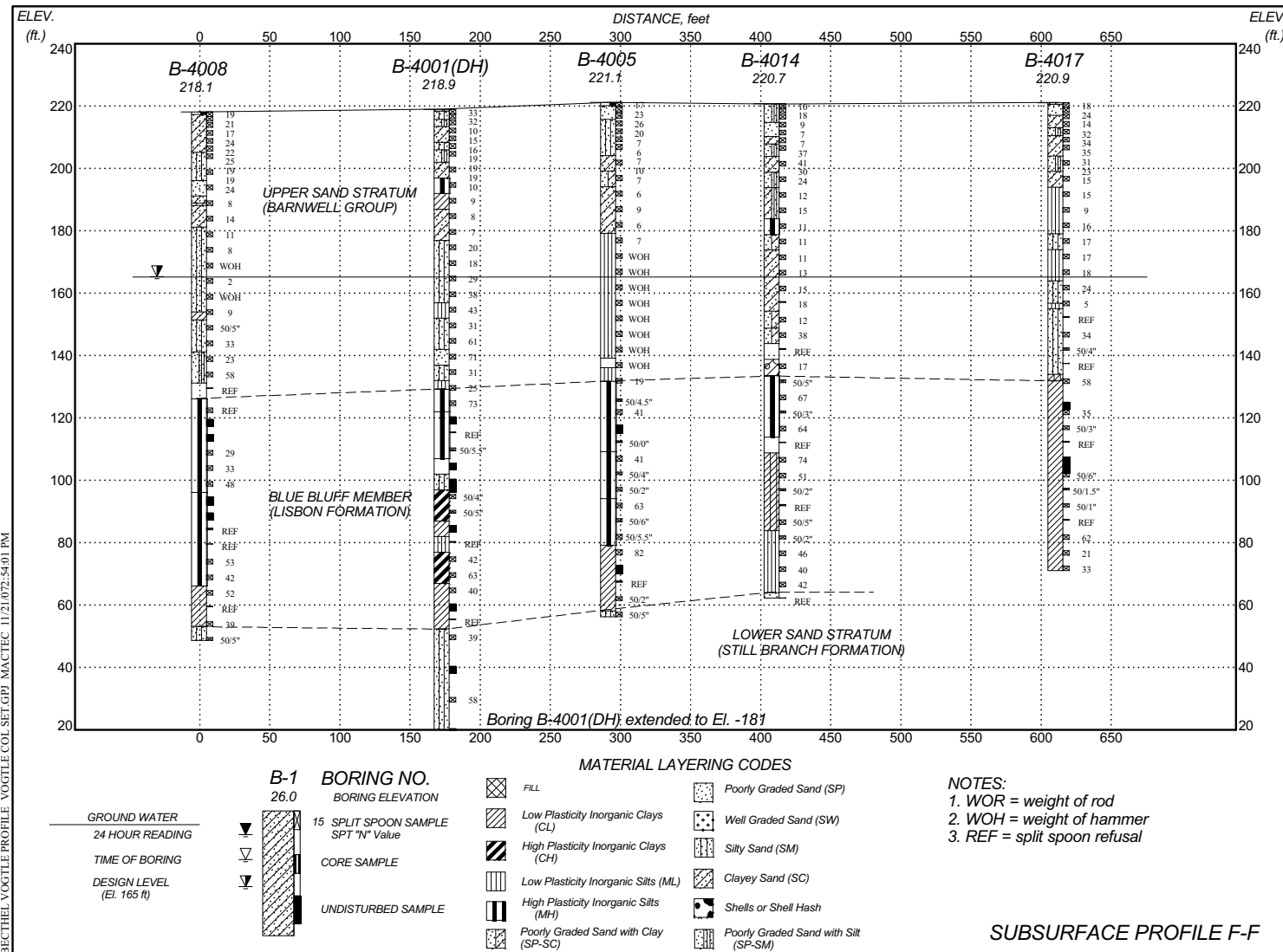
Figure 2.5.4-5b Subsurface Profile F-F'
