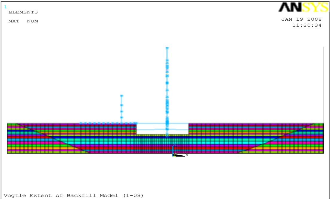
Figure A-1: 2D SASSI Backfill Model
