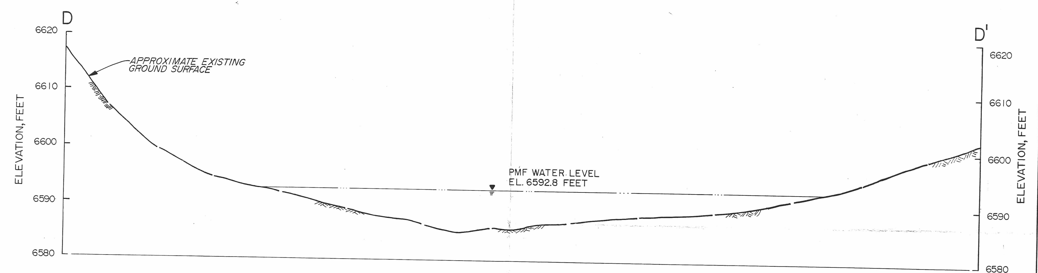
SECTION D-D'
