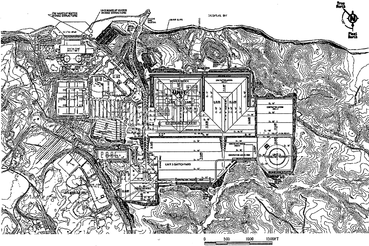
Figure 4.2-1—(Final Site Grading Plan CCNPP Unit 3)
