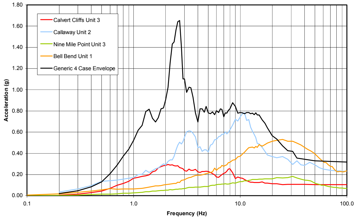
US EPR™ COL Site(s) Unbroadened Envelope In-Structure Response Spectra Center of NI Basemat, Site-Specific GMRS Input, X(E-W) Direction, 5% Damping
