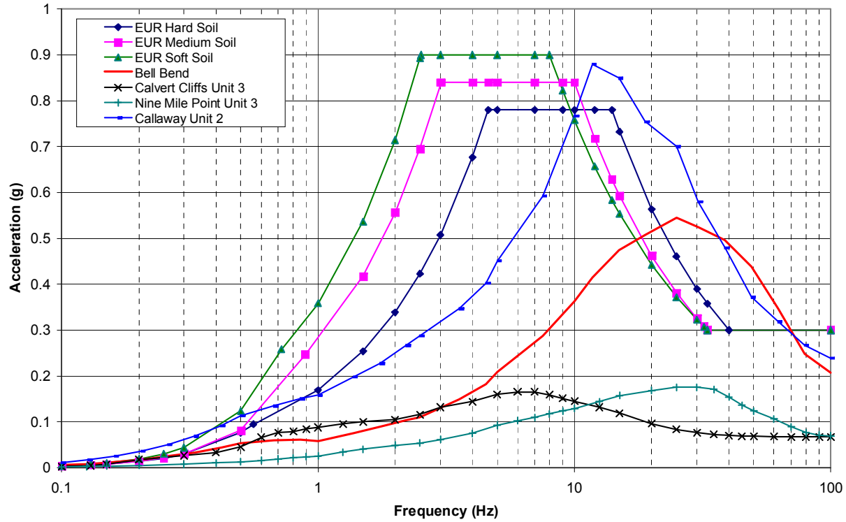
Comparison of EPR (Standard Plant) and COL Ground Design Spectra Horizontal Direction, 5% Damping
