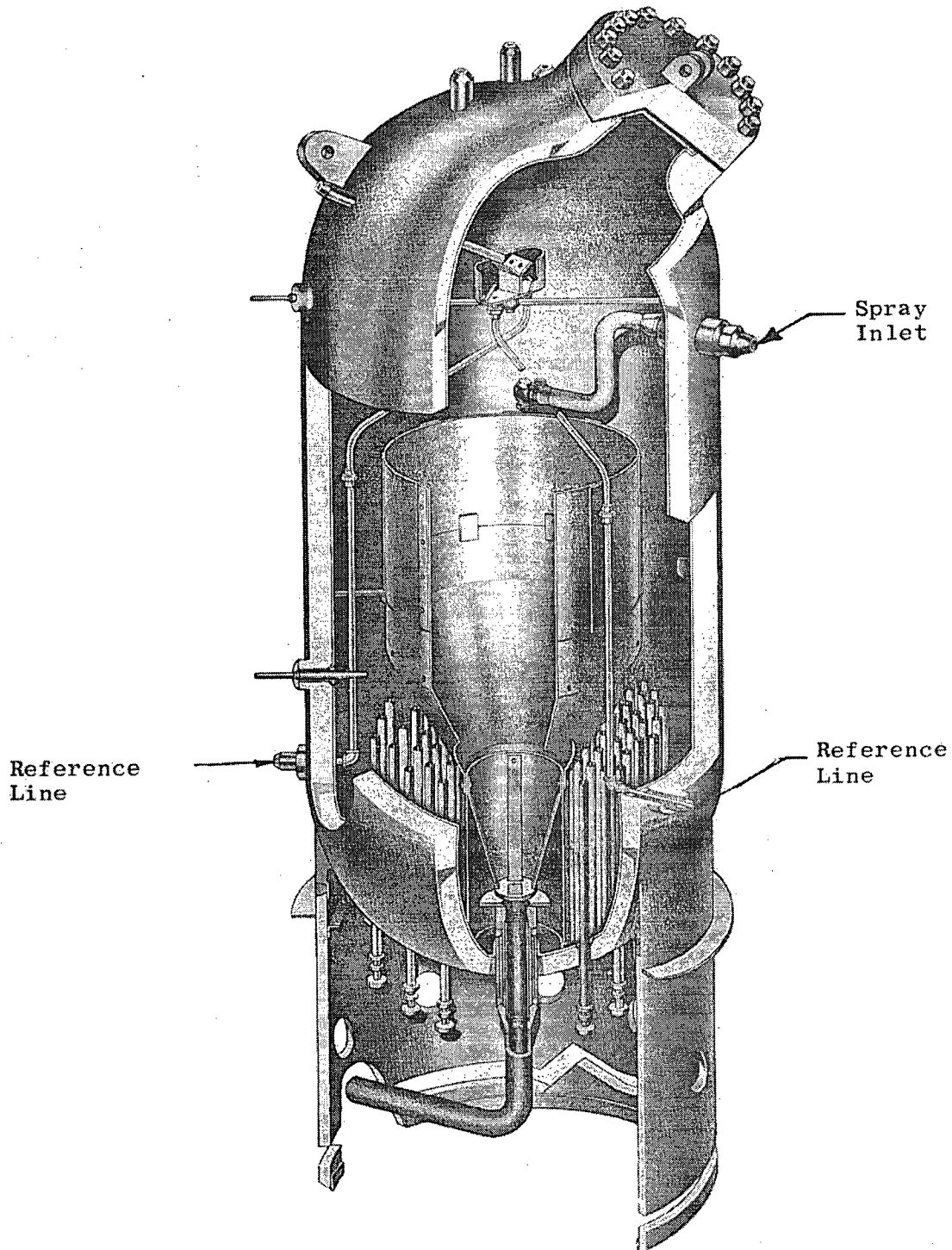
Figure 7-5 Pressurizer
