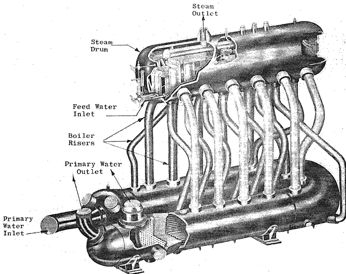
Figure 7-4 Steam Generator
