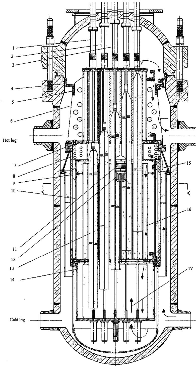
Figure 6-1 Reactor Internals
