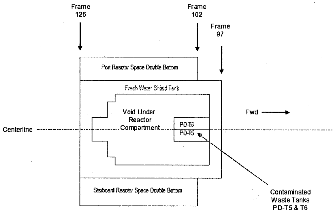
Figure 9-1 Double Bottom Tanks below RC
