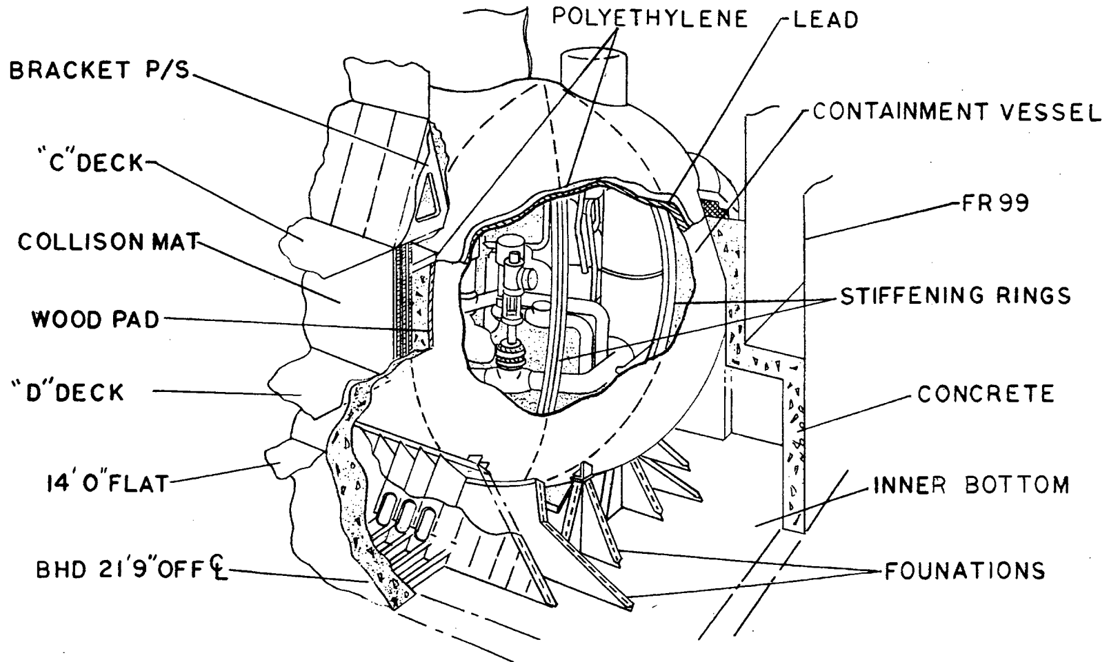
Figure 4-4 Containment Vessel (showing the secondary shield)
