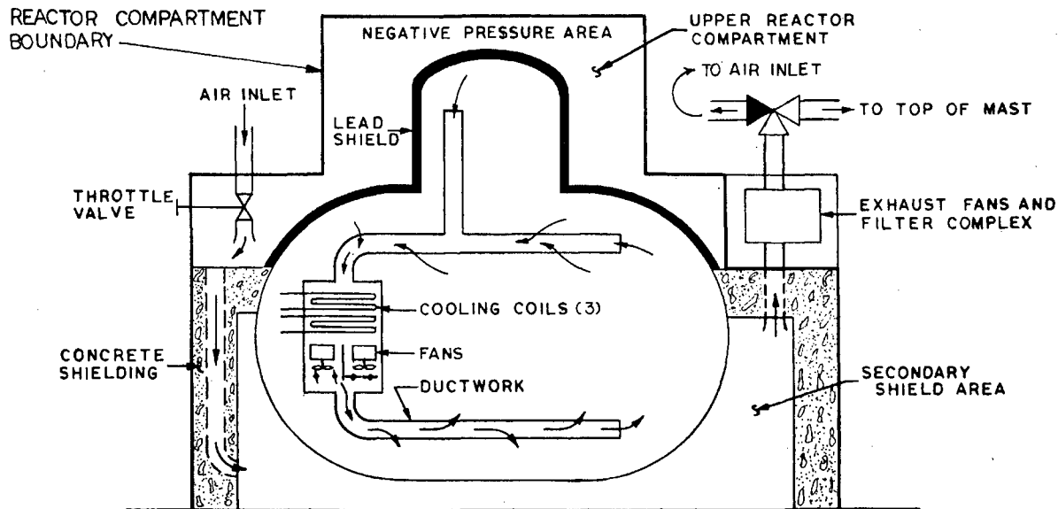
Figure 4-3 Reactor Compartment
