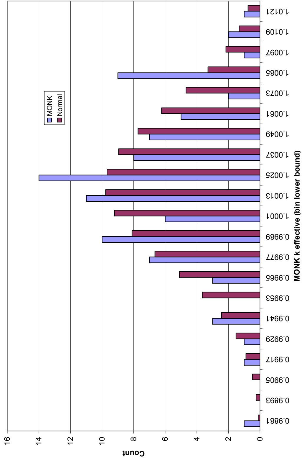
Figure 6-1: MONK8A k_{eff} Histogram
